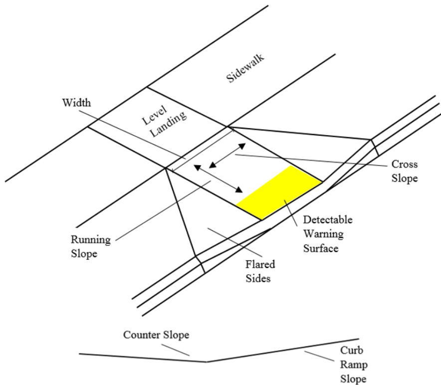
Figure 1. Diagram of Curb Ramp Elements Addressed in Federal Guidelines
