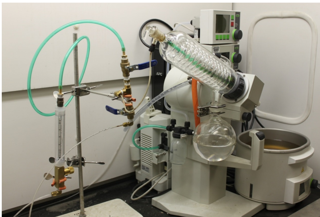
Figure 5 – Asphalt Binder Recovery Equipment at Rutgers University
