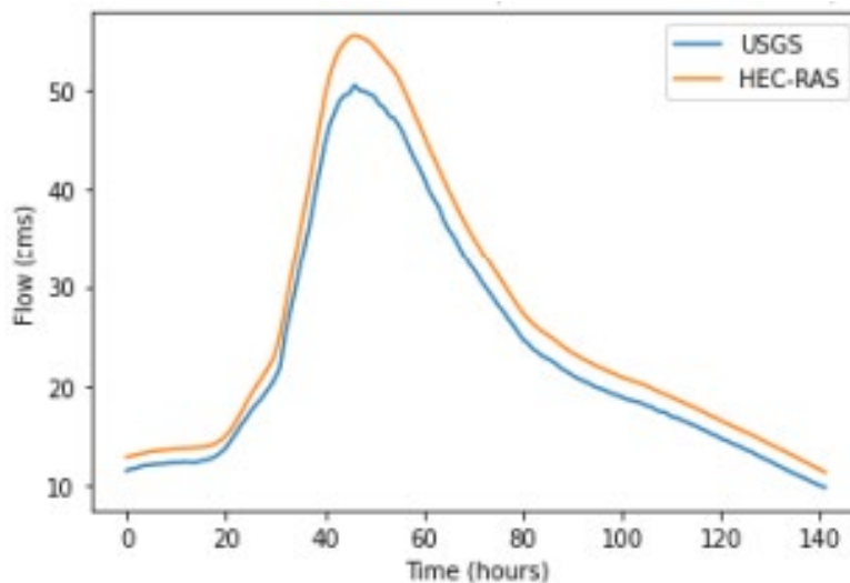
Fig. 7. Comparison of modeled (HEC-RAS) to estimated (USGS) hydrographs at the downstream model extent for the 11 April 2011 flood of 5-year recurrence interval recorded on Black Creek.
