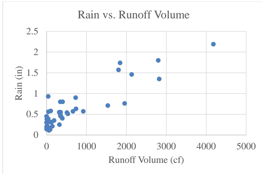
Figure 2: Rainfall-Outflow Data with Outliers Removed
