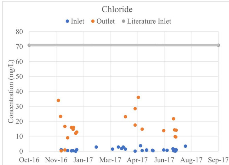
Figure 12: Inlet and Outlet Chloride Concentrations
