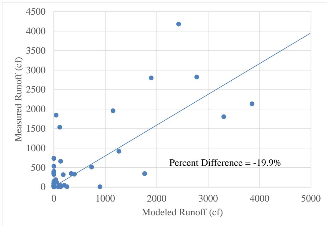
Figure 18: Measured vs. Calibrated Model Runoff Volume
