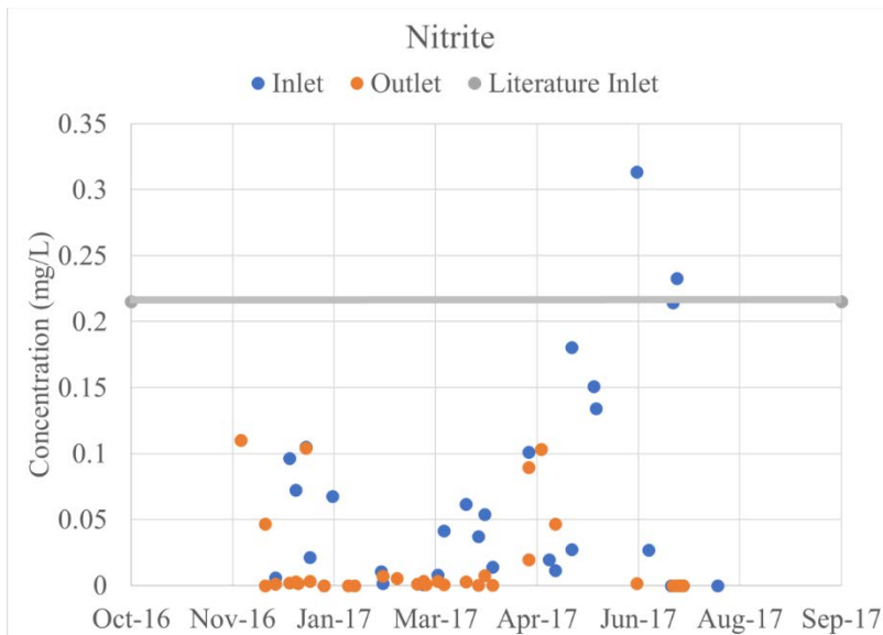
Figure 13: Inlet and Outlet Nitrite Concentrations
