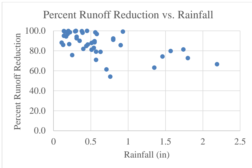
Figure 3: Percent Runoff Reduction
