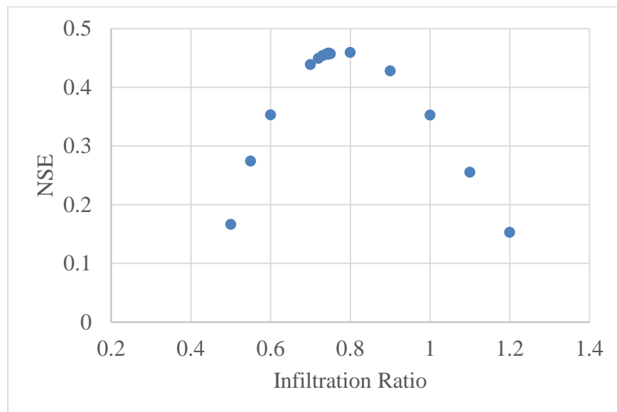
Figure 17: NSE vs. Infiltration Ratio
