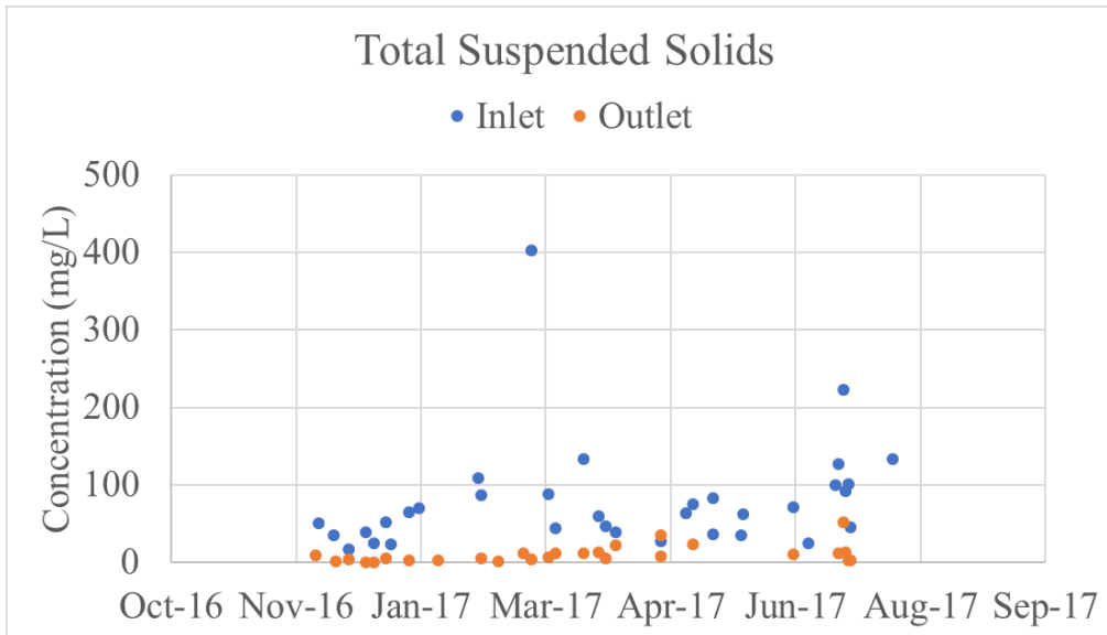
Figure 4: TSS Inlet and Outlet Concentrations
