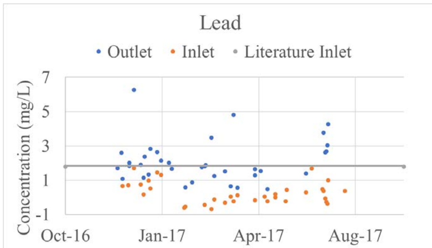
Figure 15: Lead Inlet and Outlet Concentrations
