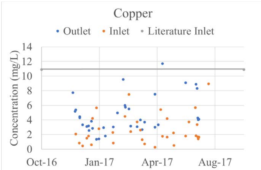
Figure 14: Copper Inlet and Outlet Concentrations
