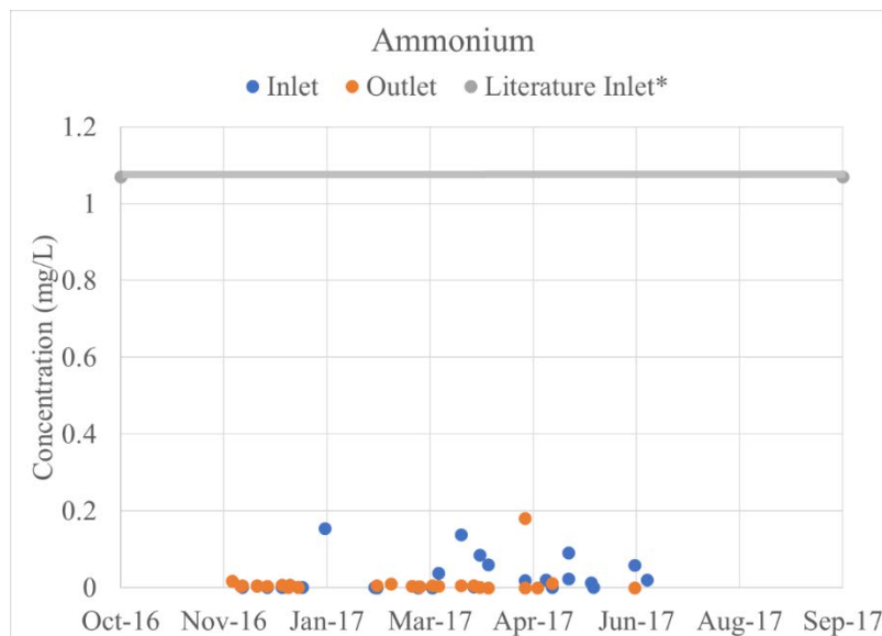
Figure 11: Inlet and Outlet Ammonium Concentrations
