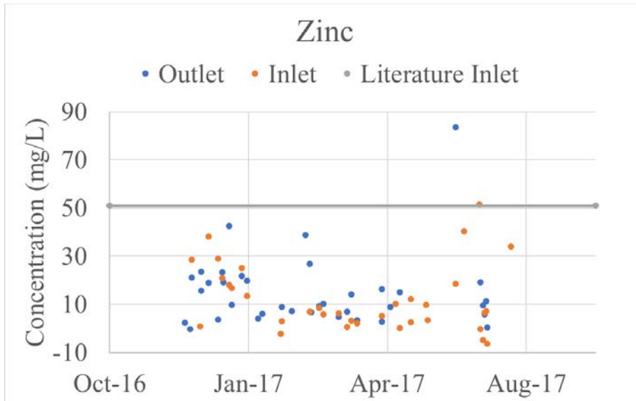
Figure 16: Zinc Inlet and Outlet Concentrations
