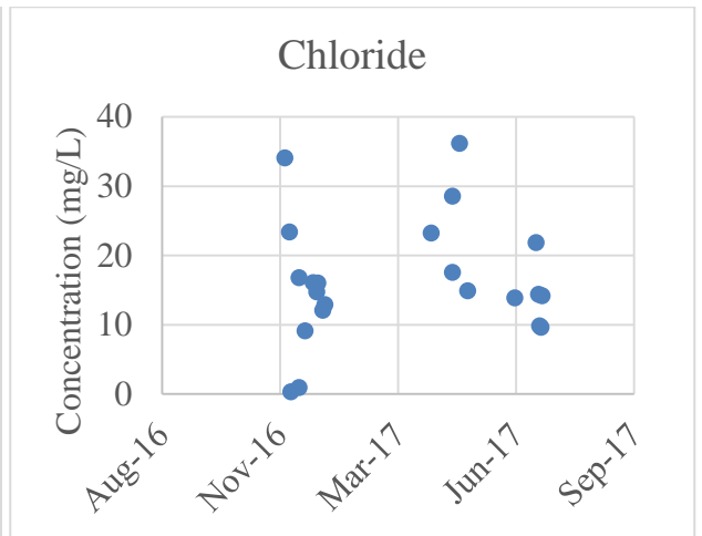
Figure 10: Chloride with Elevated Concentrations Removed
