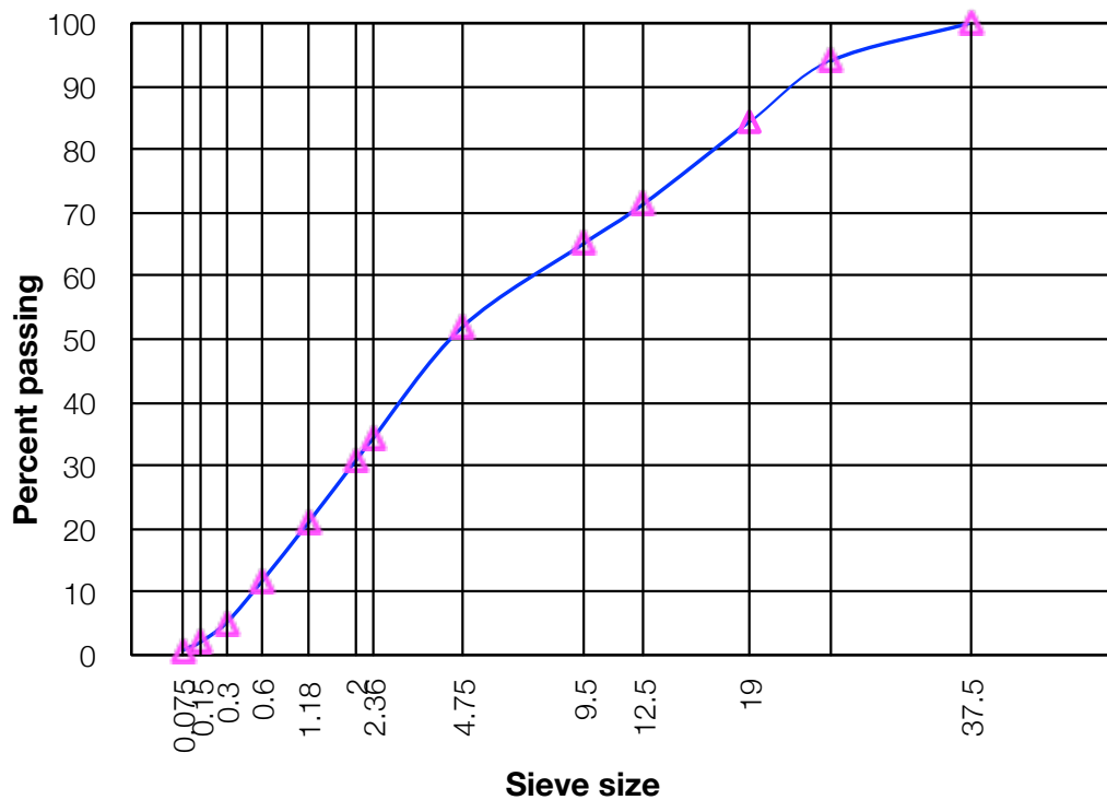
Figure 3.9: Gradation of Subgrade Soil Used in Test Pit
