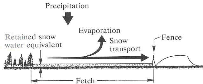
Figure 1. Diagram. The fetch concept used to estimate snow transport.
