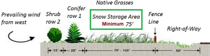
Figure 8. Diagram. Schematic design of a living snow fence. Source: Wyatt et al. 2012b
