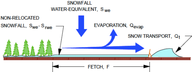
Figure 7. Diagram. Diagram of the fence concept used to estimate wind-transported snow. Source: Tabler, 2003
