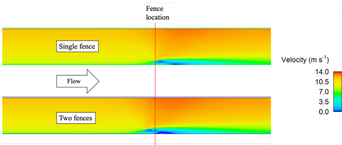
Figure 27. Diagram. Contours of velocity magnitude around a single fence and two fences separated by a distance of 3H . The red line shows the location of the second fence.
