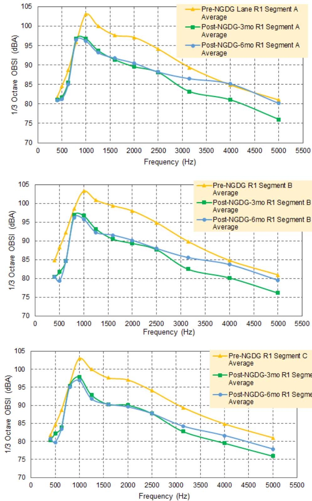
Figure 5. 2 Comparative Plots of 1/3 Octave Band Intensity Levels, Lane R1
