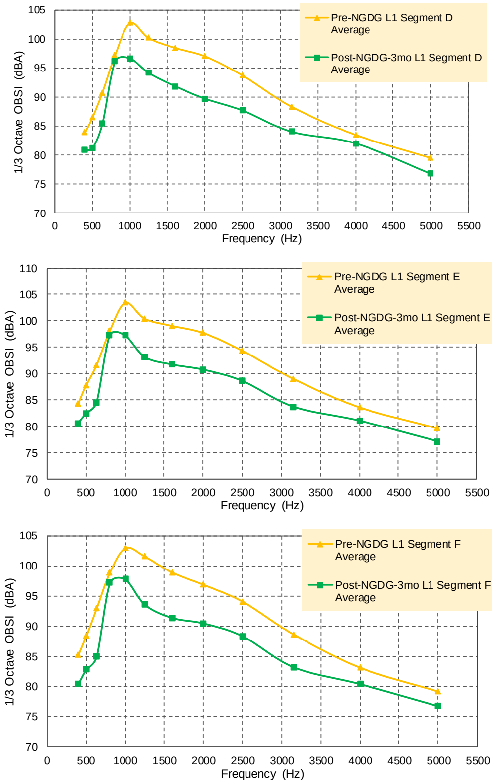
Figure 5. 4 Comparative Plots of 1/3 Octave Band Intensity Levels, Lane L1
