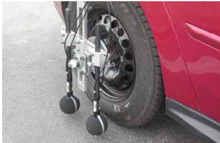
Figure 3. 1 TxDOT's Dual-Probe On-Board Sound Intensity
