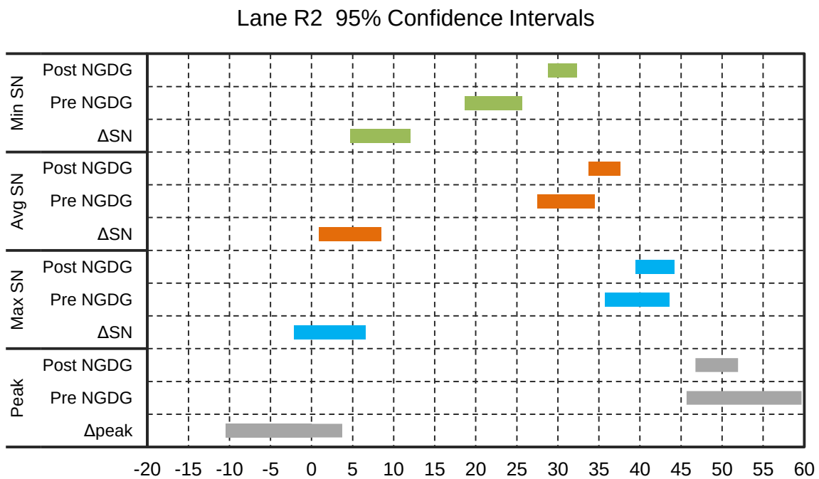
Figure 4. 5 Northbound Loop 610: 95% Confidence Intervals
