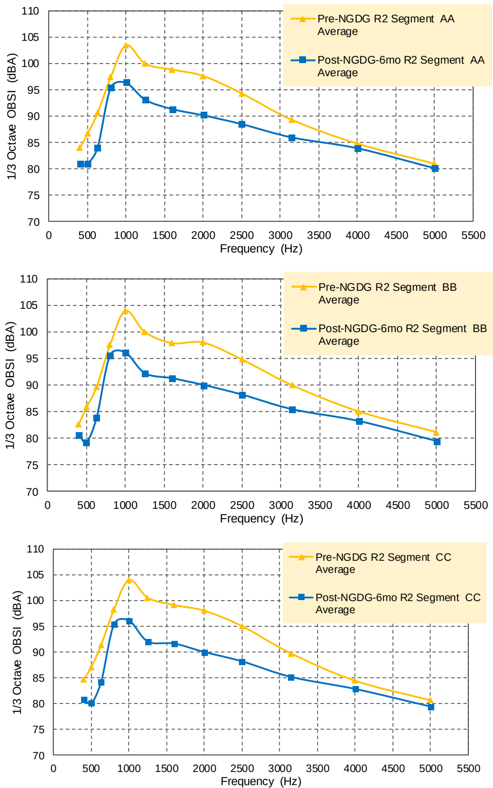
Figure 5. 3 Comparative Plots of 1/3 Octave Band Intensity Levels, Lane R2
