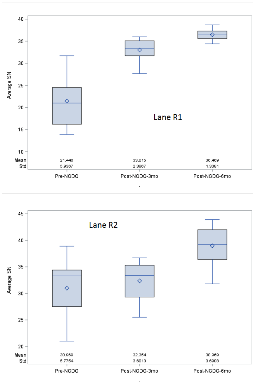
Figure 4. 3 Boxplots of Average SNs — Loop 610 Northbound
