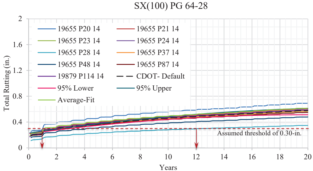
Figure 123. Total Rutting Due to AADTT = 800 by SX(100) PG 64-28 Mix
