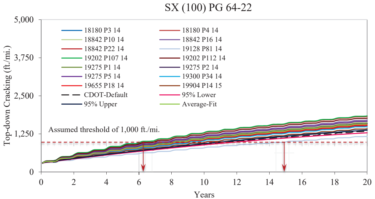
Figure 119. Longitudinal Cracking Due to AADTT = 800 by SX(100) PG 64-22 Mix
