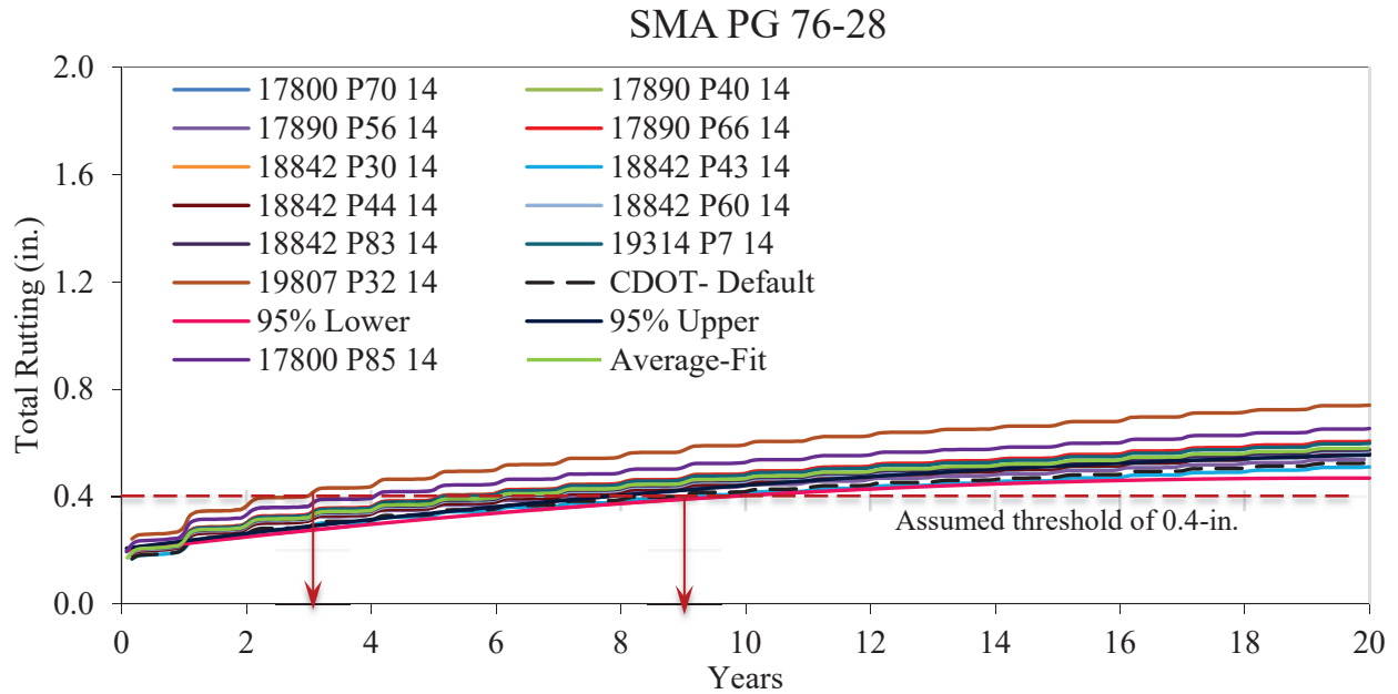
Figure 53. Total Rutting Due to AADTT = 800 by SMA PG 76-28 Mix
