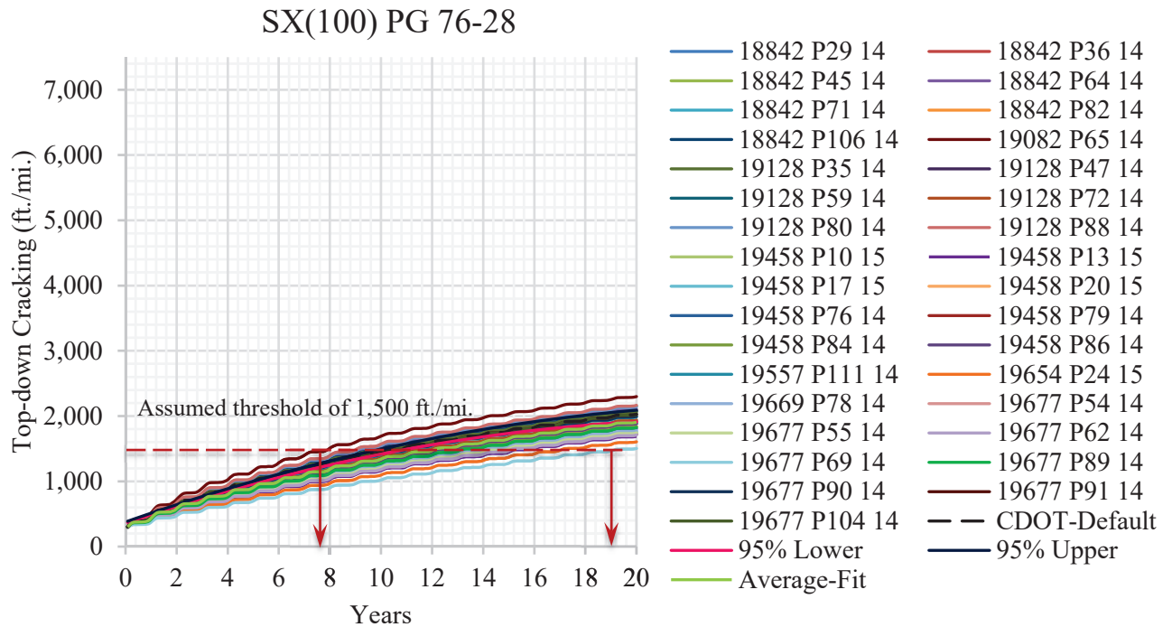
Figure 139. Longitudinal Cracking Due to AADTT = 800 by SX(100) PG 76-28 Mix
