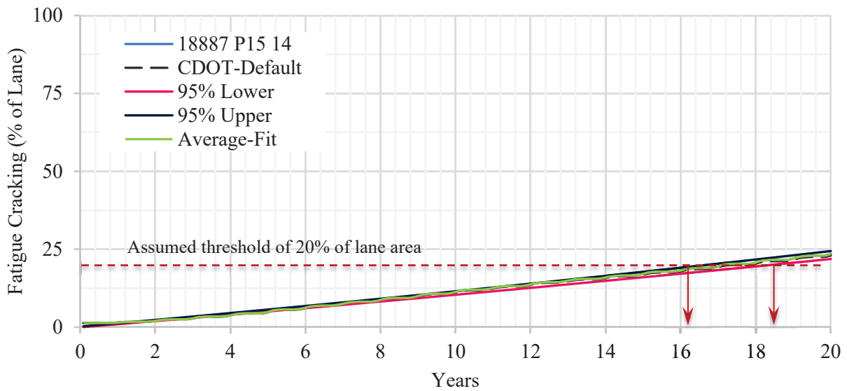
Figure 107. Bottom-up Fatigue Cracking Due to AADTT = 800 by SX(100) PG 58-28 Mix
