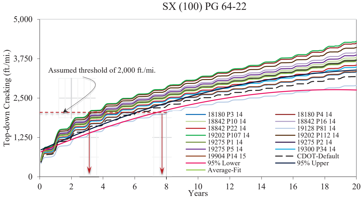
Figure 118. Longitudinal Cracking Due to AADTT = 7,000 by SX(100) PG 64-22 Mix
