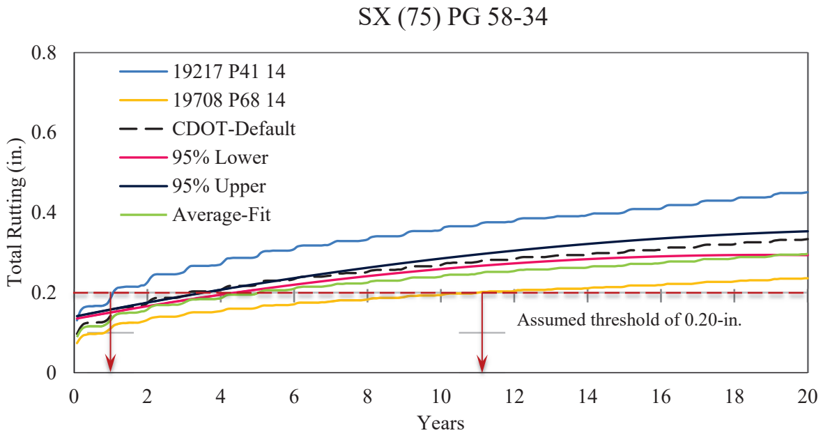
Figure 73. Total Rutting Due to AADTT = 800 by SX(75) PG 58-34 Mix
