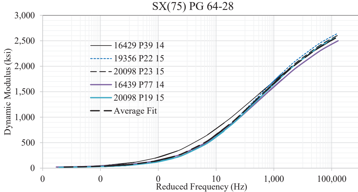
Figure 10. Dynamic Modulus of SX(75) PG 64-28 Mix
