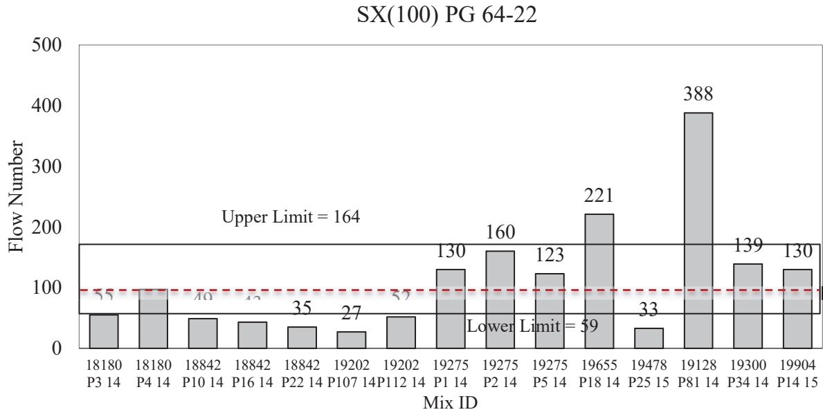
Figure 25. Flow Numbers for SX(100) PG 64-22 Mix
