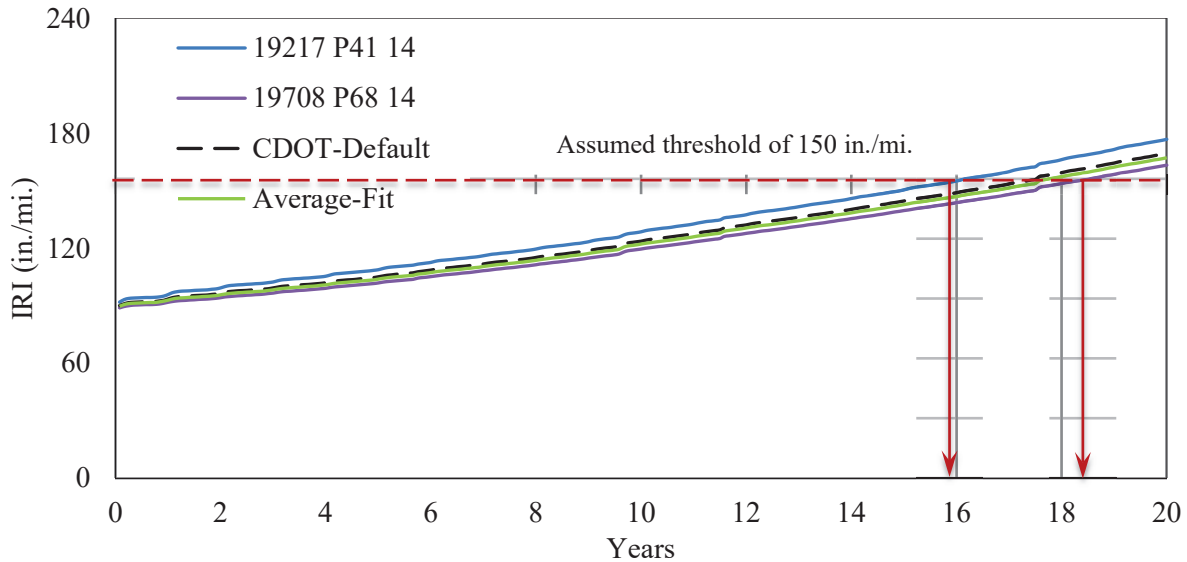
Figure 71. IRI Due to AADTT = 800 by SX(75) PG 58-34 Mix
