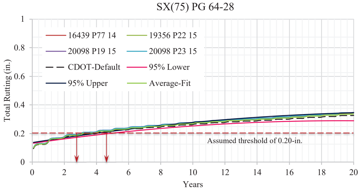
Figure 93. Total Rutting Due to AADTT = 800 by SX(75) PG 64-28 Mix
