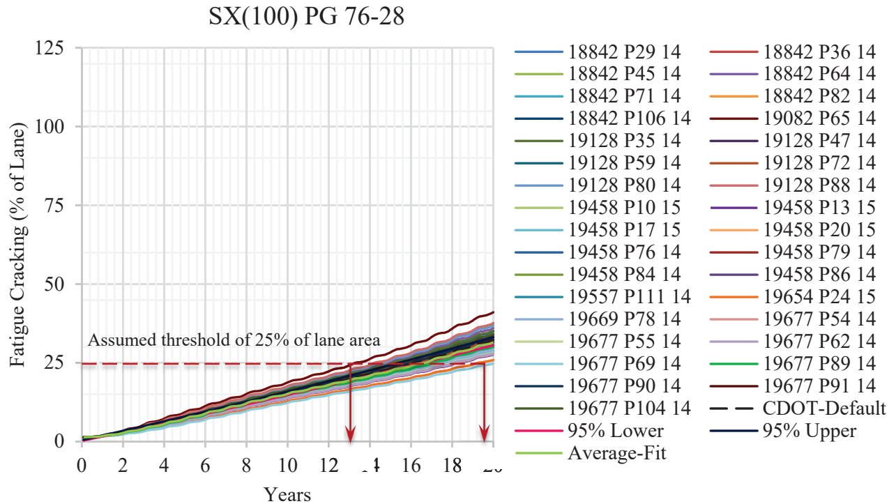
Figure 137. Bottom-up Fatigue Cracking Due to AADTT = 800 by SX(100) PG 76-28 Mix
