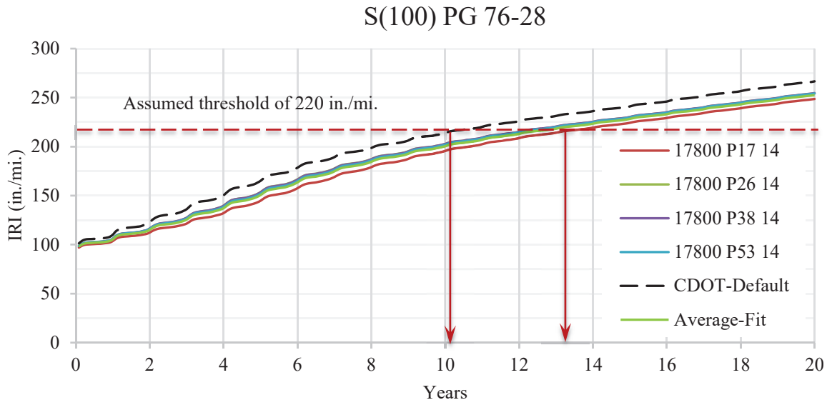
Figure 40. IRI Due to AADTT = 7,000 by S(100) PG 76-28 Mix
