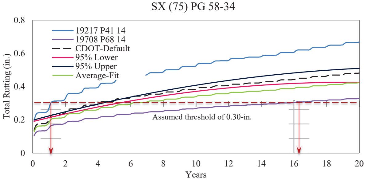
Figure 72. Total Rutting Due to AADTT = 3,000 by SX(75) PG 58-34 Mix
