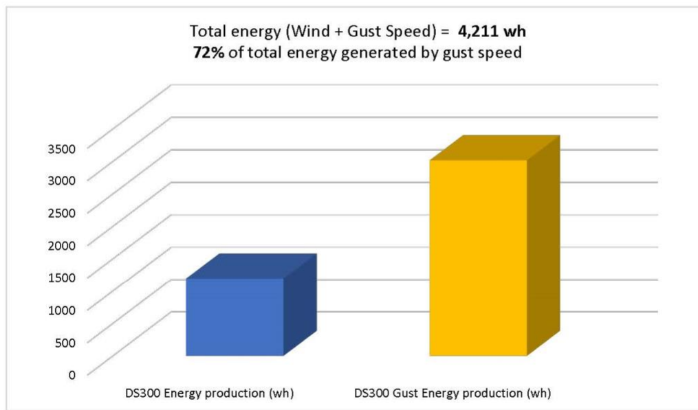
Figure 12. Avg. Speed and Gust Data, I-95 Site, 25 May - 22 June, 2019 Wired Anemometer (Wolf 2), w/ DS300 Turbine Outputs
