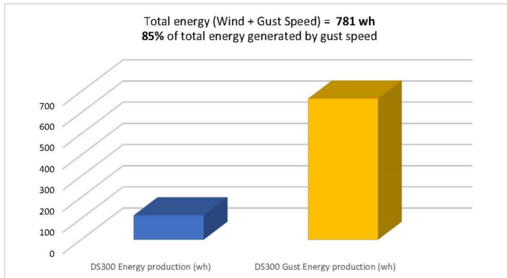
Figure 14. Avg. Speed and Gust Data, US-1 Site, 25 May - 25 June, 2019 Wireless Anemometer (Baby Wolf 2), w/ DS300 Turbine Outputs
