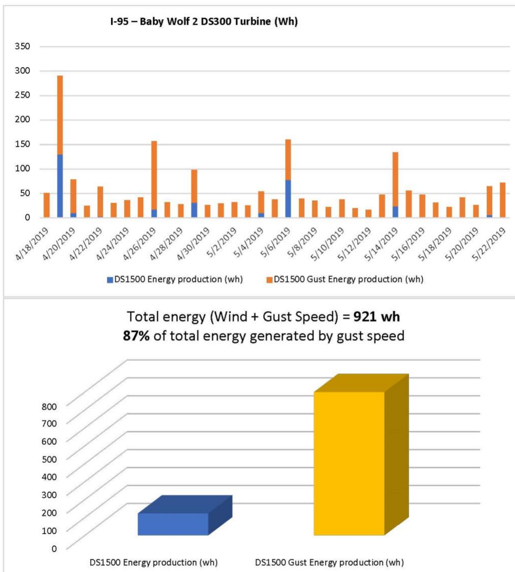
Figure 6. Avg. Speed and Gust Data, I-95 Site, 18 April – 22 May, 2019 Wired Anemometer (Wolf 2), w/ DS300 Turbine Outputs
