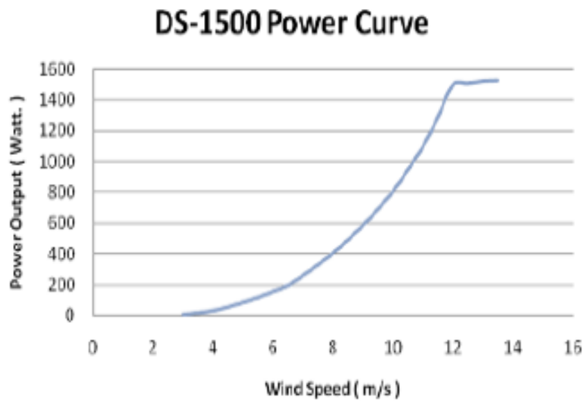
Figure 5-2 Colite DS-1500 vertical axis wind turbine wind speed power curve
