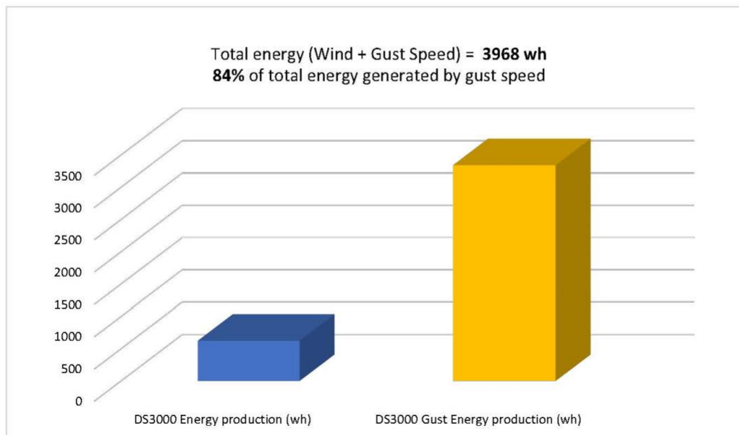
Figure 17. Avg. Speed and Gust Data, I-95 Site, 18 April - 22 May, 2019 Wireless Anemometer (Baby Wolf 2), w/ DS300 Turbine Outputs
