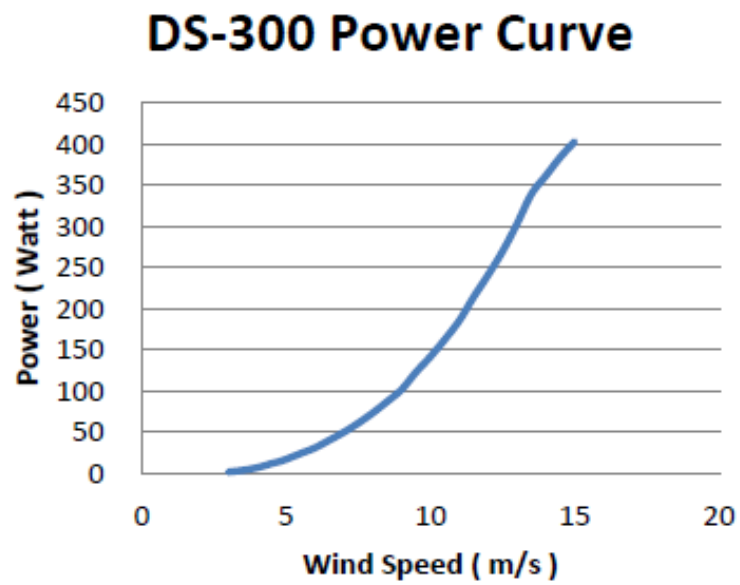
Figure 5-1 Colite DS-300 vertical axis wind turbine wind speed power curve
