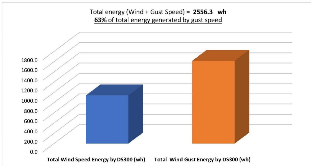
Figure 19. Avg. Speed and Gust Data, I-40/85 Site, 25 May - 18 June, 2019 Wireless Anemometer (Baby Wolf 1), w/ DS300 Turbine Outputs
