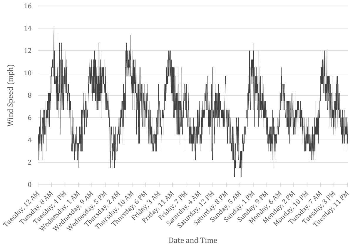
Figure 6-3 Sample wind speed data at Guilford County Site (post WGA) showing the diurnal wind pattern
