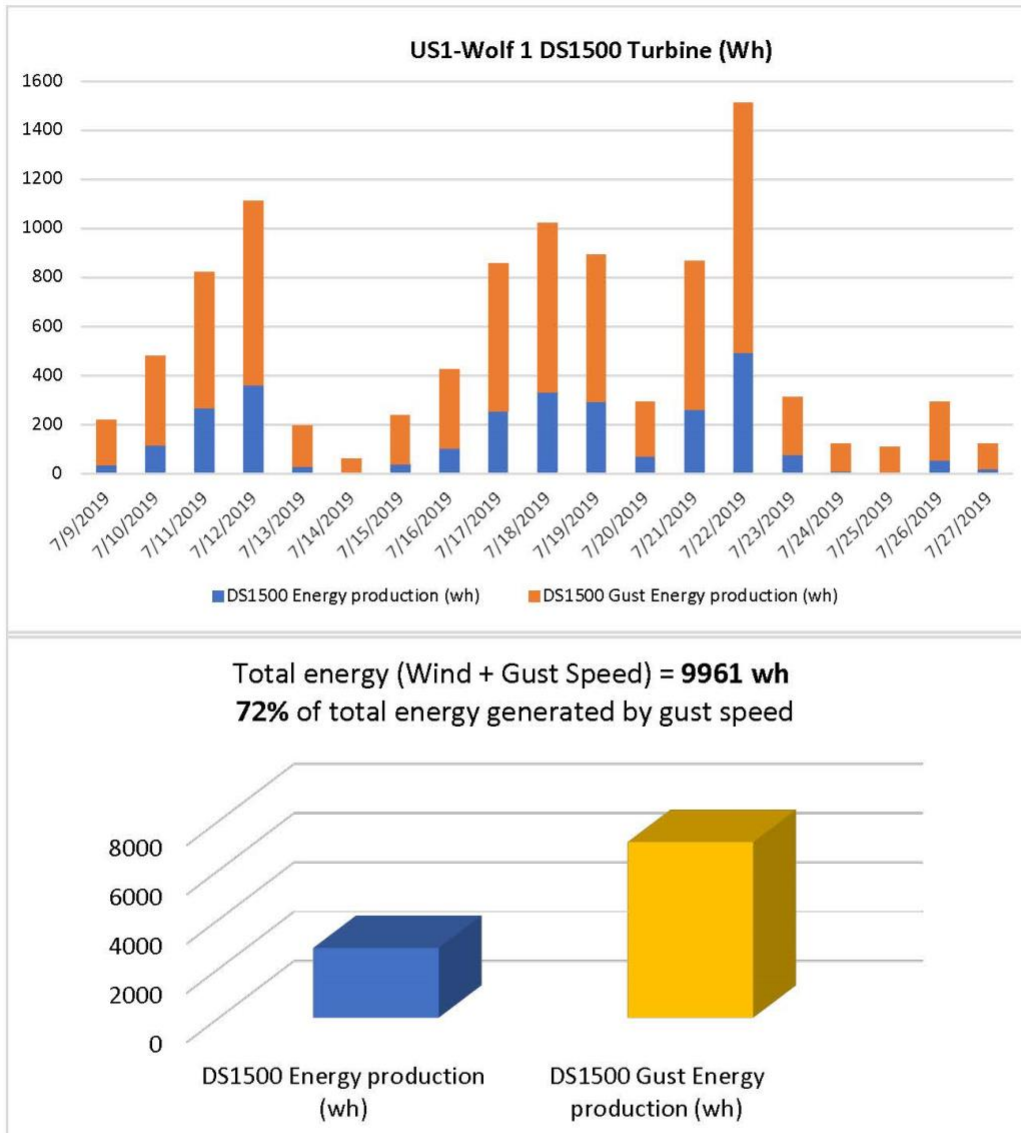
Figure 1. Avg. Speed and Gust Data, US 1/ 64 Site, 9 – 27 July, 2019 Wired Anemometer (Wolf 1), w/ DS1500 Turbine Outputs
