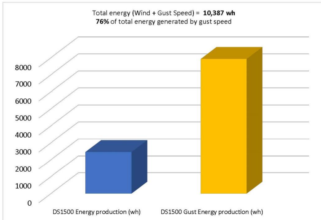
Figure 3. Avg. Speed and Gust Data, I-40/85 Site, 25 May – 25 June, 2019 Wireless Anemometer (Baby Wolf 2), w/ DS1500 Turbine Outputs
