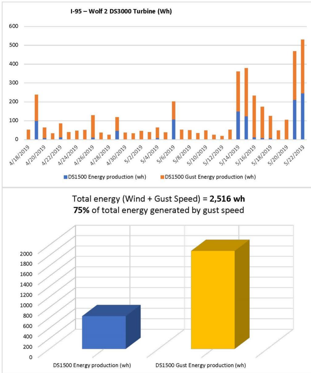
Figure 5. Avg. Speed and Gust Data, I-95 Site, 18 April – 22 May, 2019 Wired Anemometer (Wolf 2), w/ DS3000 Turbine Outputs
