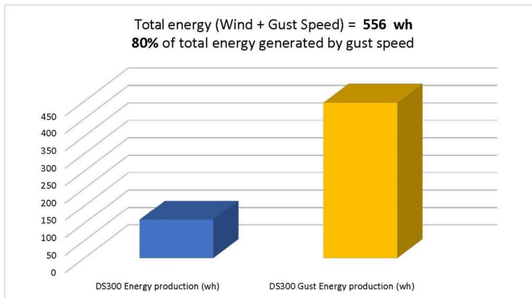
Figure 18. Avg. Speed and Gust Data, I-95 Site, 18 April - 22 May, 2019 Wireless Anemometer (Baby Wolf 2), w/ DS300 Turbine Outputs
