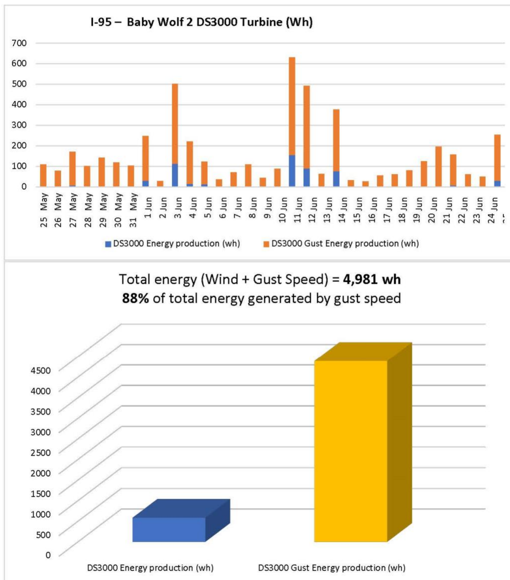
Figure 13. Avg. Speed and Gust Data, I-95 Site, 25 May - 25 June, 2019 Wireless Anemometer (Baby Wolf 2), w/ DS3000 Turbine Outputs
