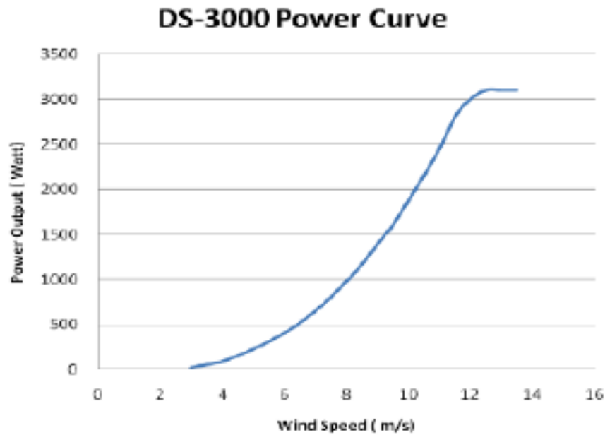
Figure 5-3 Colite DS-3000 vertical axis wind turbine wind speed power curve
