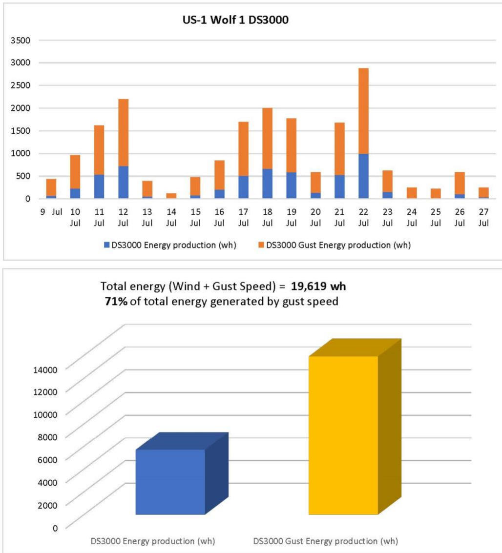
Figure 7. Avg. Speed and Gust Data, US-1 Site, 9 - 27 July, 2019 Wired Anemometer (Wolf 1), w/ DS3000 Turbine Outputs
