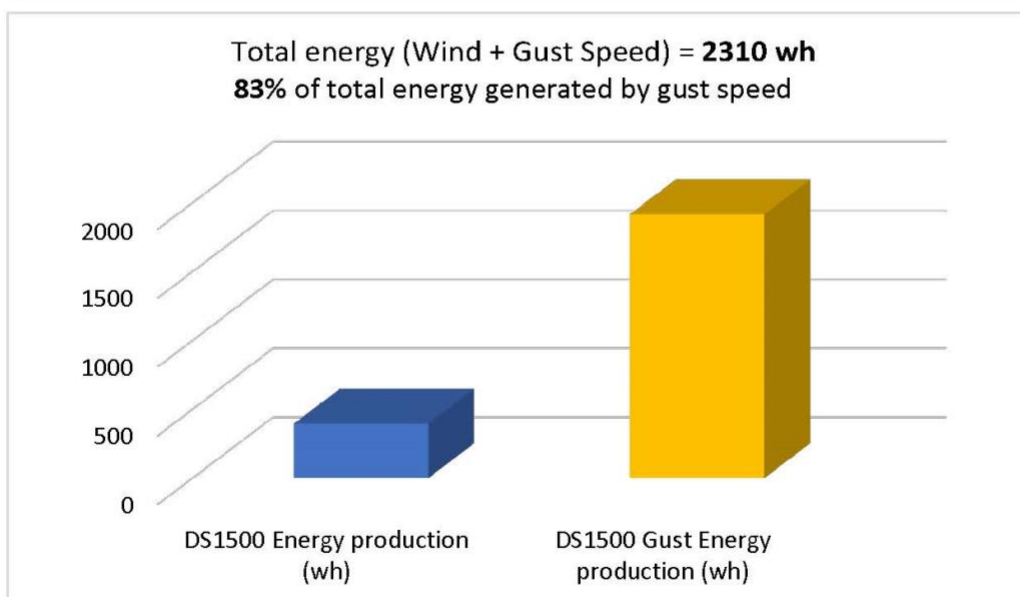
Figure 2. Avg. Speed and Gust Data, US 1/ 64 Site, 9 – 27 July, 2019 Wireless Anemometer ( Baby Wolf 1), w/ DS1500 Turbine Outputs
