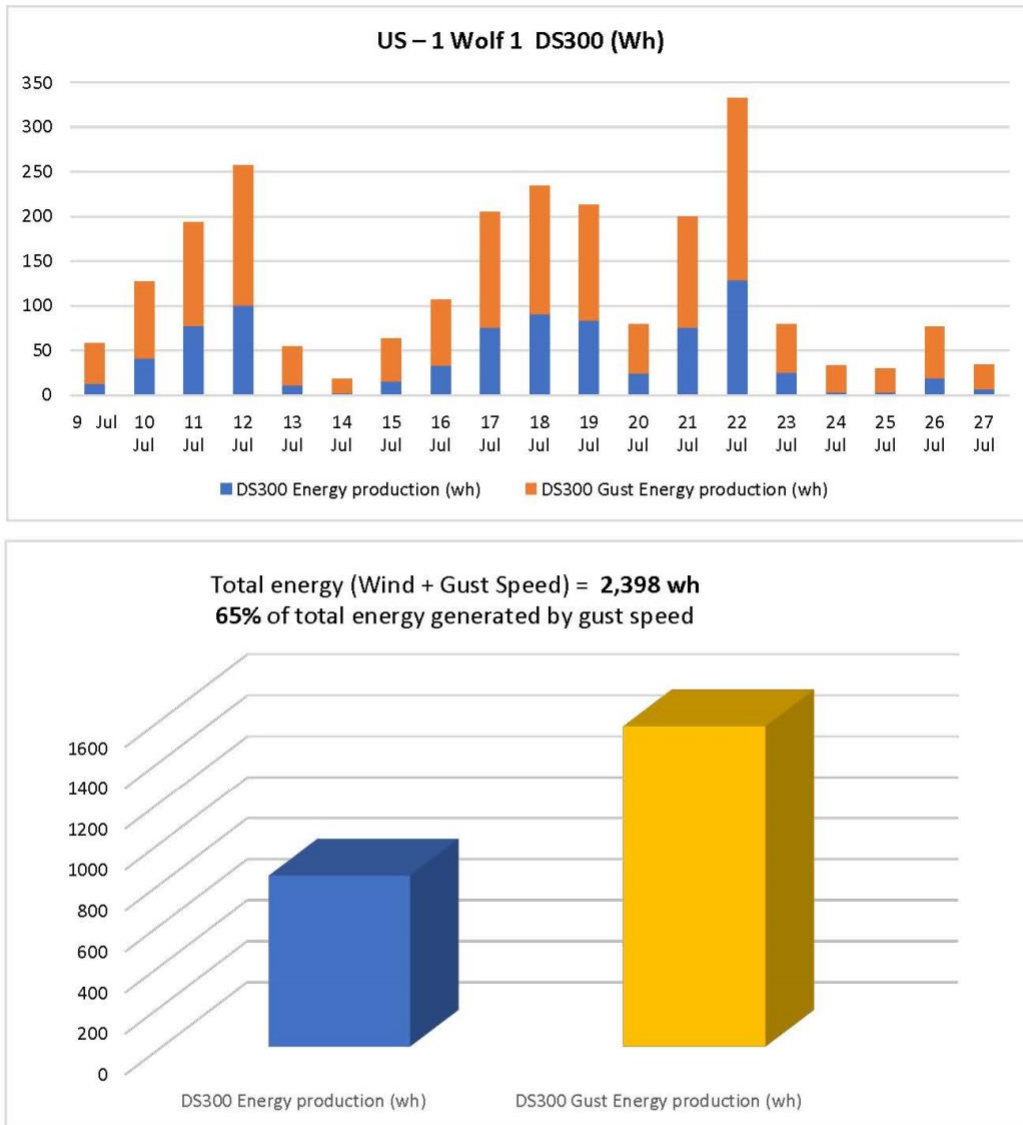
Figure 8. Avg. Speed and Gust Data, US-1 Site, 9 - 27 July, 2019 Wired Anemometer (Wolf 1), w/ DS300 Turbine Outputs
