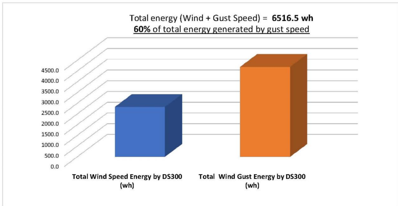
Figure 20. Avg. Speed and Gust Data, I-40/85 Site, 25 May - 18 June, 2019 Wired Anemometer (Wolf 1), w/ DS300 Turbine Outputs
