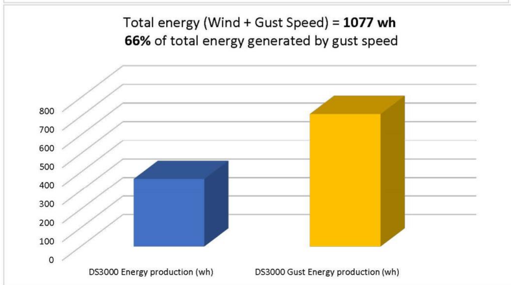
Figure 16. Avg. Speed and Gust Data, I-95 Site, 18 April - 22 May, 2019 Wired Anemometer (Wolf 2), w/ DS300 Turbine Outputs
