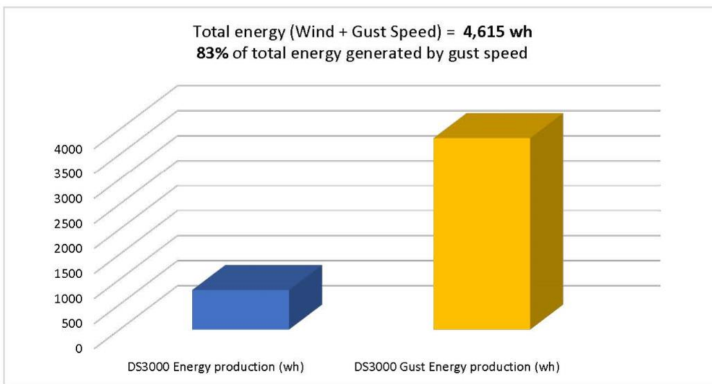
Figure 9. Avg. Speed and Gust Data, US-1 Site, 9 - 27 July, 2019 Wired Anemometer (Wolf 1), w/ DS3000 Turbine Outputs
