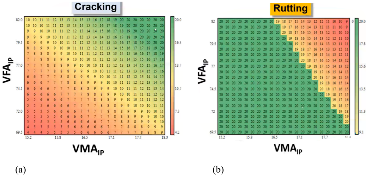
Figure 2.2. PEMD-predictive results (in years) for: (a) cracking, and (b) rutting.
