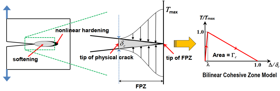
Figure 4.1 Schematic illustration of FPZ of typical quasi-brittle materials.
