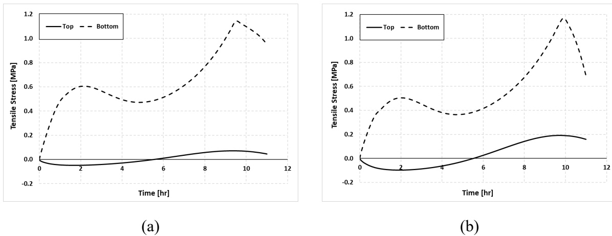
Figure 4.16. Horizontal stresses at top and bottom of overlay in case V, using a) good-quality, and b) poor-quality material.
