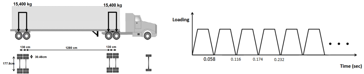
Figure 4.10. Mechanical load configuration.
