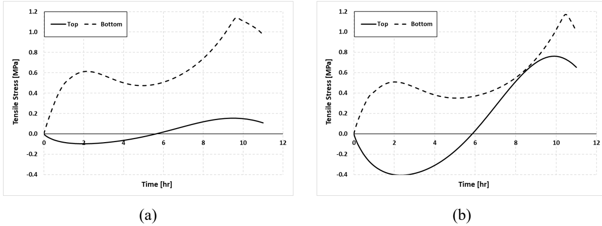
Figure 4.15. Horizontal stresses at top and bottom of overlay in case IV, using a) good-quality, and b) poor-quality material.
