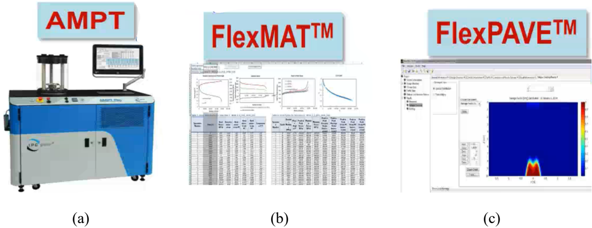
Figure 2.1. FlexPAVE system tools for: a) material testing, b) material analysis, and c) pavement analysis.
