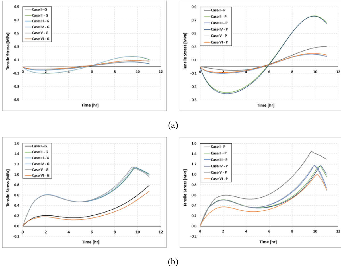
Figure 4.18. Thermal cracking behavior of pavements with different overlay configuration, a) top of the overlay, and b) bottom of the overlay.
