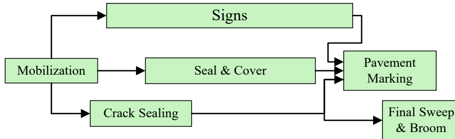
Figure 3 The sequence logic diagram for seal & cover projects
