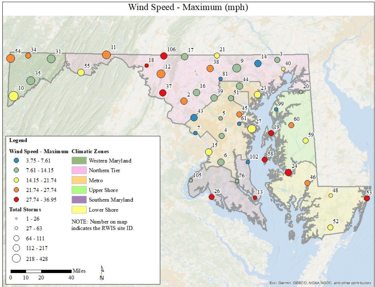
Figure 94. Shows the maximum wind speed in miles per hours (mph) for each storm event at each RWIS location in Maryland form 2012-2019.
