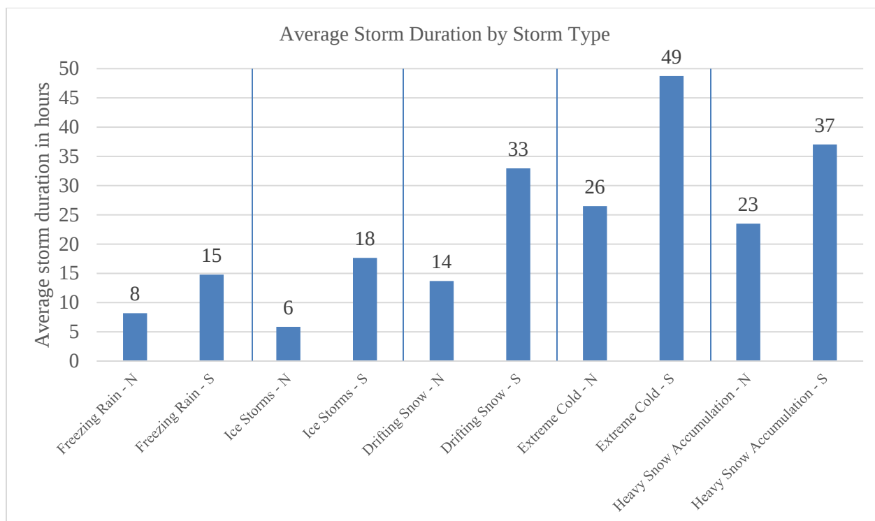
Figure 52. Average Duration of Various Storm Types (N – Normal Duration, S – Severe Duration)
