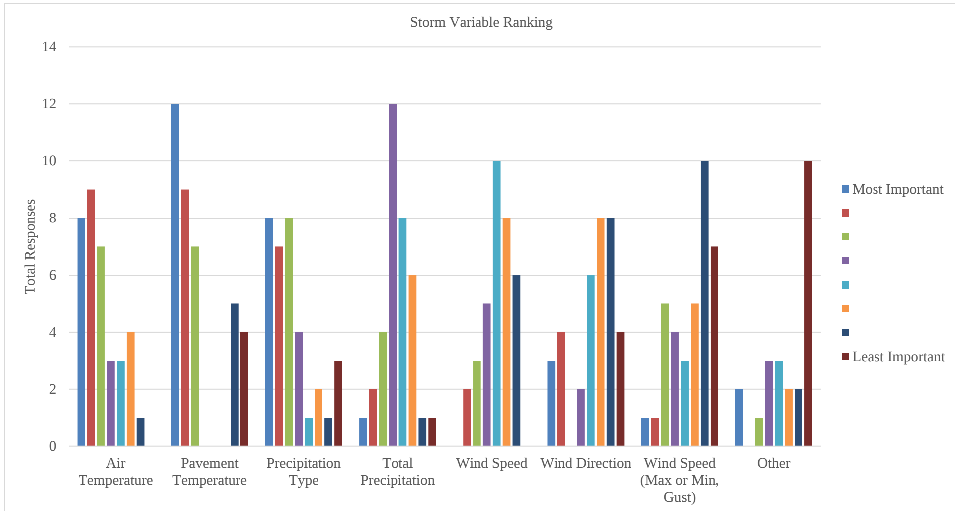
Figure 26. Storm Variable Ranking
