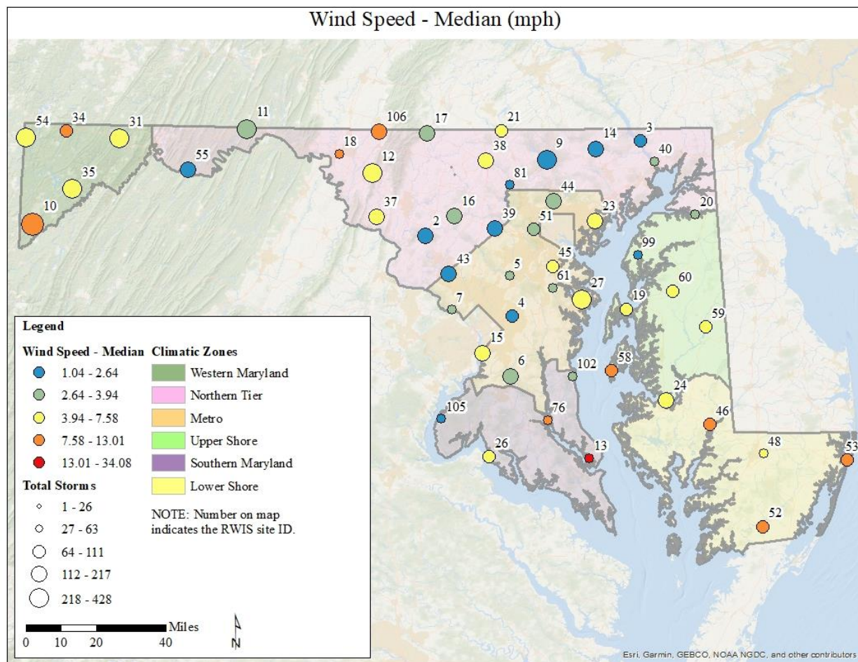
Figure 92. Shows the median wind speed in miles per hours (mph) for each storm event at each RWIS location in Maryland form 2012-2019.
