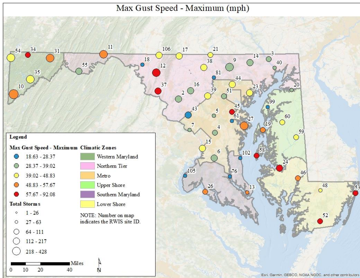
Figure 90. Shows the maximum wind gust speed in miles per hours (mph) for each storm event at each RWIS location in Maryland form 2012-2019.
