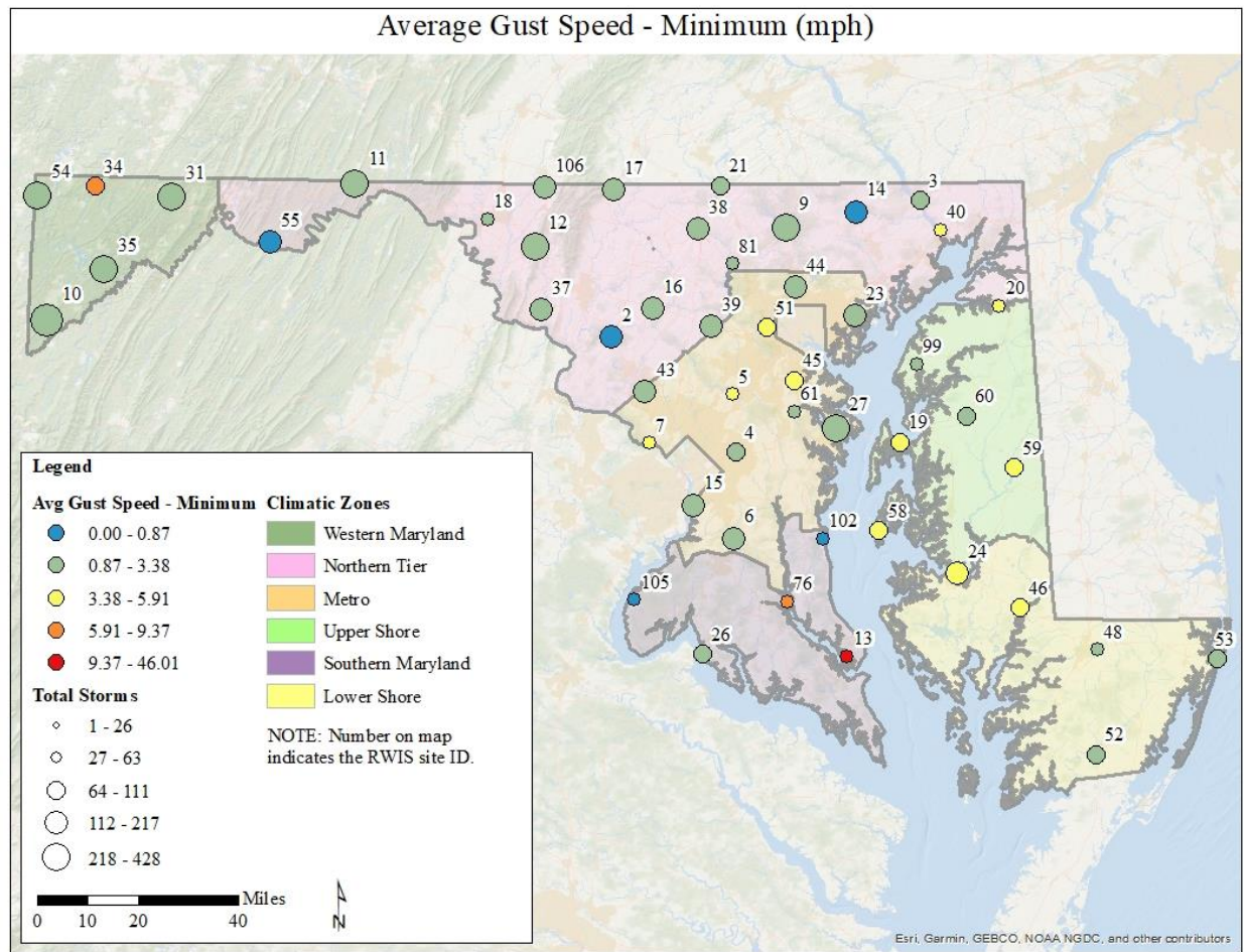
Figure 85. Shows the minimum of the average wind gust speed in miles per hours (mph) for each storm event at each RWIS location in Maryland from 2012-2019.
