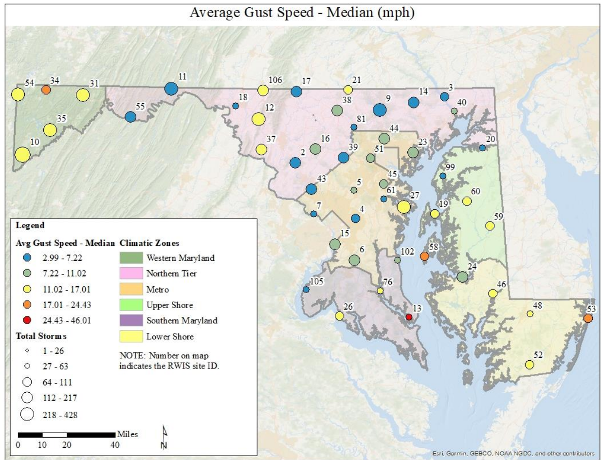
Figure 84. Shows the median of the average wind gust speed in miles per hours (mph) for each storm event at each RWIS location in Maryland form 2012-2019.
