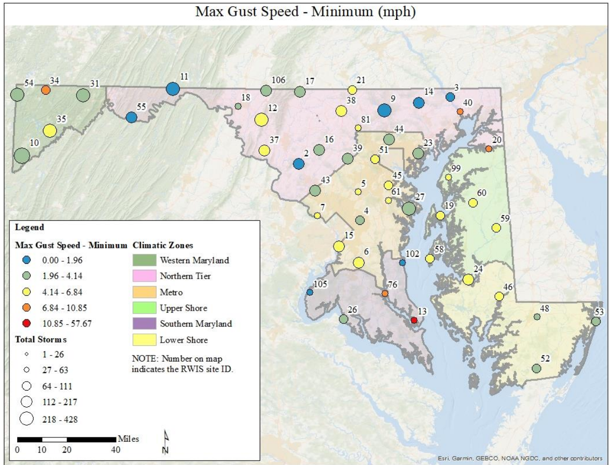
Figure 89. Shows the minimum of the maximum wind gust speed in miles per hours (mph) for each storm event at each RWIS location in Maryland from 2012-2019.
