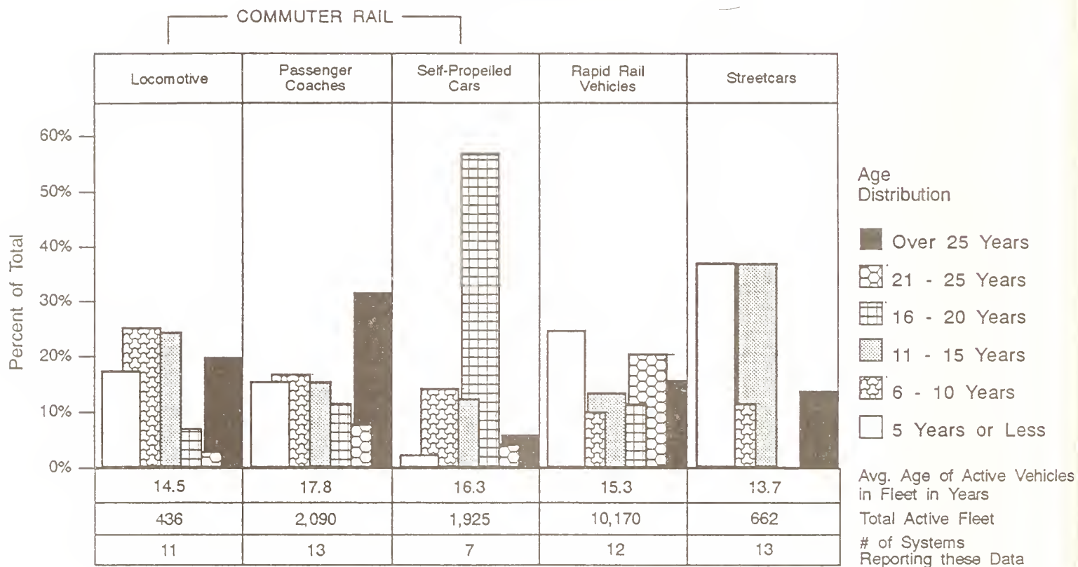
FIGURE 2.09.2 SUMMARY AGE DISTRIBUTION OF REVENUE VEHICLE INVENTORY BY VEHICLE TYPE
