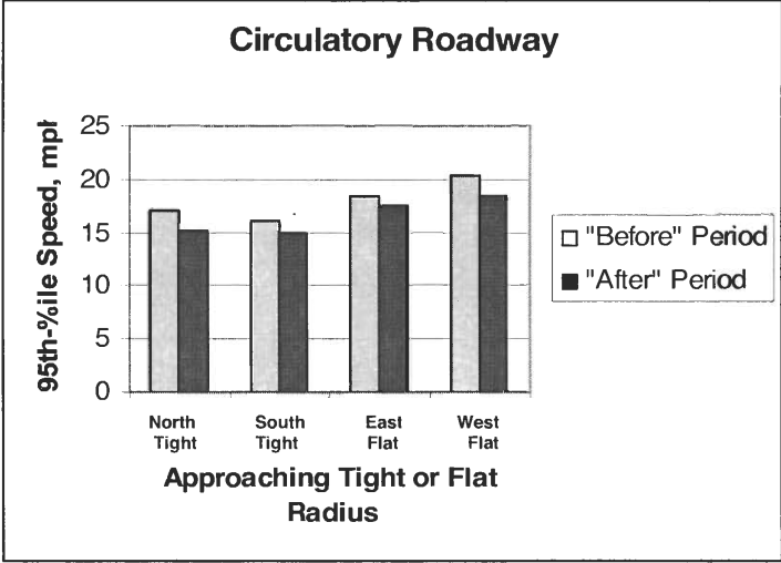
FIGURE 15 Graphical View of Difference in “Before” and “After” Period 95 th -Percentile Speeds, mph
