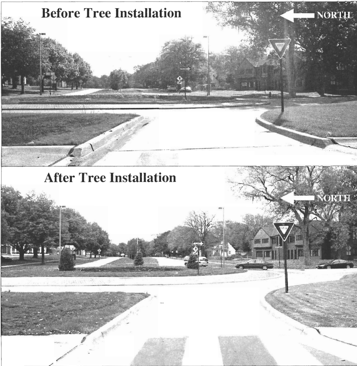
FIGURE 7 Before and After Views of Central Island from West Approach on Sheridan Blvd, 10 ft in Advance of Pedestrian Crossing
