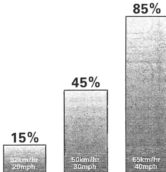
FIGURE 23 Pedestrian Chance of Fatality If Hit by Motor Vehicle
