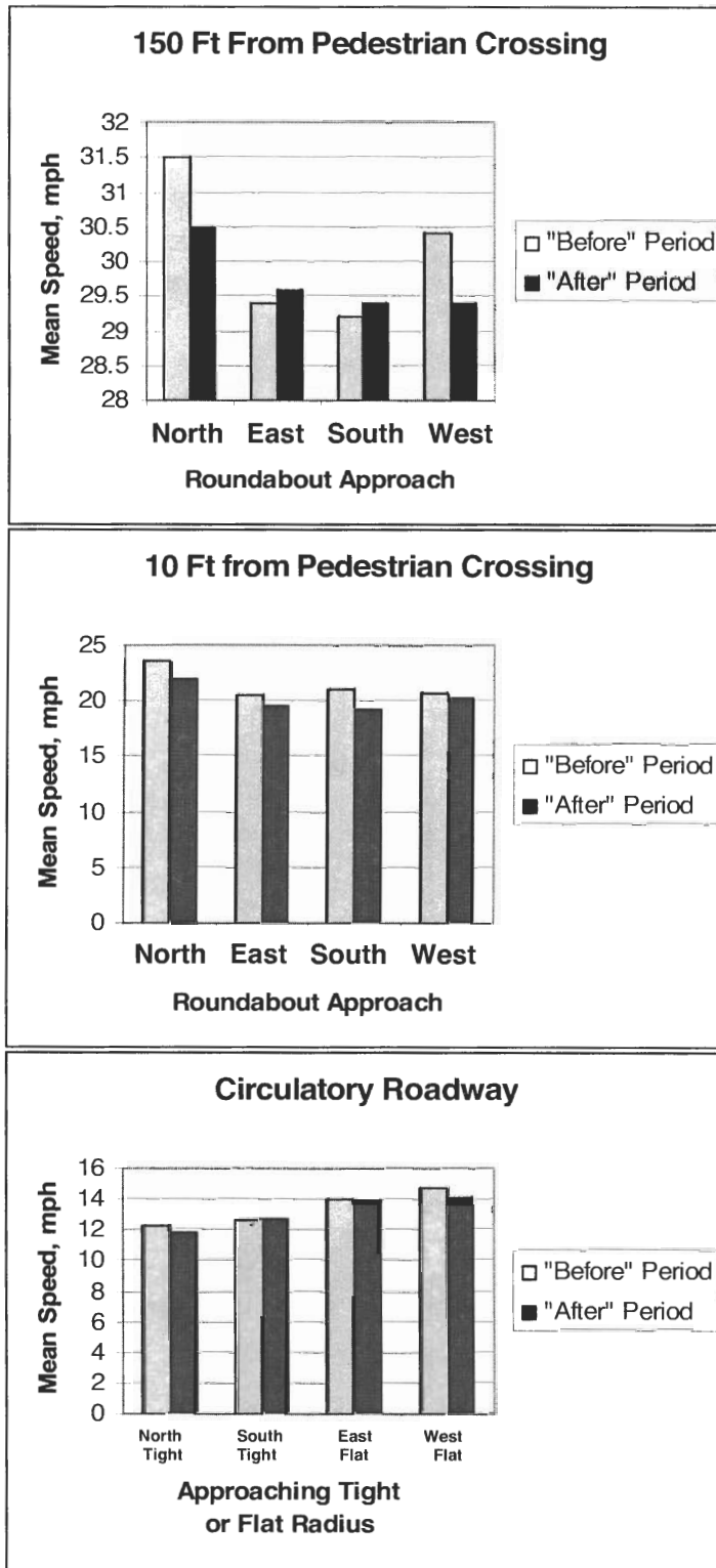
FIGURE 13 Graphical View of Difference in “Before” and “After” Period Mean Speeds, mph
