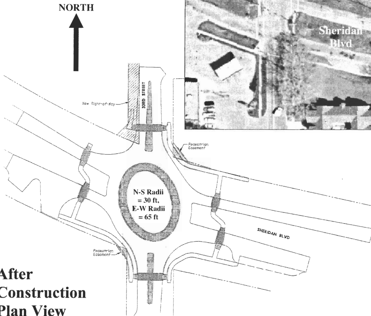
FIGURE 6 Before Construction Aerial Photograph and After Construction Line Drawing of the Sheridan Blvd and 33 rd Street Intersection
