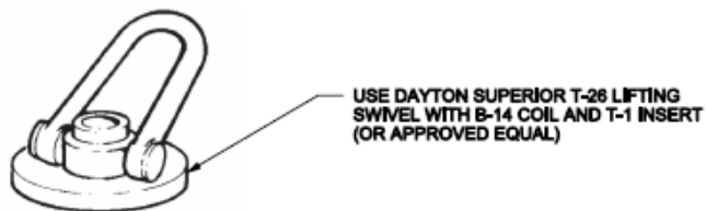
Figure 12. Lifting device details.
