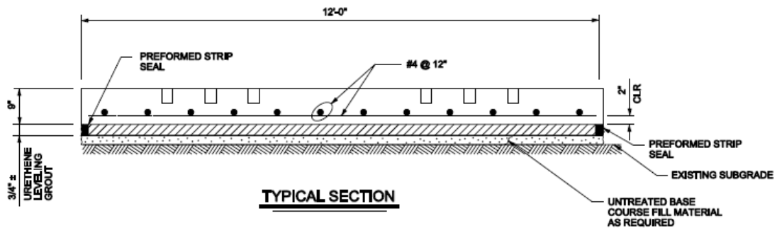
Figure 9. Typical plan view and section view for 12-ft x 12-ft panels.
