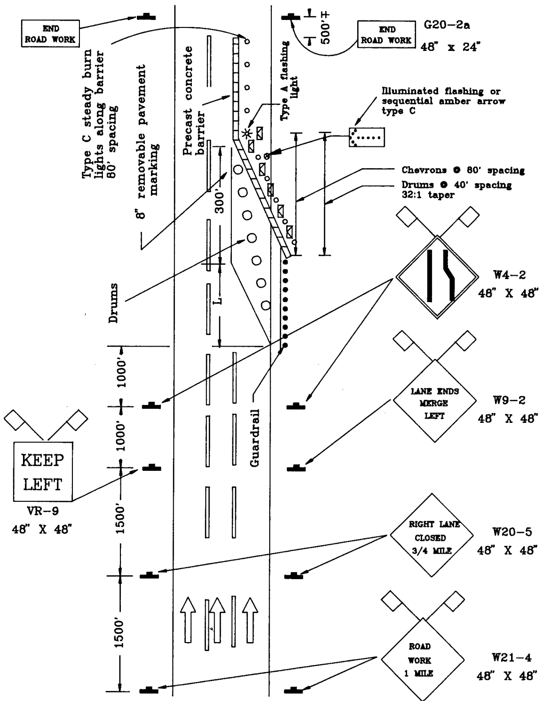
Figure 11. Chevron arrows on portable concrete safety-shaped barriers
