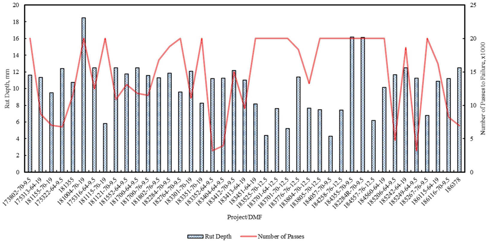
Figure E.1 HWTT data for PMFC specimens.
