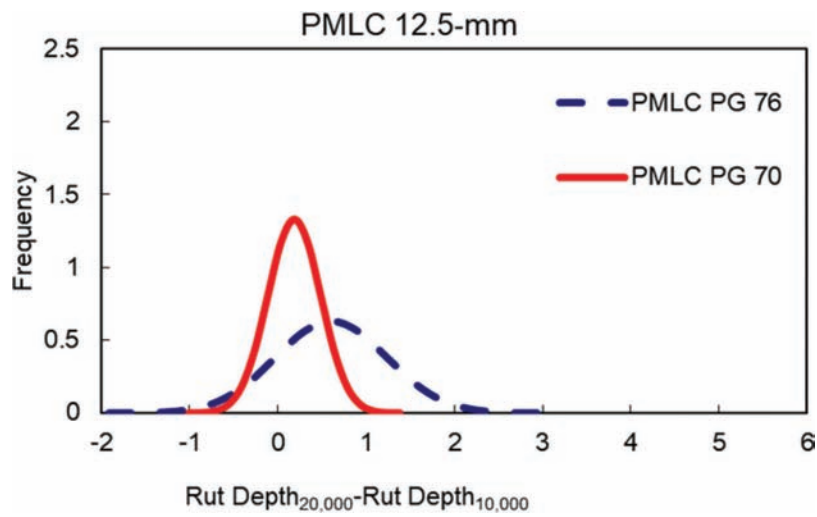
Figure 3.42 Moisture susceptibility distributions for 12.5-mm mixture specimens.
