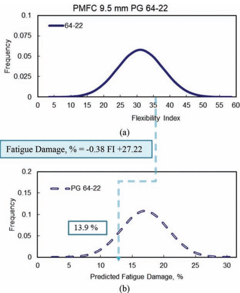
Figure 4.8 Development of predicted pavement performance distributions.
