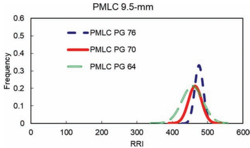
Figure 3.38 Rutting resistance index distributions for 9.5-mm mixture specimens.
