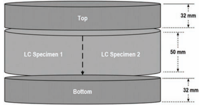
Figure 3.2 Schematic of test specimen preparation.
