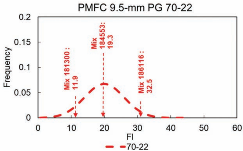
Figure 3.30 Flexibility index distribution and corresponding rankings for 9.5-mm mixture containing PG 70-22.
