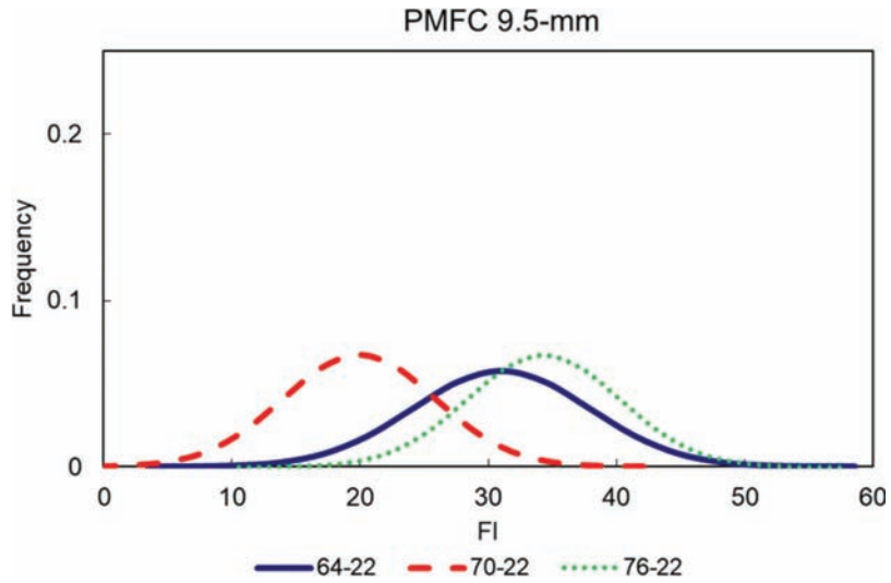
Figure 3.16 9.5-mm mixture PMFC flexibility index distributions.
