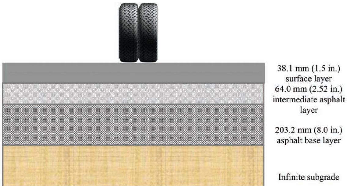
Figure 4.1 Full-depth asphalt pavement section used in FlexPAVE.
