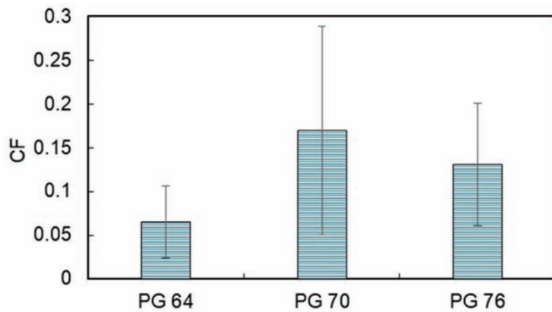
Figure 3.34 Average C_F values for mixtures with different binder grades.
