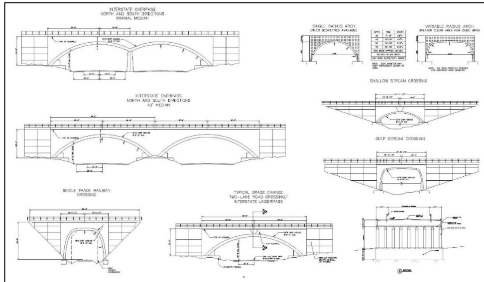
Figure 8: Different geometry applications of CFFT bridge spans [59].
