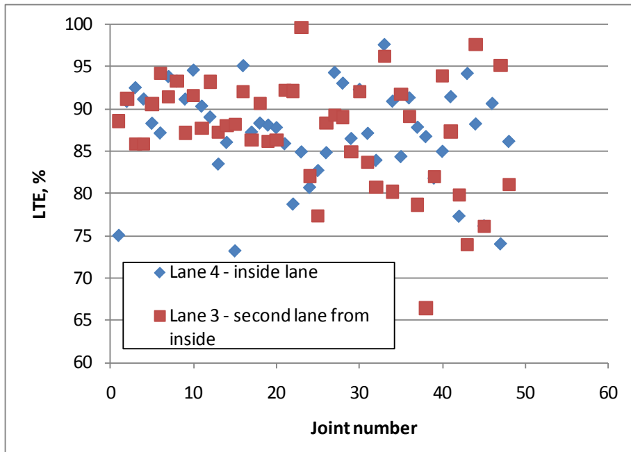
Figure 64. LTE across the joints tested in lanes 3 and 4 of the mainline.
