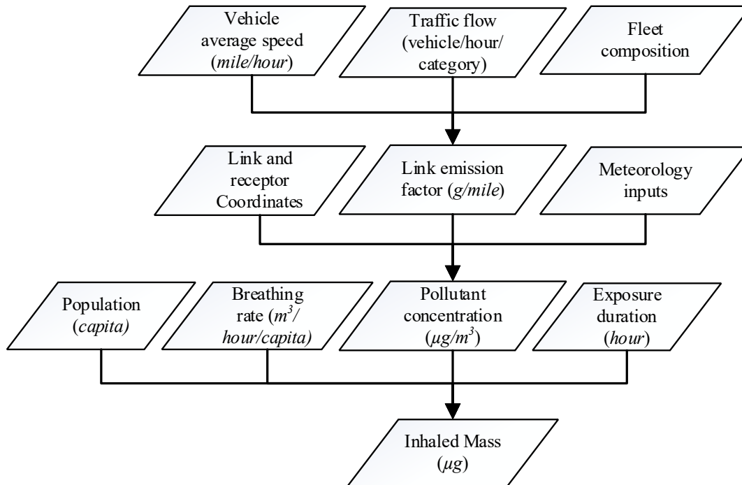
Figure 3. Critical link-based inputs for the overall exposure modeling method
