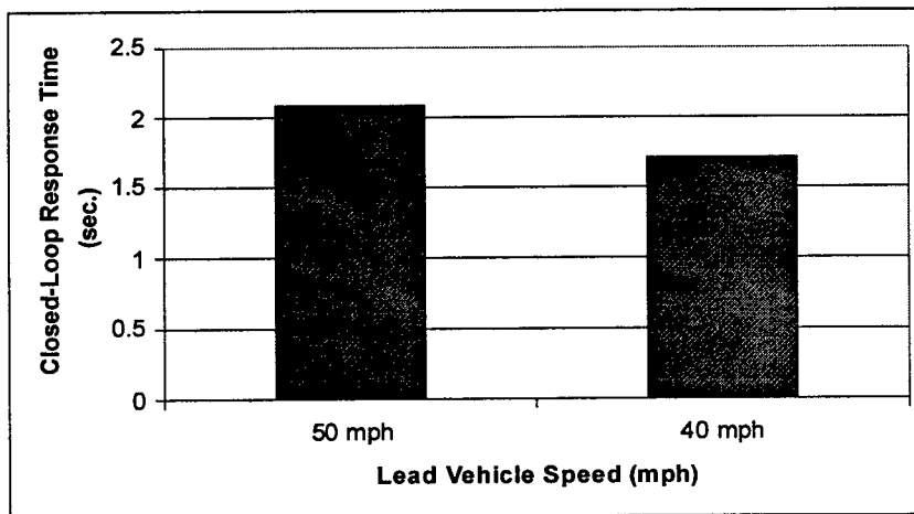
Figure 3.1. Closed-Loop Response Times at 40 and 50 mph (17.88 and 22.35 m/sec).
