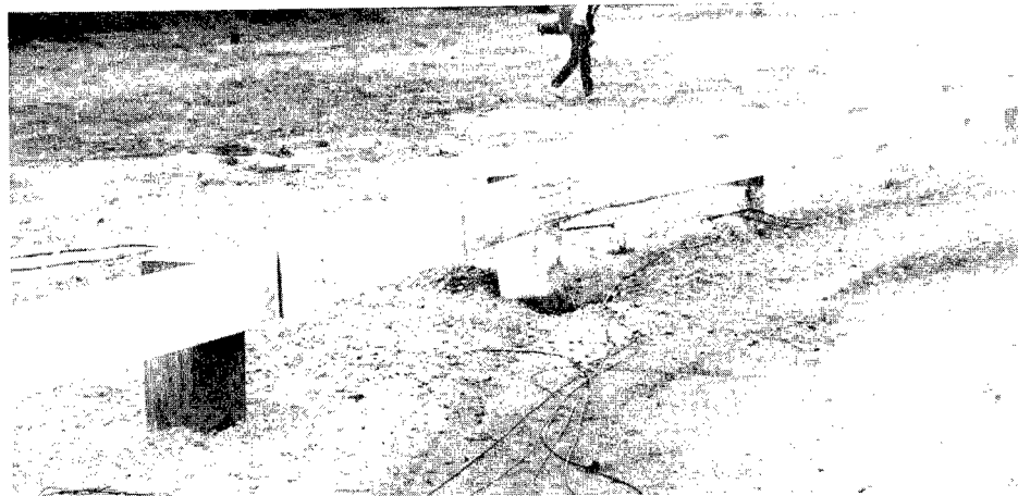
Figure 73. Posttest photographs of guardrail system, test 1818-8-88.
