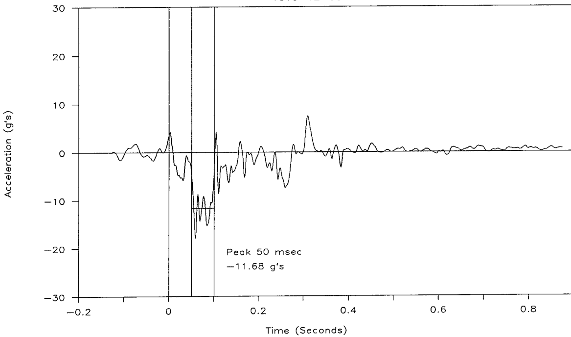
Figure 87. Vehicle acceleration, test 1818-12-88.
