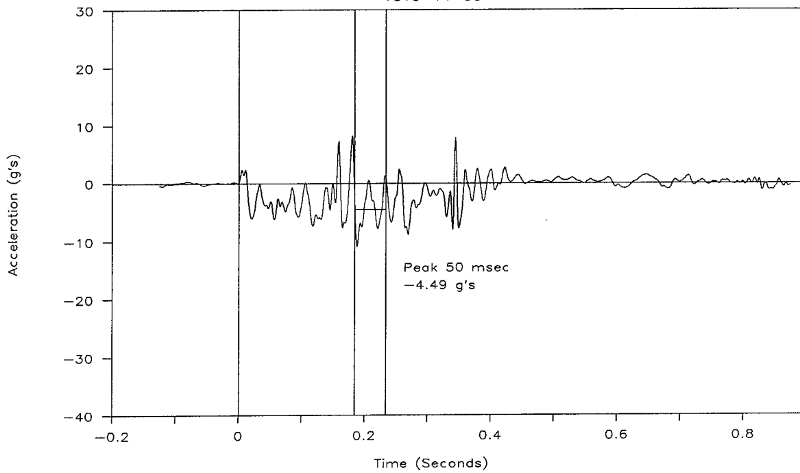
Figure 95. Vehicle acceleration, test 1818-14-88.
