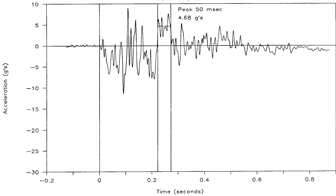
Figure 24. Vehicle acceleration, test 1818-5-2-87.
