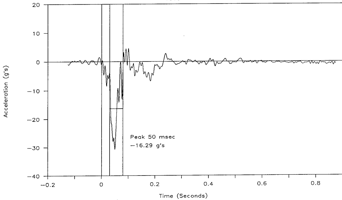
Figure 63. Vehicle acceleration, test 1818-7-88.
