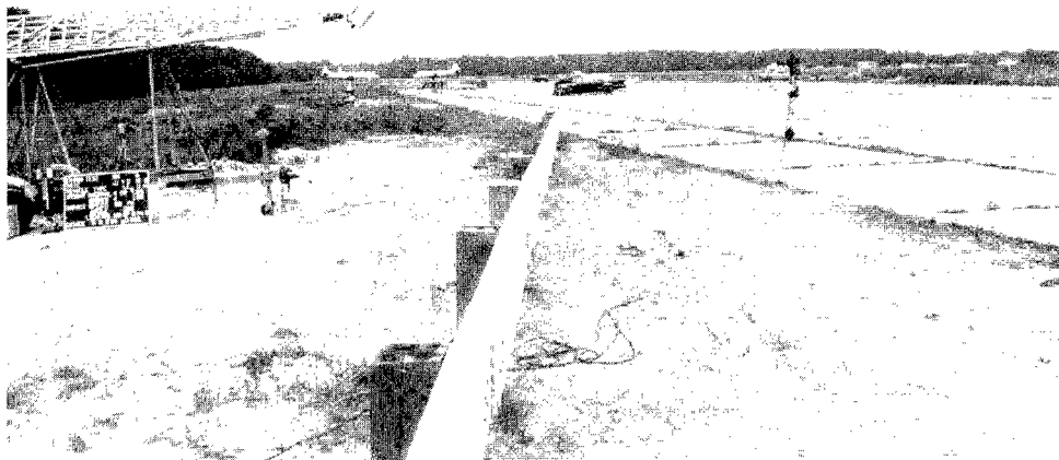
Figure 92. Pretest photographs of guardrail system, test 1818-14-88.
