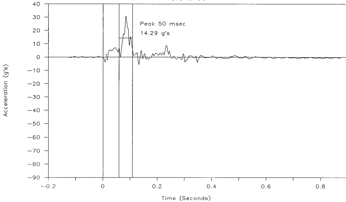
Figure 79. Vehicle acceleration, test 1818-9-90.
