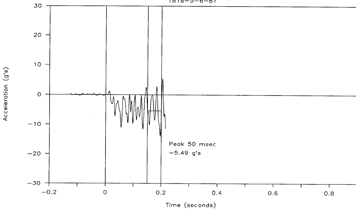
Figure 55. Vehicle acceleration, test 1818-5-6-87.
