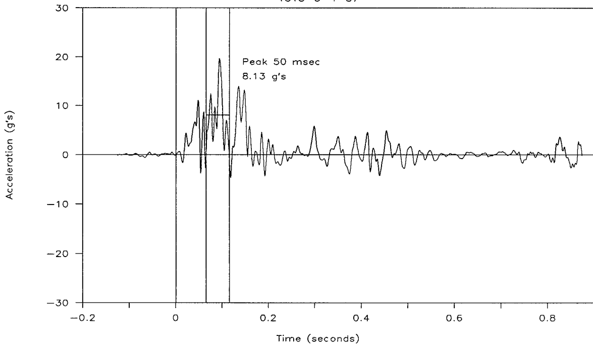
Figure 40. Vehicle acceleration, test 1818-5-4-87.
