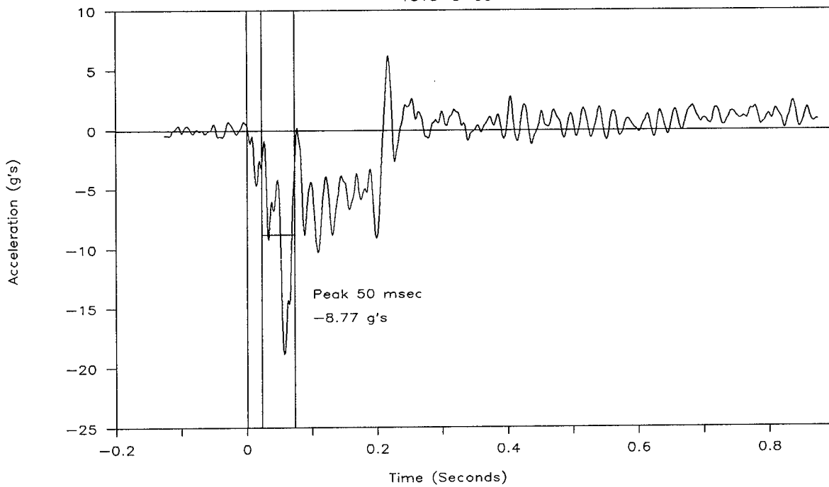
Figure 71. Vehicle acceleration, test 1818-8-88.
