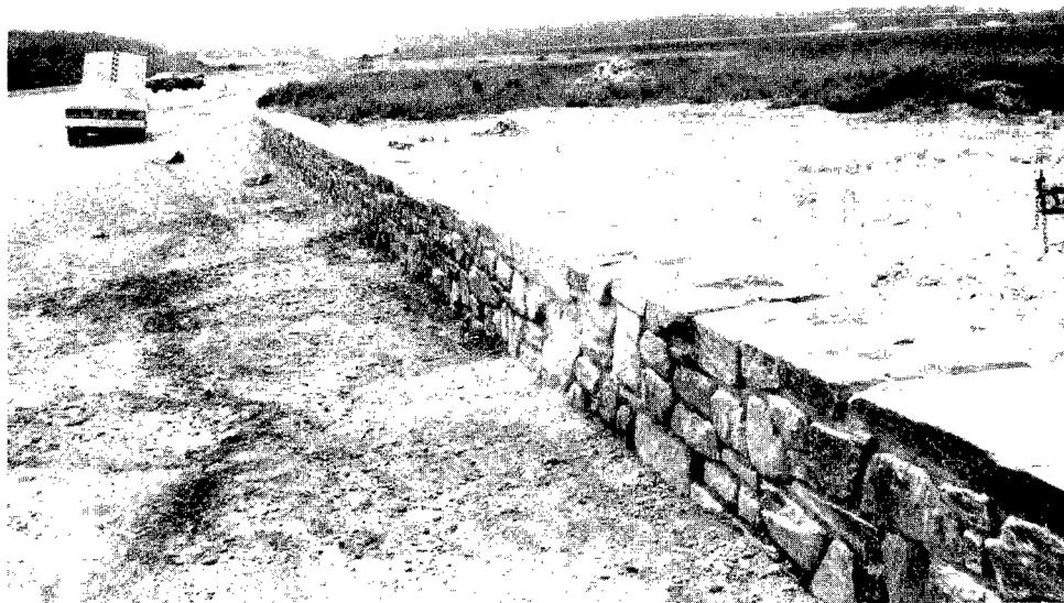
Figure 49. Posttest photographs of guardwall system, test 1818-5-88.
