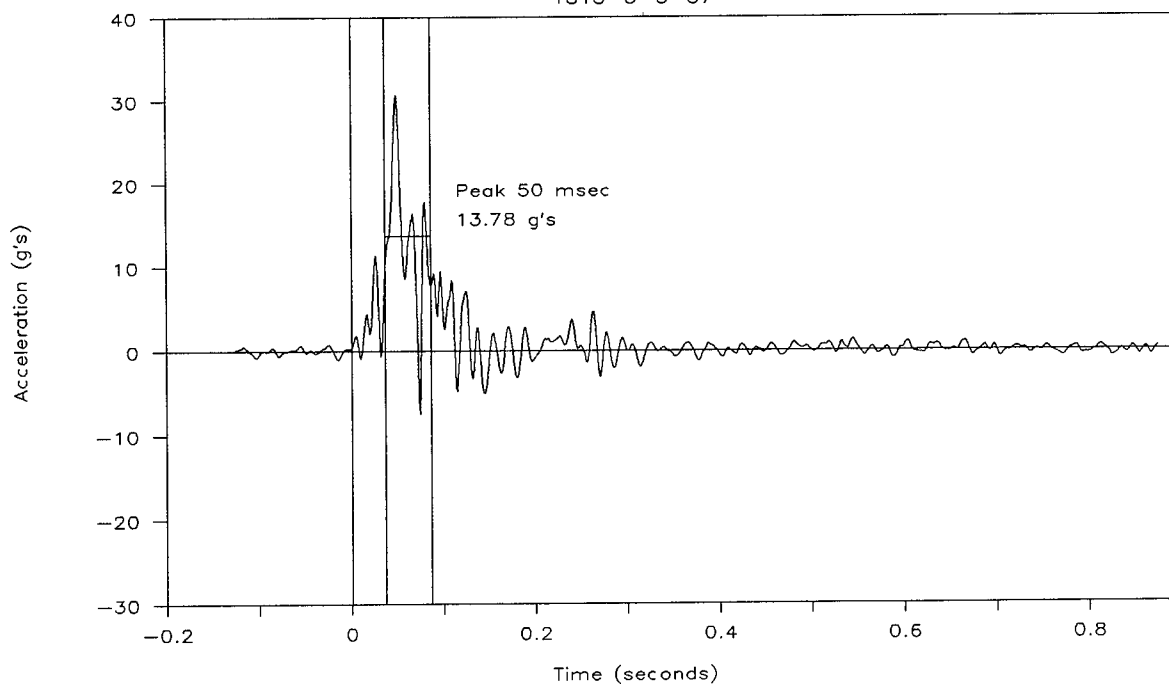
Figure 32. Vehicle acceleration, test 1818-5-3-87.
