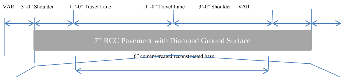
Figure 5. Diagram. Section 1 typical pavement from log mile 2.02 to log mile 2.88 of State Highway 213.
