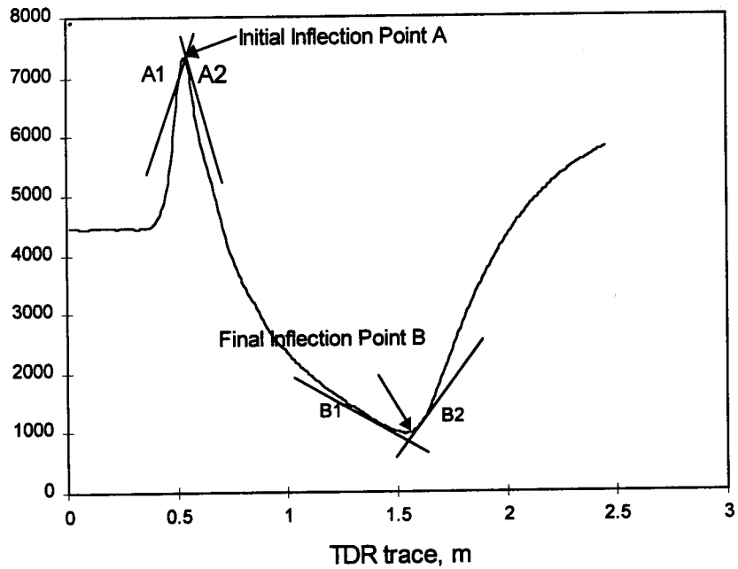
Figure 6. Illustration of the Method of Peaks (section 510113).
