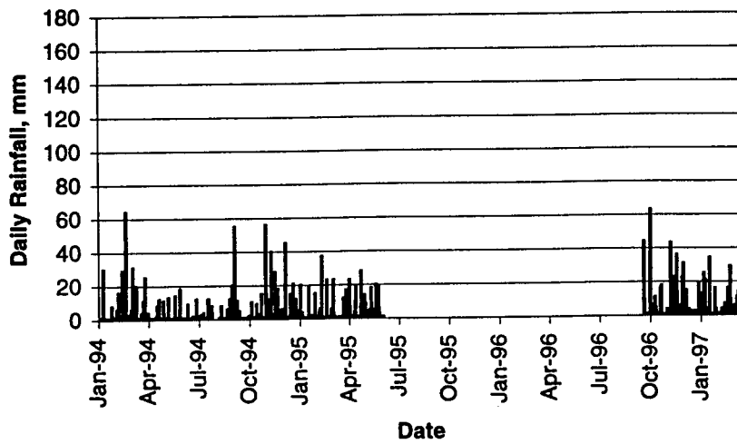
Figure 87. Seasonal variation in volumetric and gravimetric moisture content and daily rainfall for section 091803 in Connecticut.
