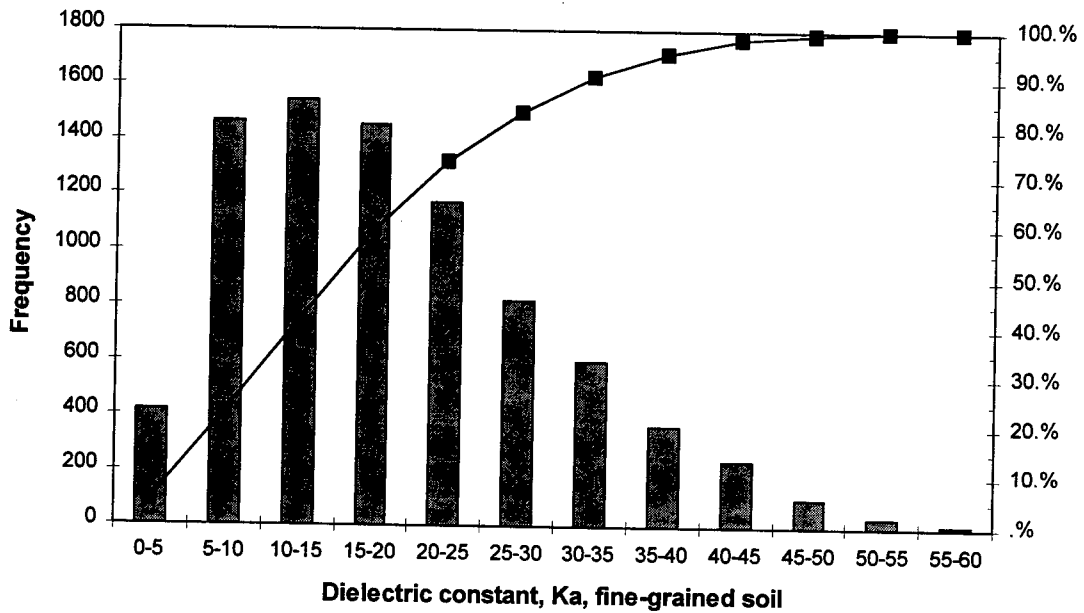
Figure 16. Frequency distribution of the dielectric constants for the LTPP SMP fine-grained soils.
