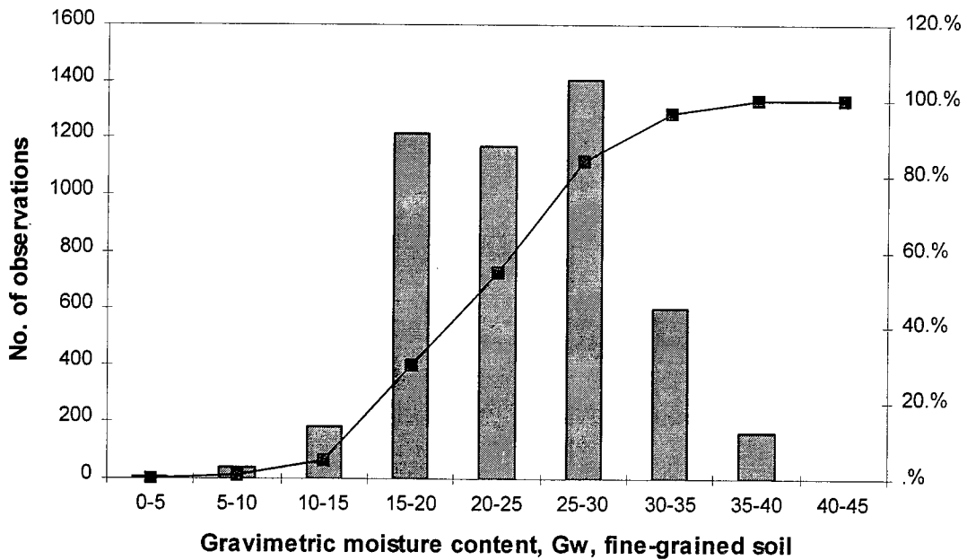
Figure 44. Frequency distribution of the computed gravimetric moisture contents using the TDR traces collected at SMP sites, fine-grained material.
