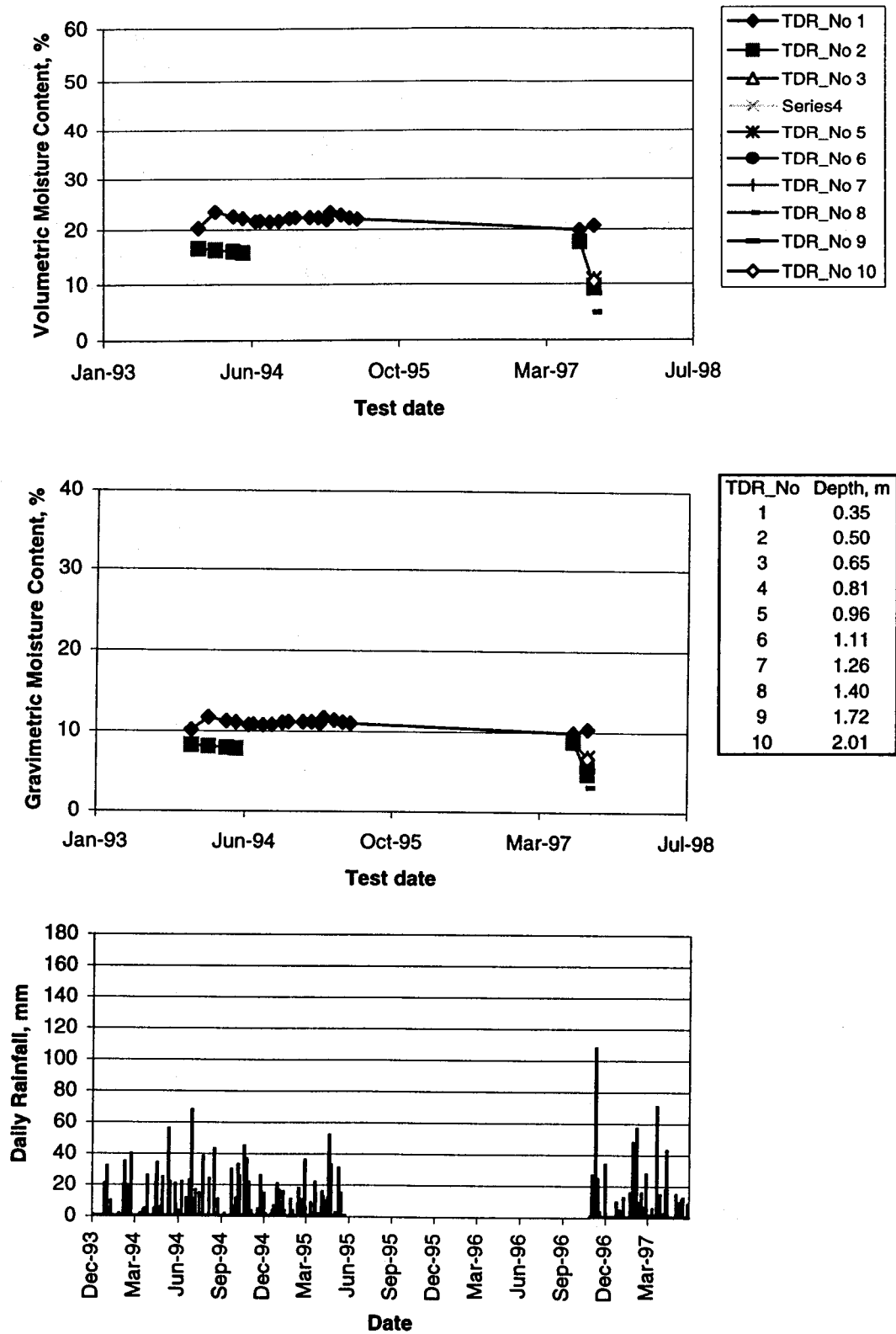
Figure 118. Seasonal variation in volumetric and gravimetric moisture content and daily rainfall for section 481068 in Texas.
