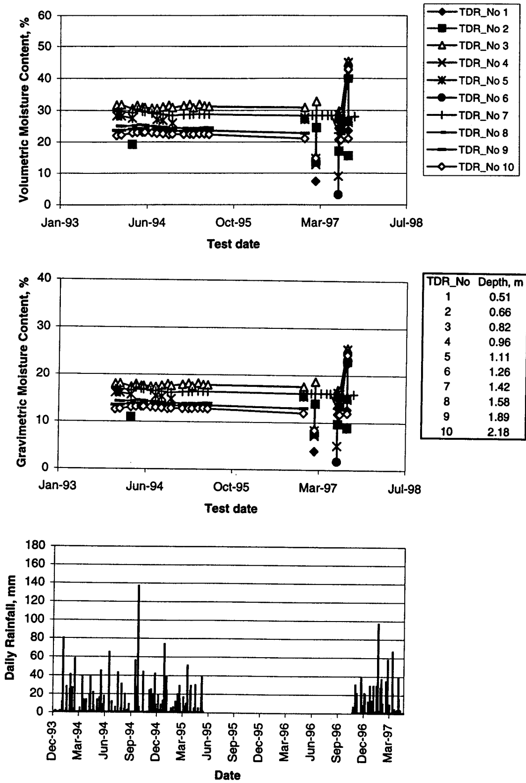
Figure 122. Seasonal variation in volumetric and gravimetric moisture content and daily rainfall for section 484142 in Texas.
