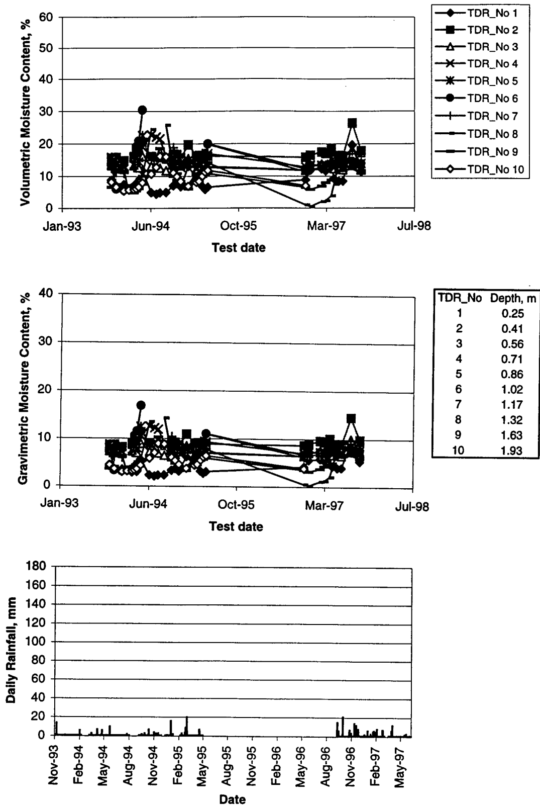
Figure 124. Seasonal variation in volumetric and gravimetric moisture content and daily rainfall for section 491001 in Utah.
