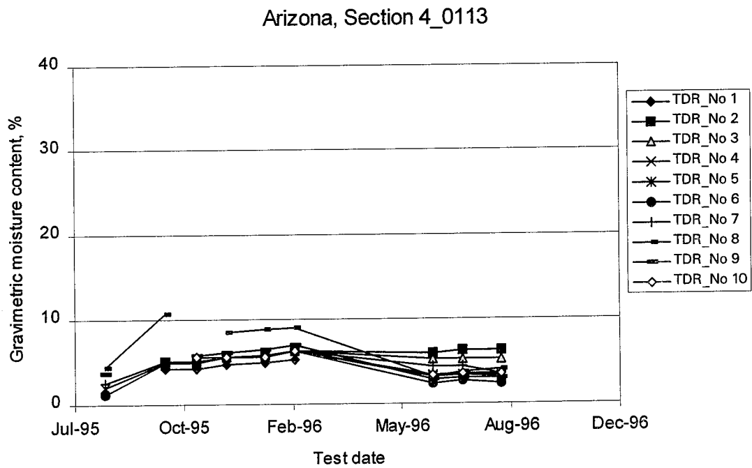
Figure 46. Example of seasonal variation in gravimetric moisture content for section 040113 in Arizona.
