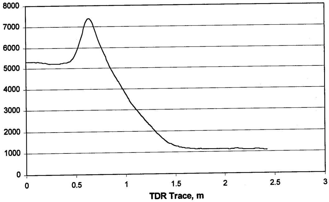
Figure 11. Example TDR trace for which error code "b1" applies (section 331001).
