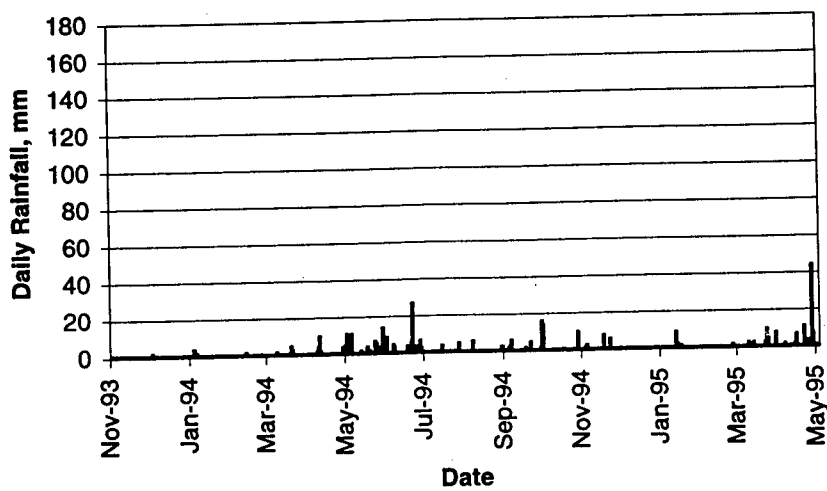
Figure 103. Seasonal variation in volumetric and gravimetric moisture content and daily rainfall for section 308129 in Montana.
