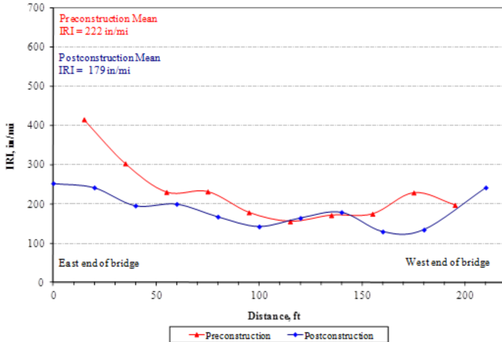
Figure 26. Mean IRI values computed at 20-ft intervals before and after construction.
