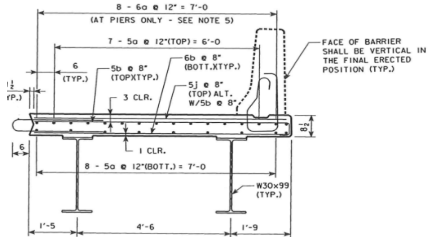
Figure 7. Cross section of a typical exterior module.
