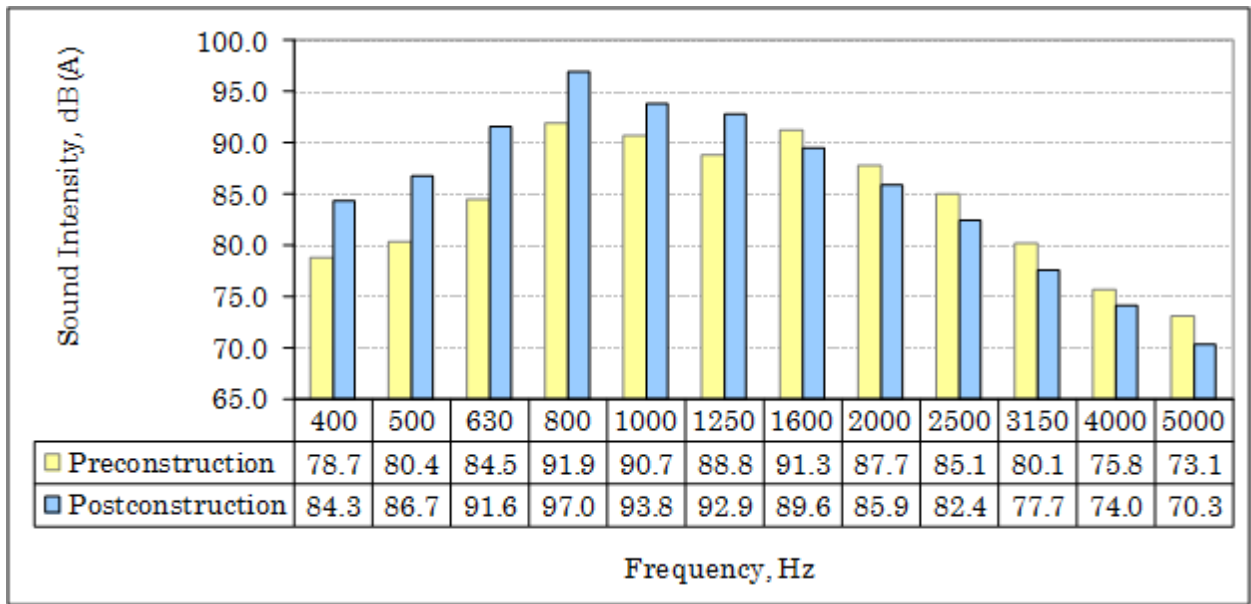
Figure 24. Mean A-weighted SI frequency spectra before and after construction.
