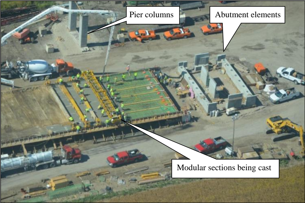
Figure 5. View during the modular section pour.
