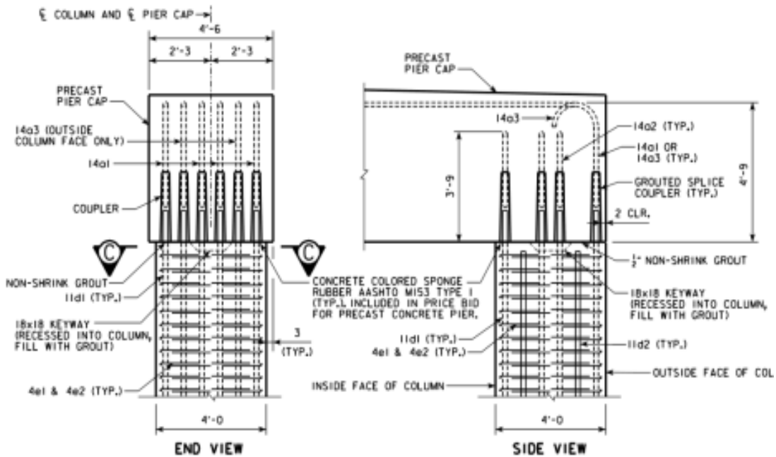
Figure 11. Cap to column detail.
