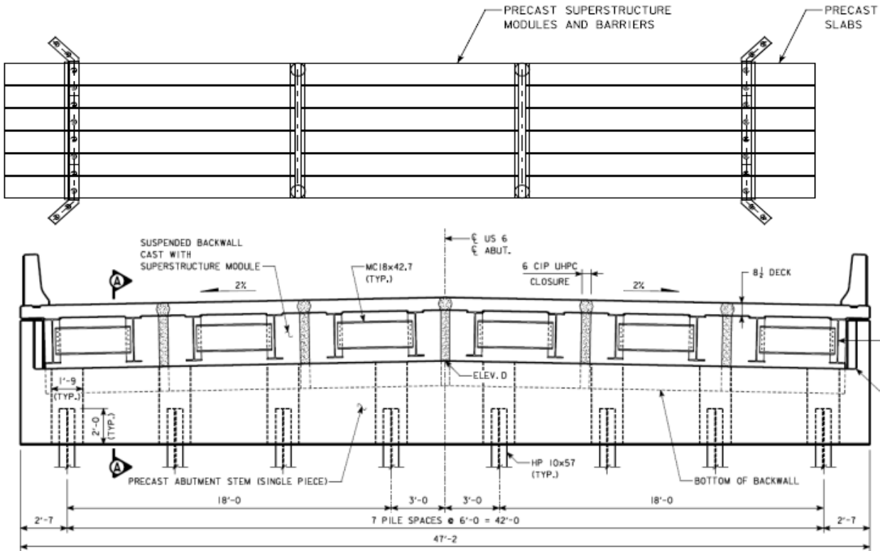
Figure 6. Modular section plan and cross section.
