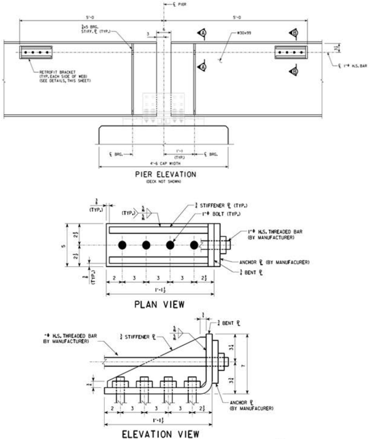
Figure 20. Post-tension retrofit design.
