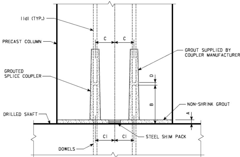
Figure 12. Detail of the drilled shaft to column connection.
