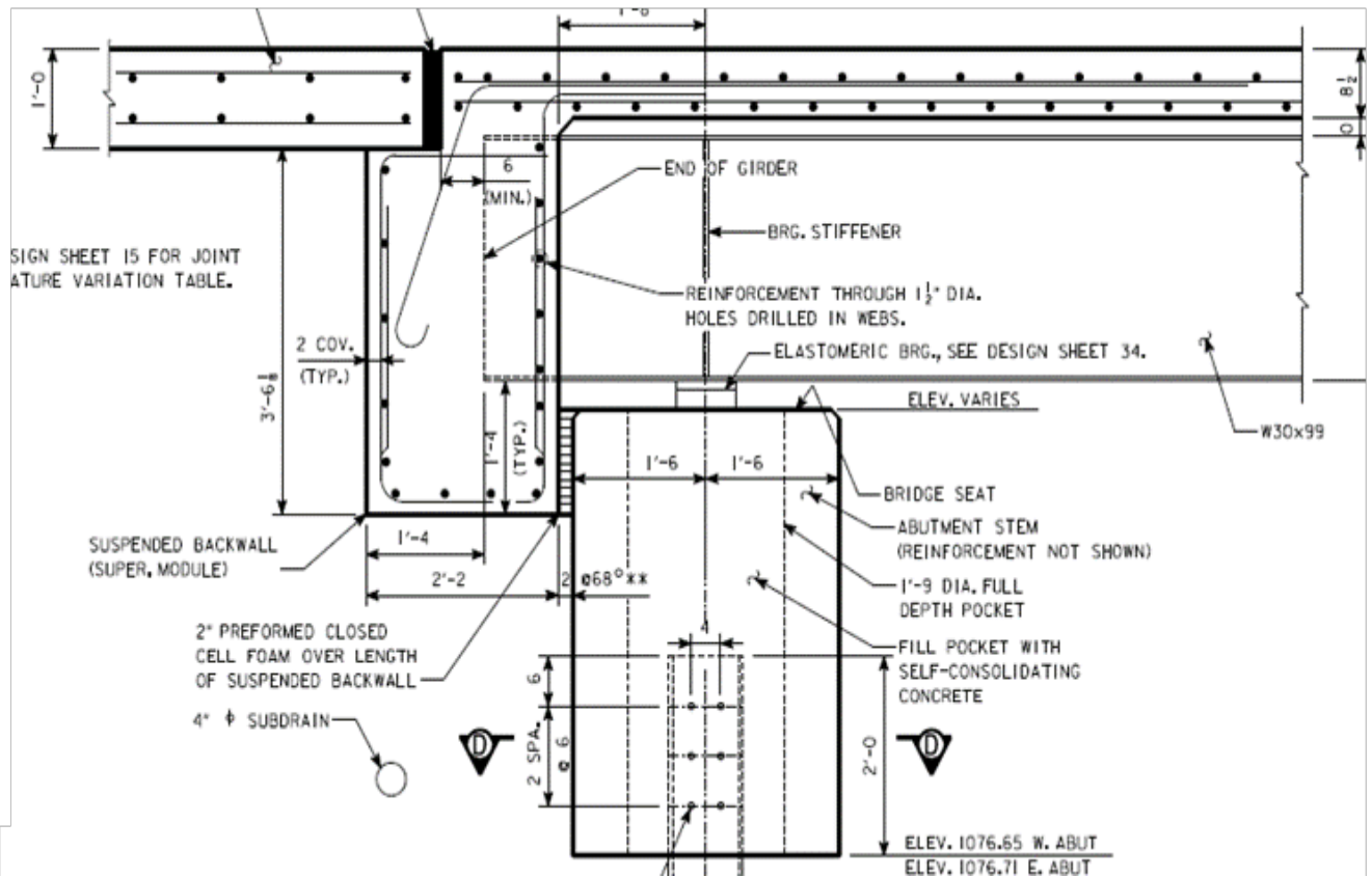
Figure 13. Suspended backwall detail.
