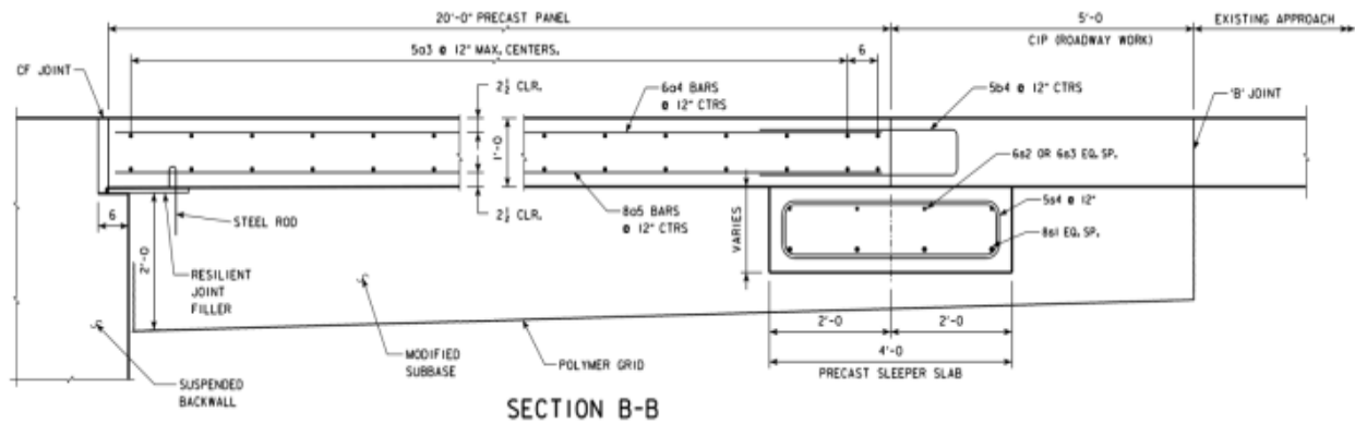
Figure 17. Approach slab cross section.
