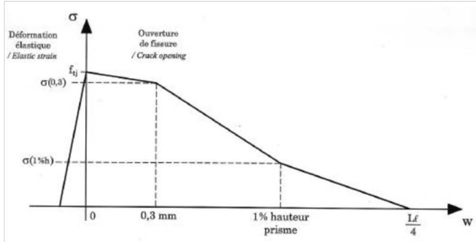
Figure 17 A relationship proposed for the UHPC tensile strength variation as a function of crack width (AFGC 2002).
