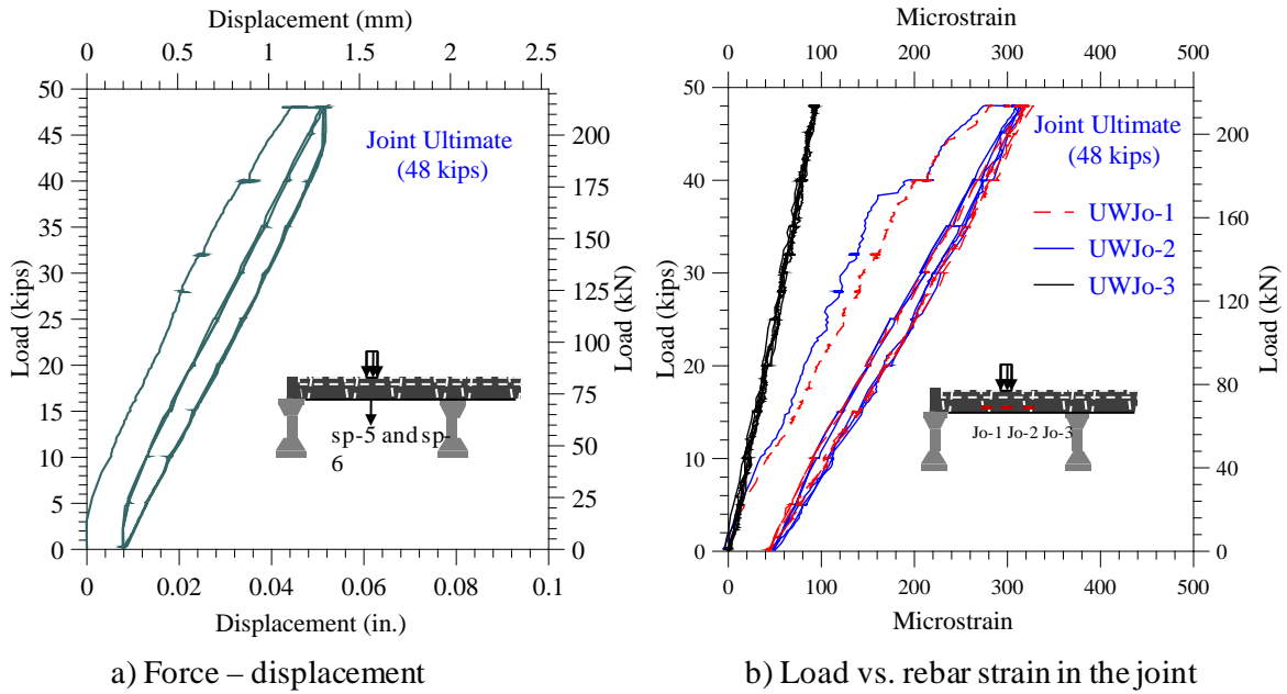
Figure 28 Measured force-displacement response and peak rebar strain at the center of the joint at the ultimate load of 48 kips.
