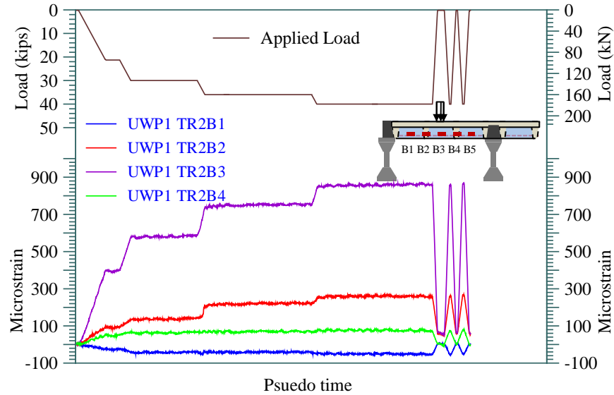
Figure 39 Measured strains in the bottom reinforcement of the transverse rib along the length of UWP1 at during the ultimate load test.
