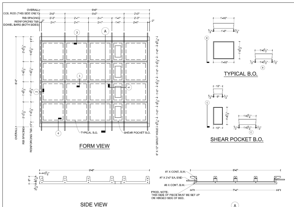
Figure 1 Prototype Panel Shop Drawing
