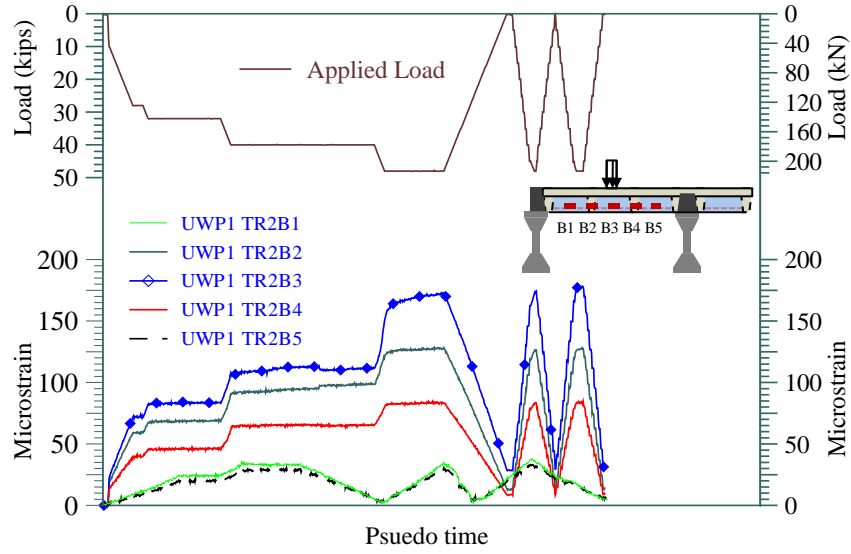
Figure 30 Measured strains in the bottom reinforcement of transverse rib TR2 along the length of Panel UWP1 at the ultimate load.
