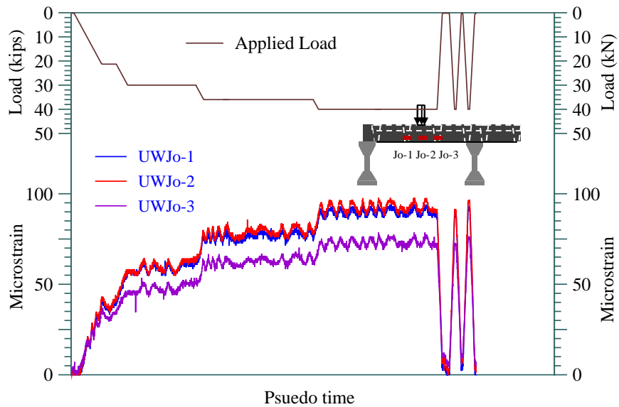
Figure 40 Measured strains in the bottom reinforcement of the joint along the joint length during the ultimate load test.
