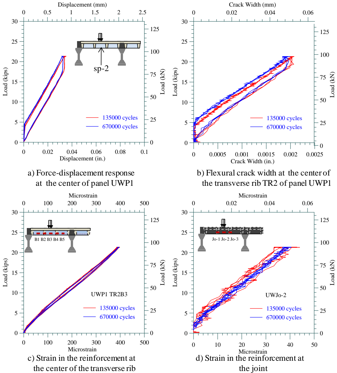
Figure 37 Measured responses of the waffle deck system for static service load tests conducted during the panel fatigue test.
