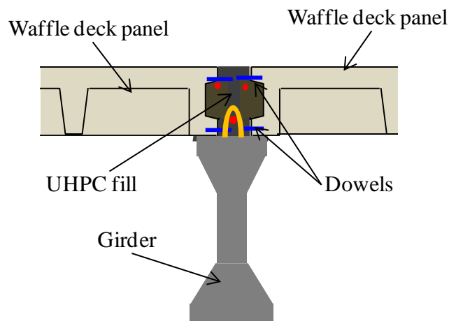
Figure 3 Connection details between the central girder and the waffle deck
