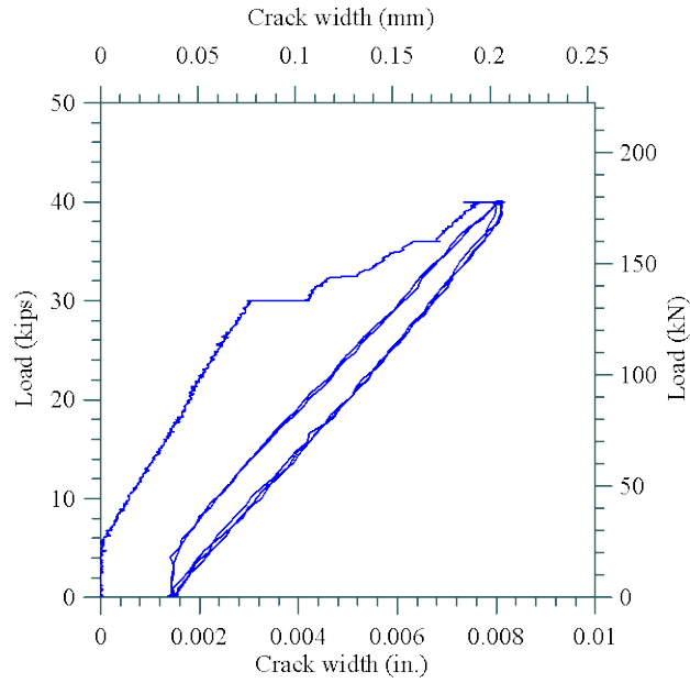
Figure 42 Measured crack width in transverse rib TR2 of UWP1 at during the ultimate load test.
