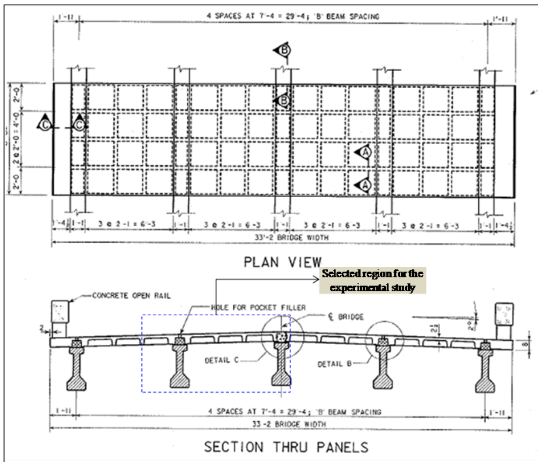
Figure 1 Plan and cross section details of the proposed UHPC Waffle Deck Bridge in Wapello County.
