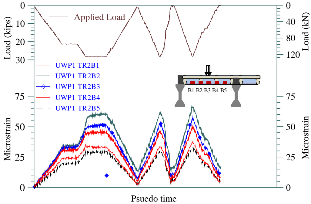
Figure 21 Measured strains in the bottom reinforcement of the transverse rib (TR2) along the length of panel UWP1 at service load.
