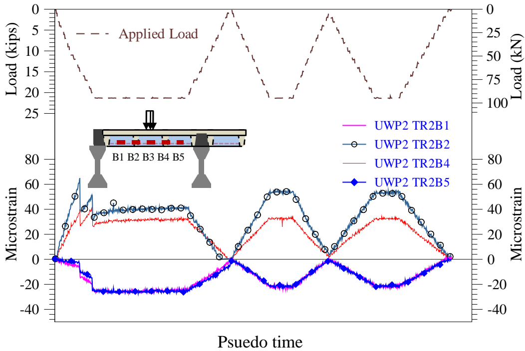
Figure 14 Measured strains along the bottom reinforcement of the transverse rib TR2 of panel UWP2.
