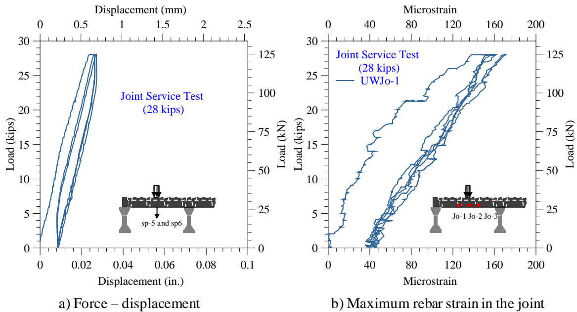
Figure 18 Measured force-displacement response and peak rebar strain at the center of the joint at the service load.
