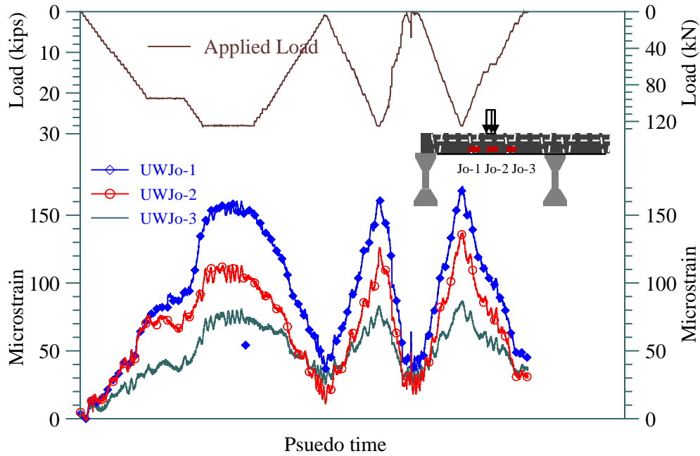
Figure 19 Measured strains along the bottom reinforcement of the joint during the service load test.
