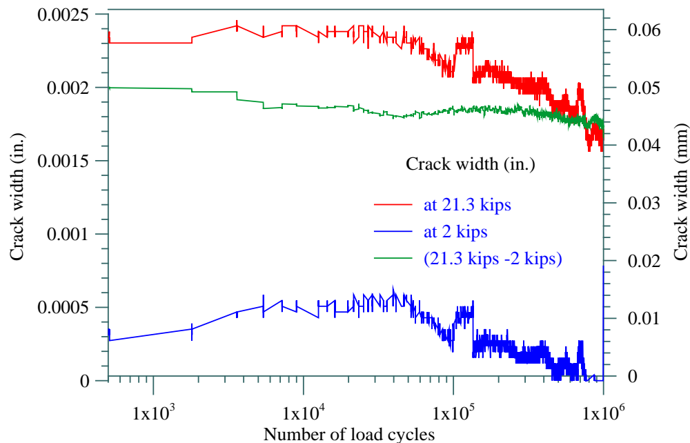
Figure 36 The crack width variation in transverse rib TR2 of panel UWP1 during panel fatigue test
