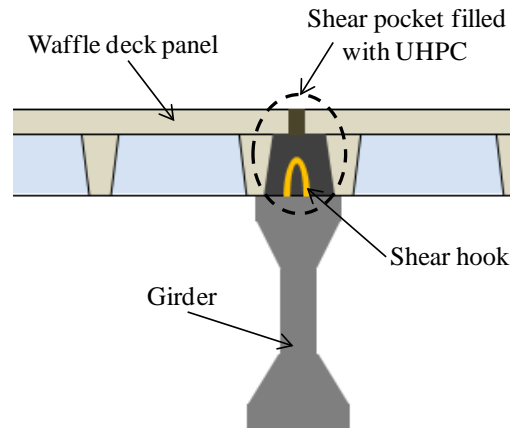
Figure 2 Shear pocket connection details between girder and the waffle deck
