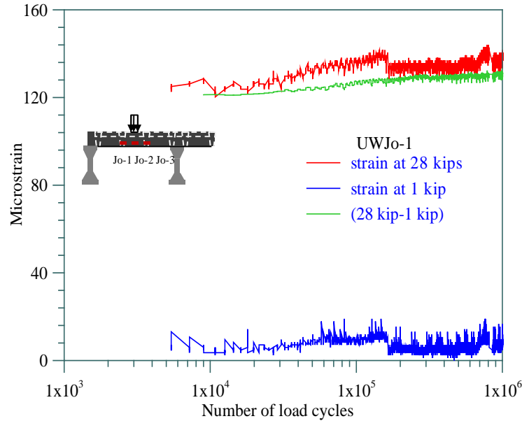
Figure 25 The variation of the peak strain in the bottom joint transverse reinforcement during the joint fatigue test.
