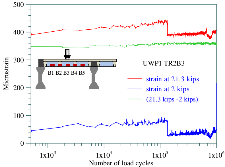
a) Peak rebar strain in the transverse rib
