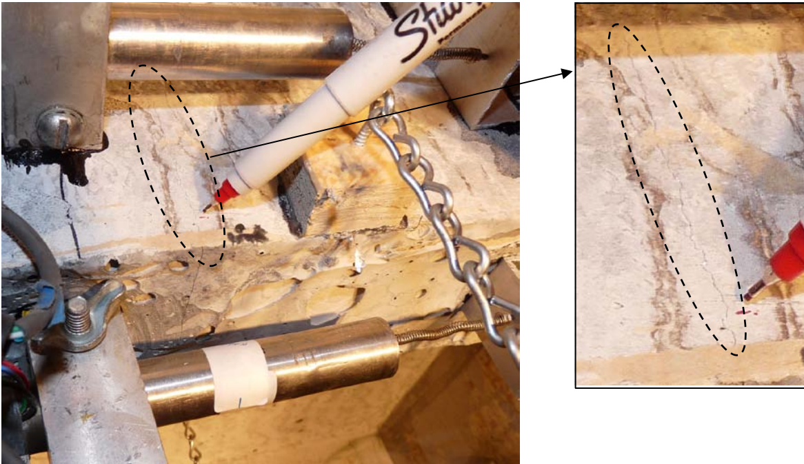
Figure 16 A hairline crack in the UWP2 panel transverse rib TR2 at 21.3 kips.
