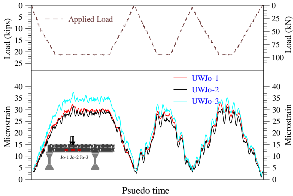
Figure 15 Measured strains along a bottom reinforcement of the panel-to-panel joint.
