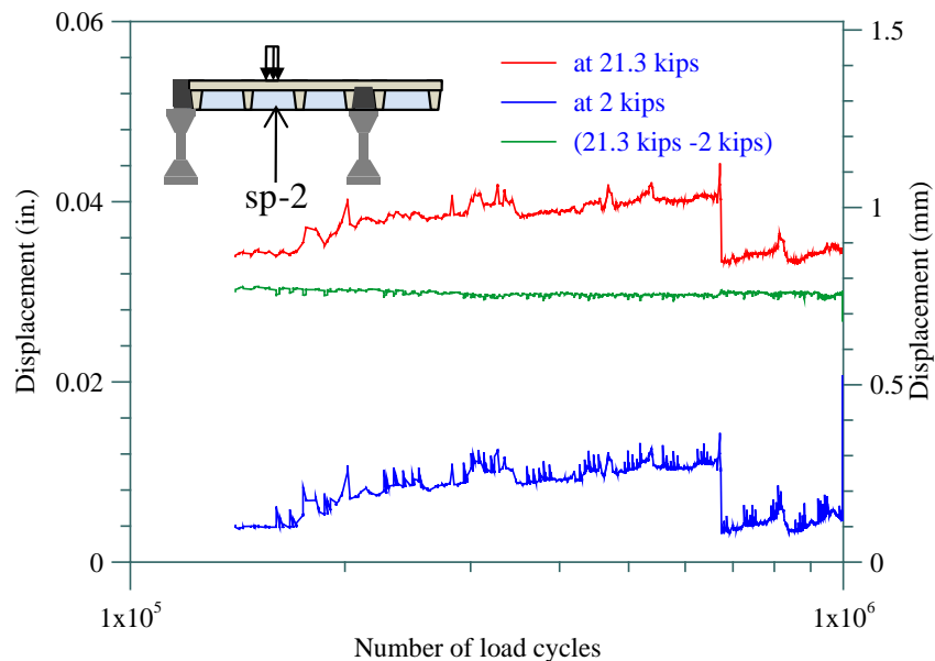
Figure 34 The peak displacement variation at the center of Panel UWP1 during the joint fatigue test.
