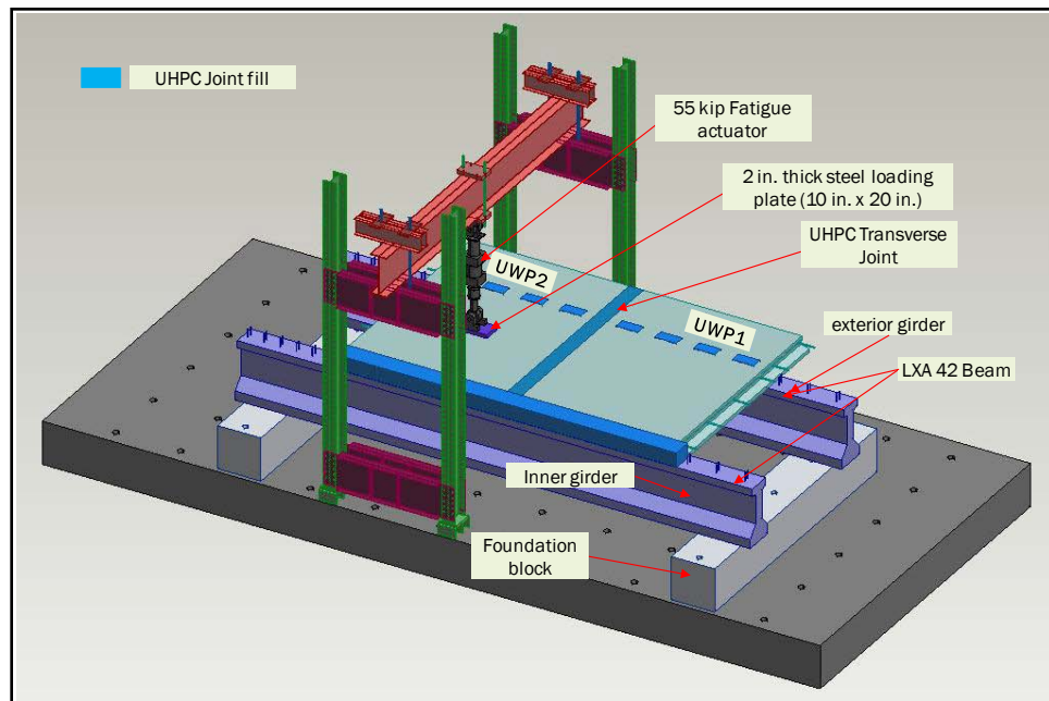
Figure 7 Schematic of the test setup used for testing of the UHPC Waffle deck panel system.
