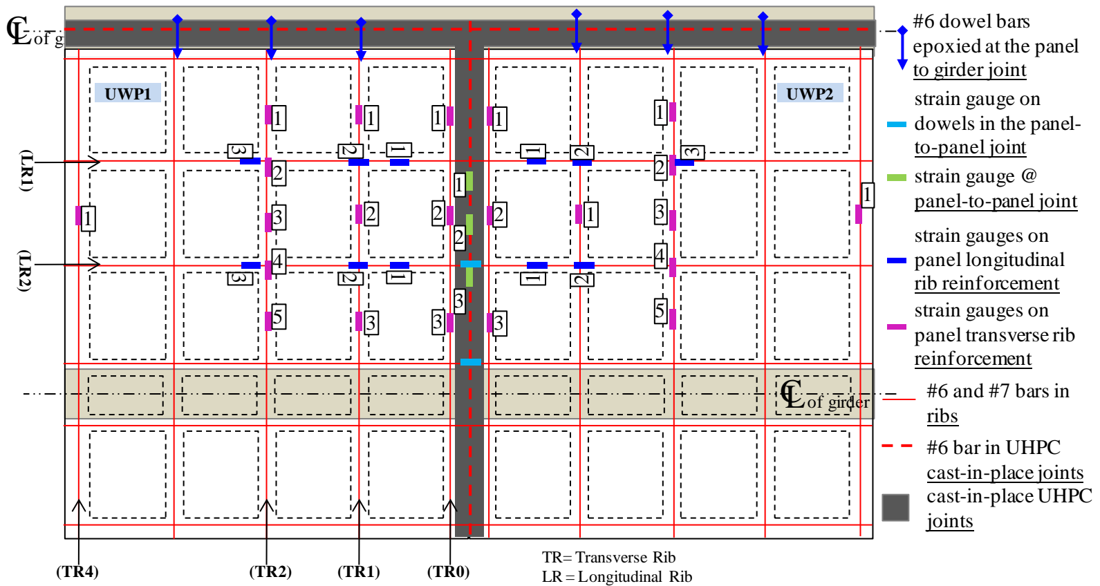
Figure 11 Location of strain gauges used on the bottom deck reinforcing bars.
