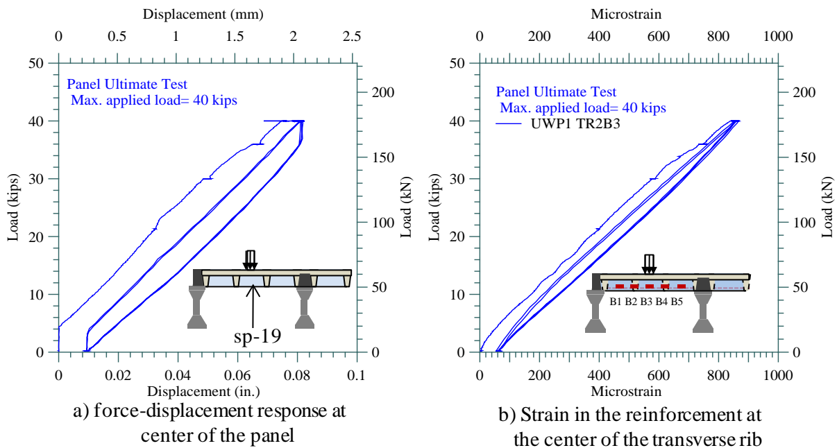
Figure 38 Measured force-displacement response and peak rebar strain at the center of the transverse rib of UWP1 at the ultimate load of 40 kips.
