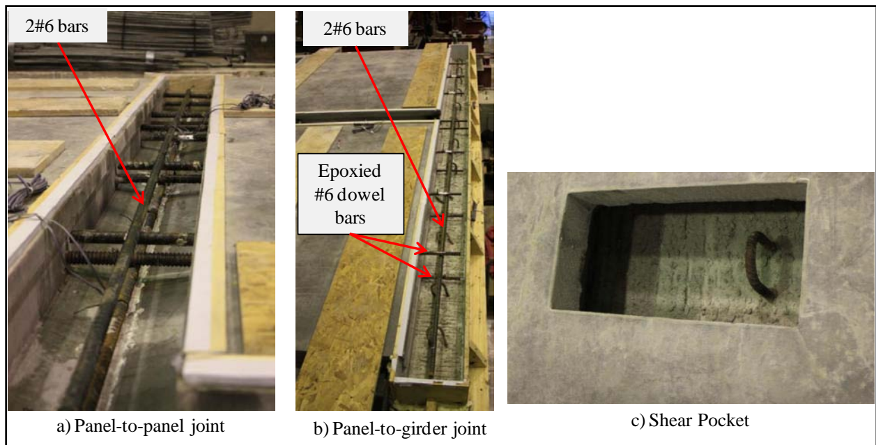
Figure 8 Details of the reinforcement provided in various joints.
