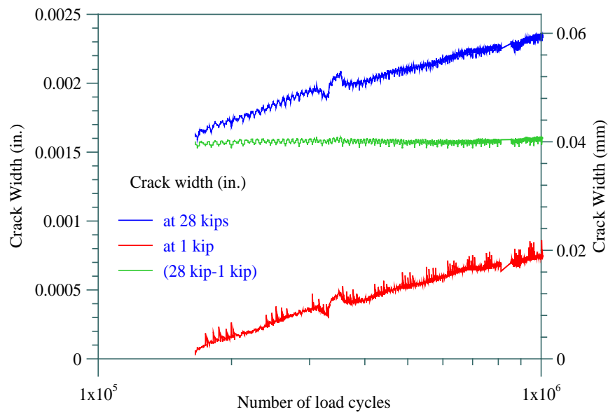
Figure 26 The variation of the crack width in the transverse joint with number of load cycles.
