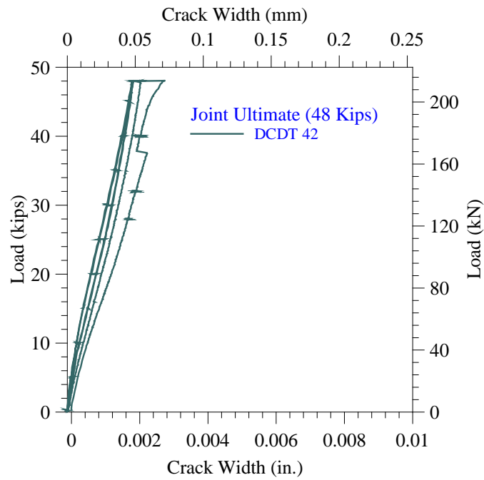
Figure 33 The variation in the width of the most critical crack in the ribs forming the transverse joint.
