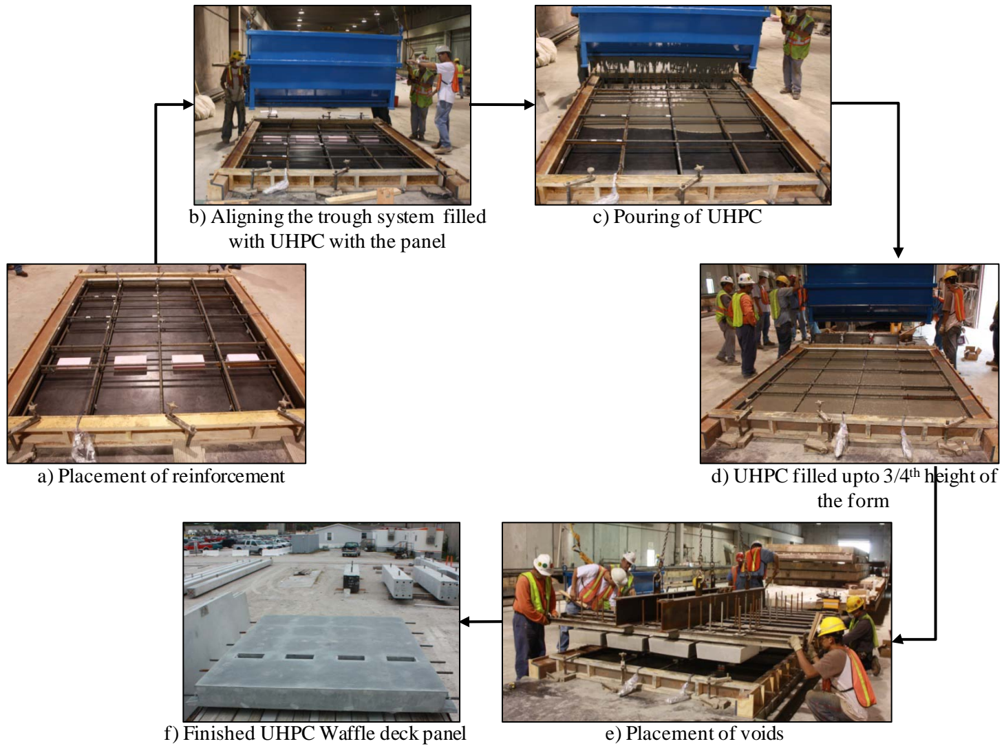
Figure 6 Construction sequence of the UHPC Waffle deck panel at the precast plant.
