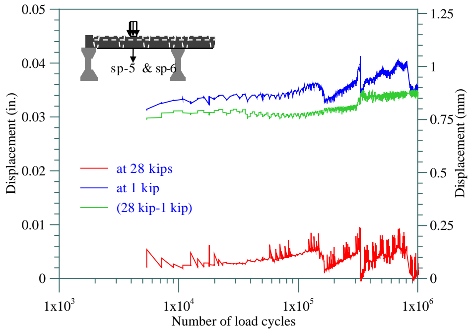
Figure 24 The variation of the peak displacement at the center of the joint during the joint fatigue test.
