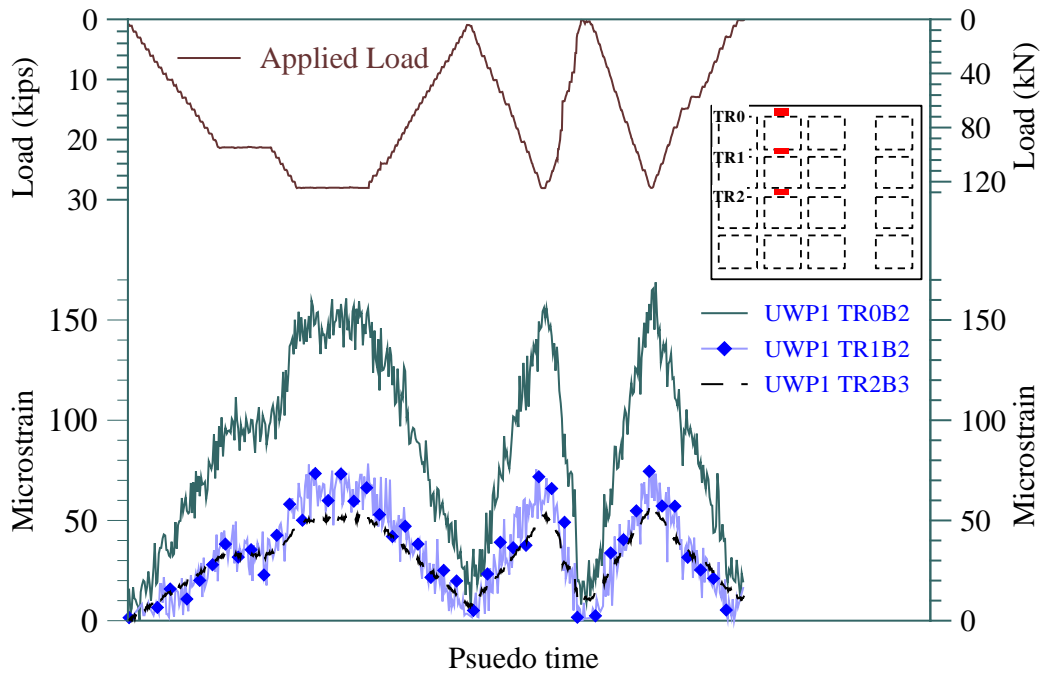
Figure 22 Measured strains at the center of the panel across the transverse ribs of UWP1 at service load.
