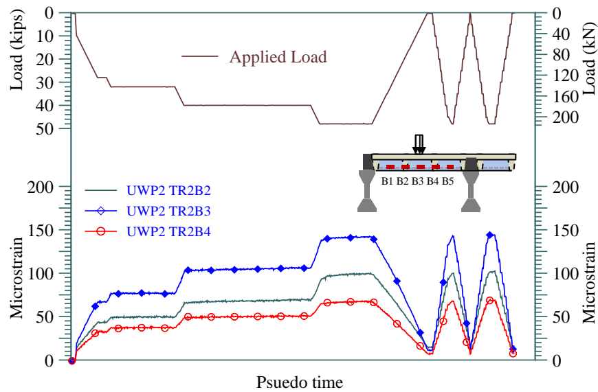
Figure 29 Measured strains in the bottom reinforcement of transverse rib TR2 along the length of Panel UWP2 at the ultimate load.
