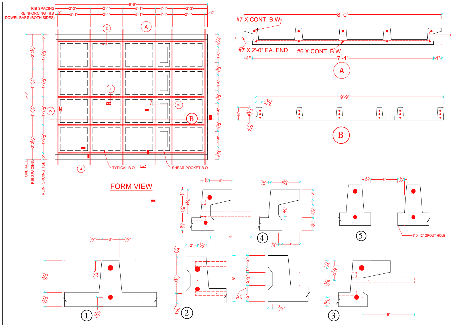
Figure 5 Reinforcement details of the UHPC waffle deck test panels.
