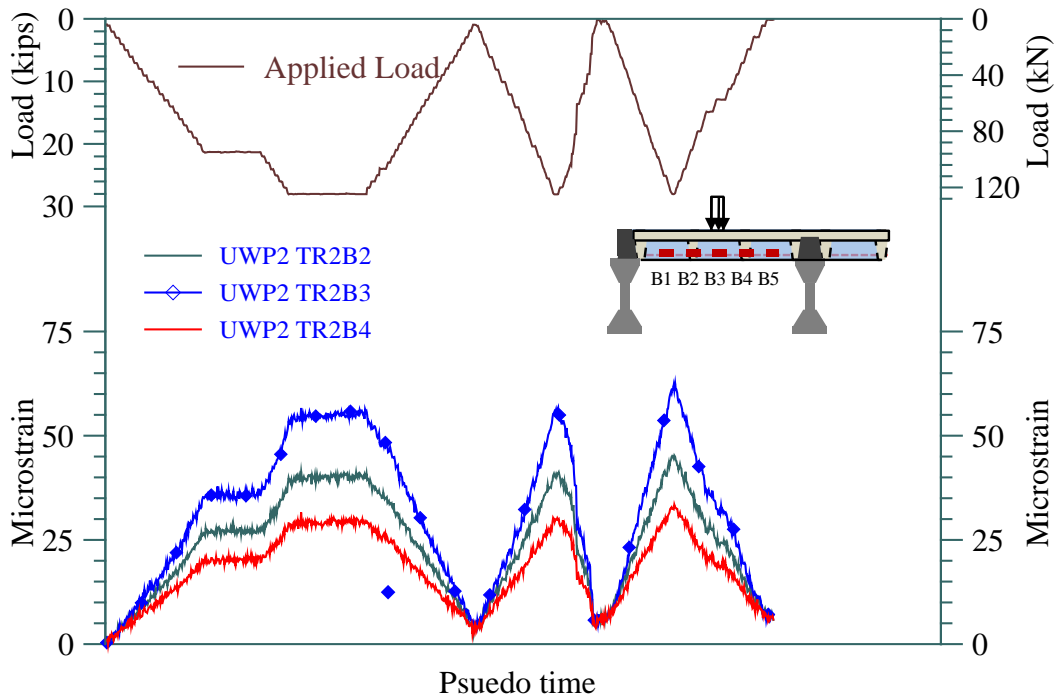
Figure 20 Measured strains in the bottom reinforcement of the transverse rib (TR2) along the length of panel UWP2 at service load.
