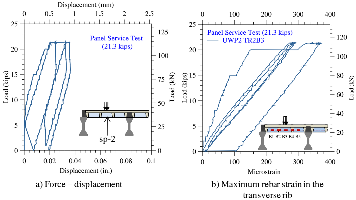
Figure 13 Measured force-displacement response and peak rebar strain from gauge B3 at the center of the transverse rib TR2 of panel UWP2.
