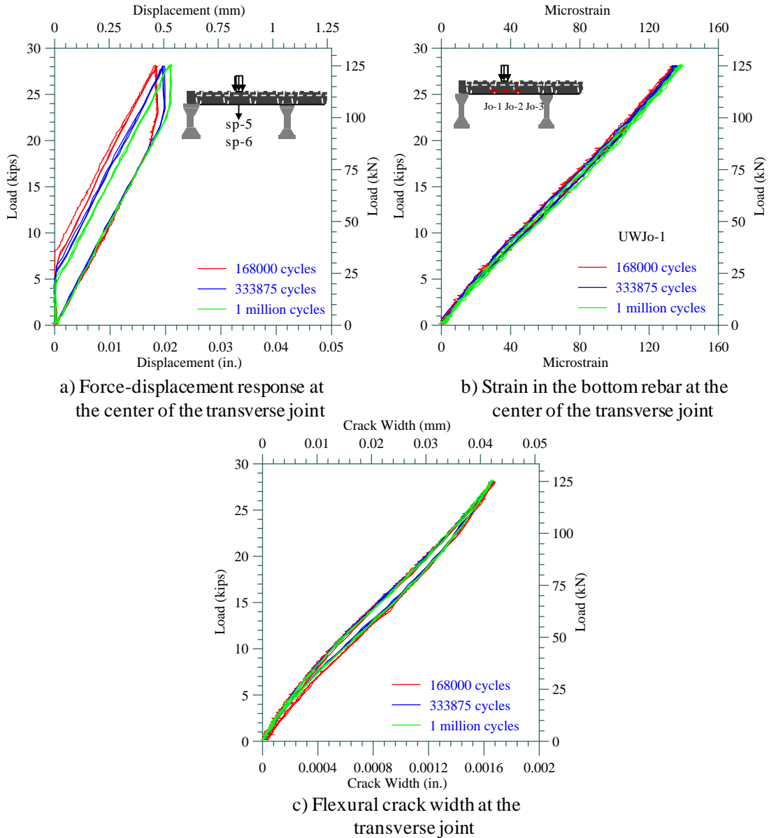
Figure 27 Measured responses of the waffle deck system from the static service load tests conducted during the joint fatigue test.
