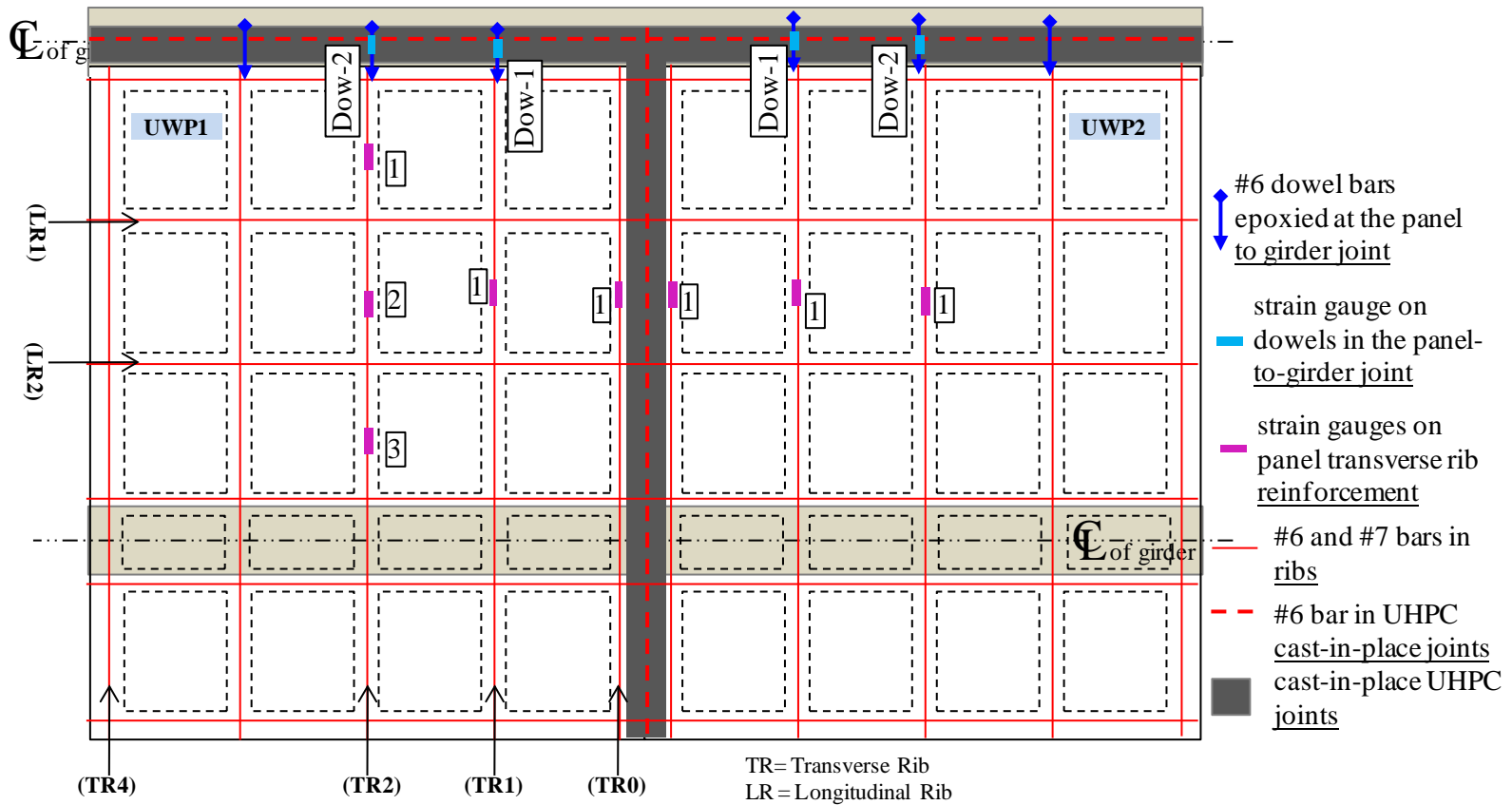
Figure 12 Location of strain gauges on the top deck reinforcing bars and dowel bars.
