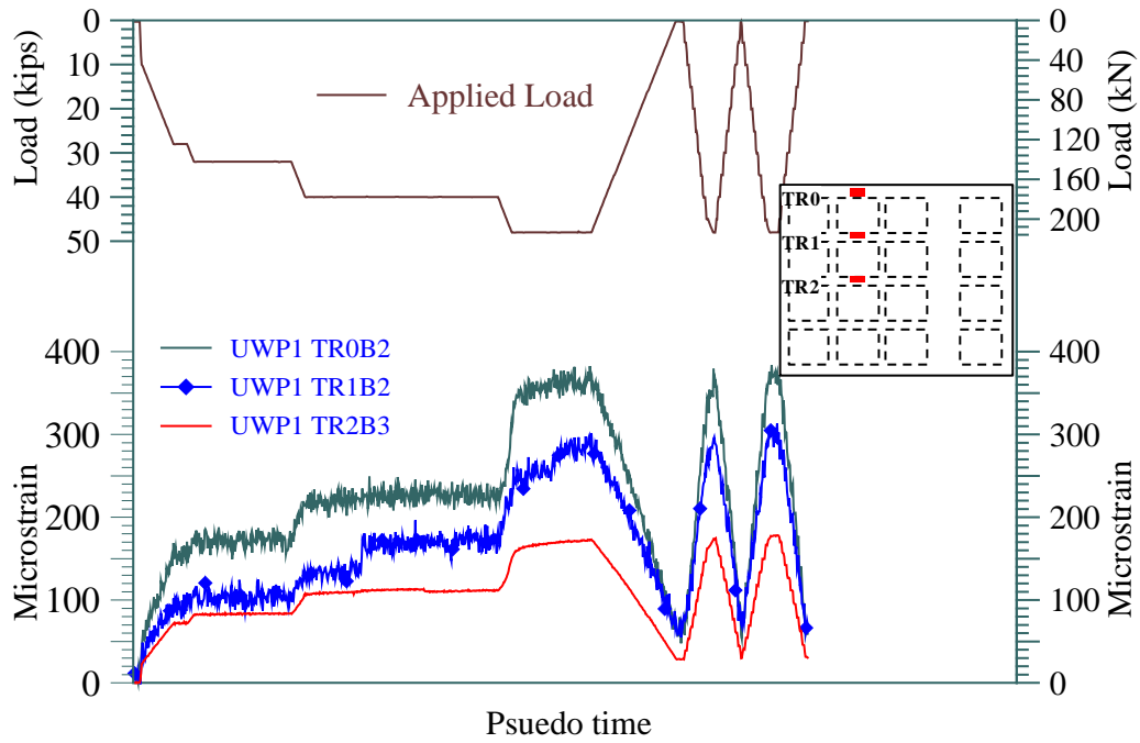
Figure 31 Measured strains at the center of the panel across the transverse ribs of panel UWP1 at joint ultimate load.
