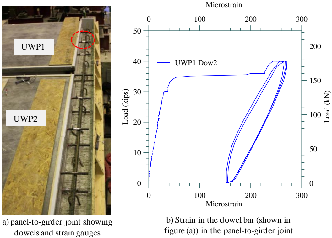
Figure 43 Strain variations in a dowel bar placed in the panel-to-girder joint during the panel ultimate load test.
