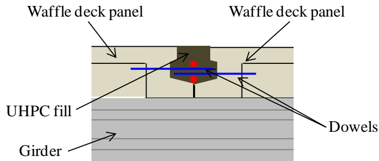
Figure 4 Connection details between the waffle deck panels
