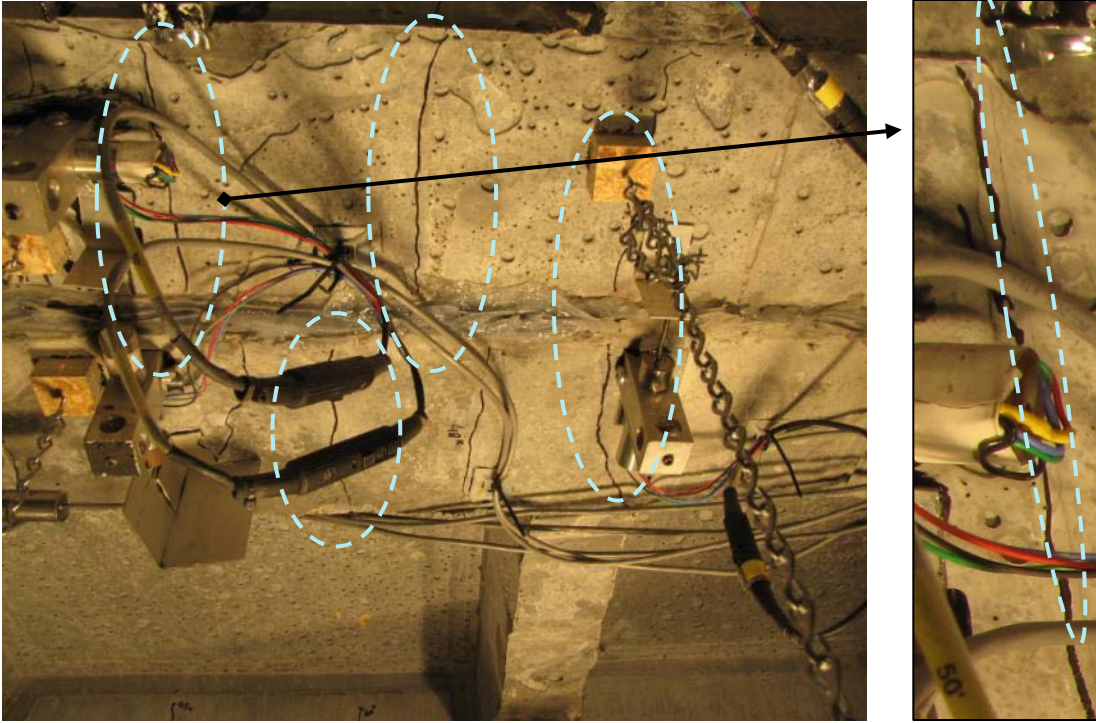
Figure 32 Hairline cracks formed at the center of underside of the transverse joint at the ultimate load of 48 kips.
