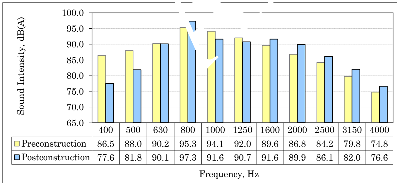
Figure 52. Chart. Mean A-weighted SI frequency spectra of the I-84 WB bridge before and after construction.
