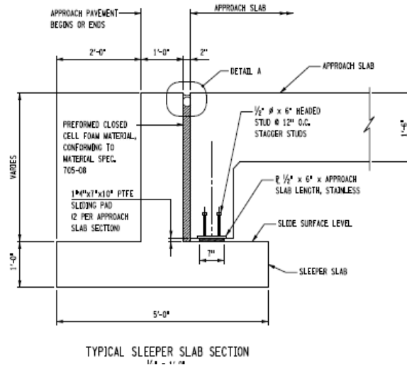
Figure 9. Diagram. Typical precast sleeper slab section.
