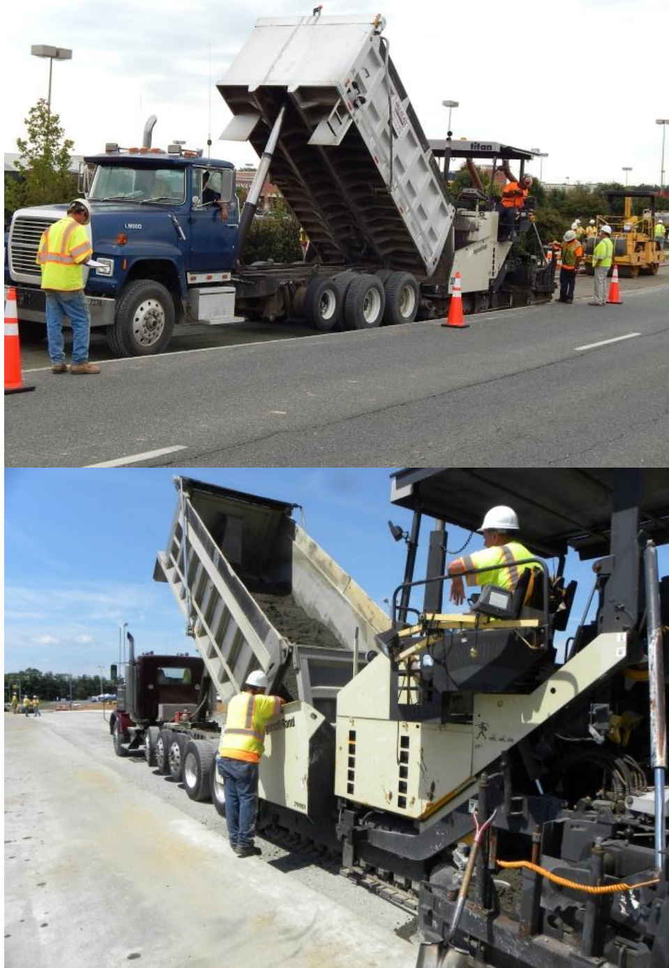
Figure 9. Photos. RCC placement.
