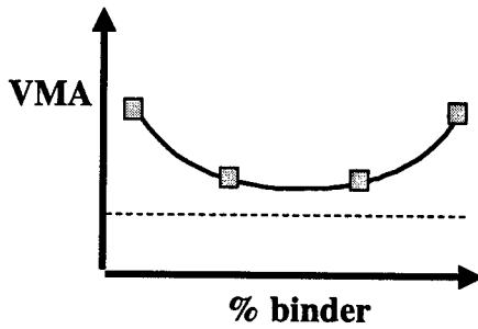
Voids in the Mineral Aggregate
