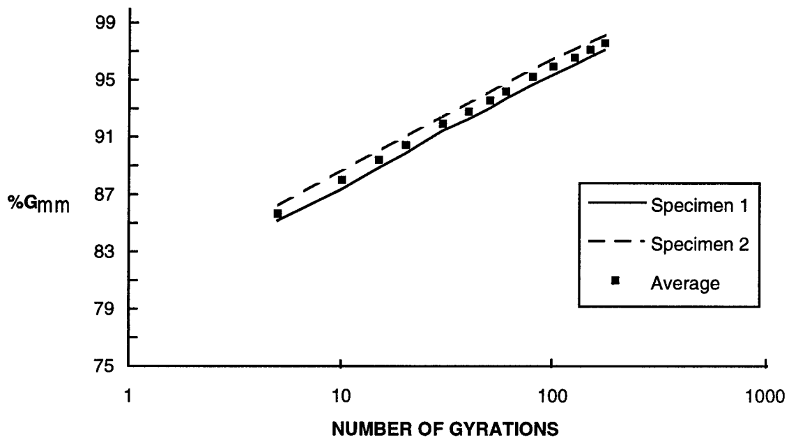
IH-43, 19.0 mm Nominal, 4.4% AC, Trial Blend 1
