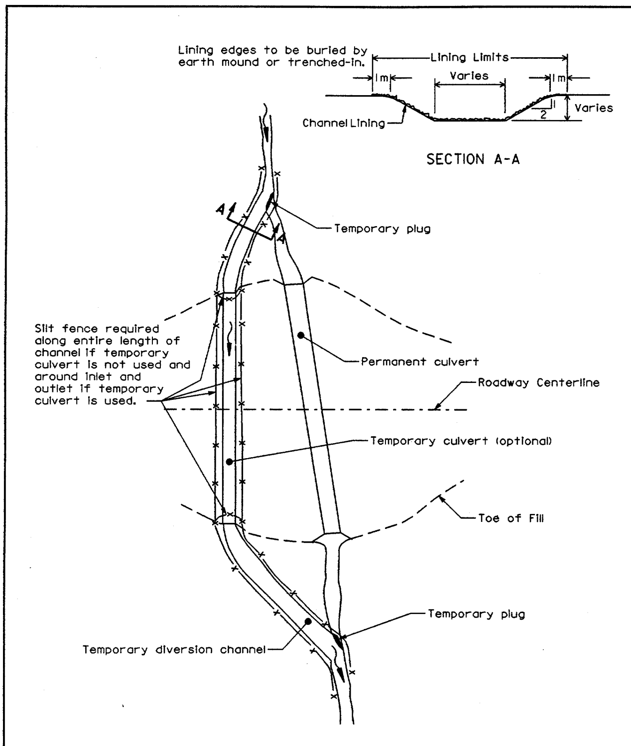
Figure 5.5 Diversion for Culvert Installation
