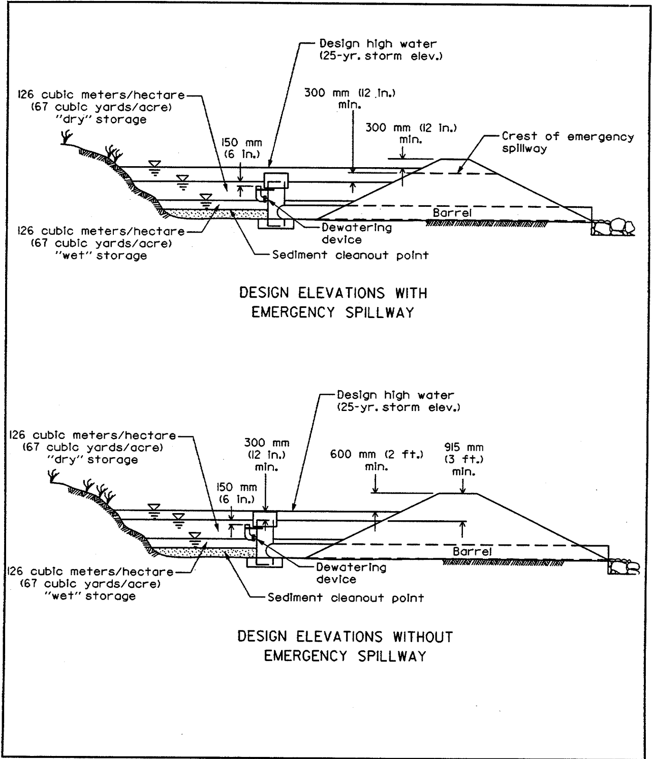
Figure 6.4 Sediment Basin Design Elevations
