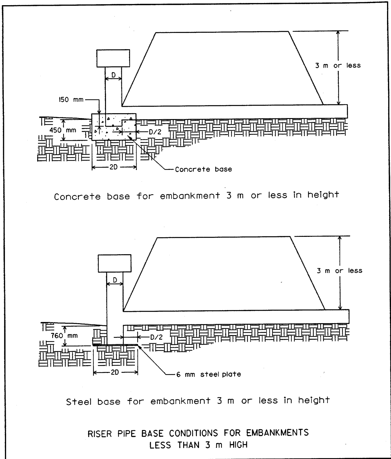
Figure 6.9 Riser Pipe Anchors
