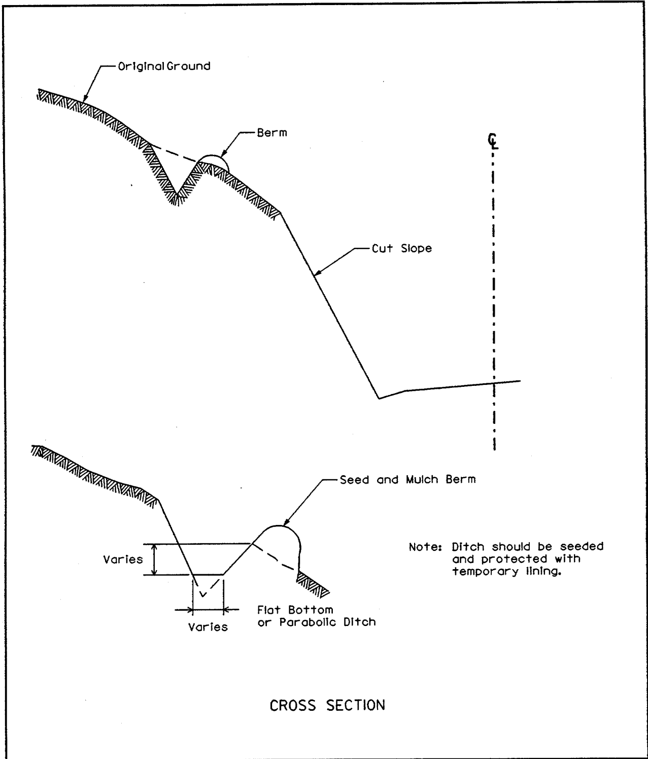
Figure 5.3 Diversion Channel and Berm
