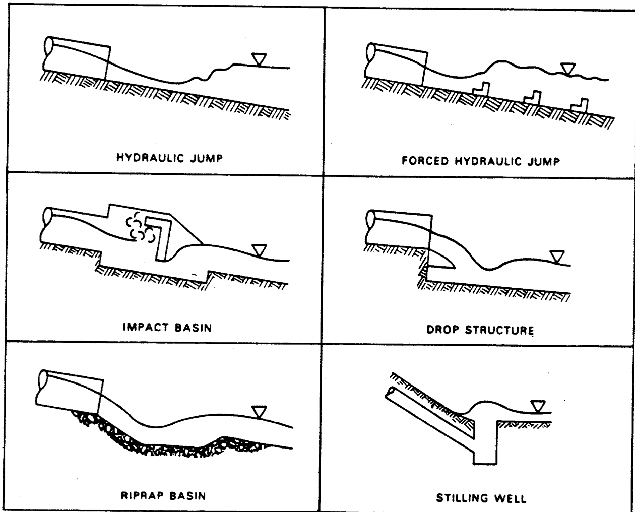
Figure 5.9 Types of Energy Dissipators
