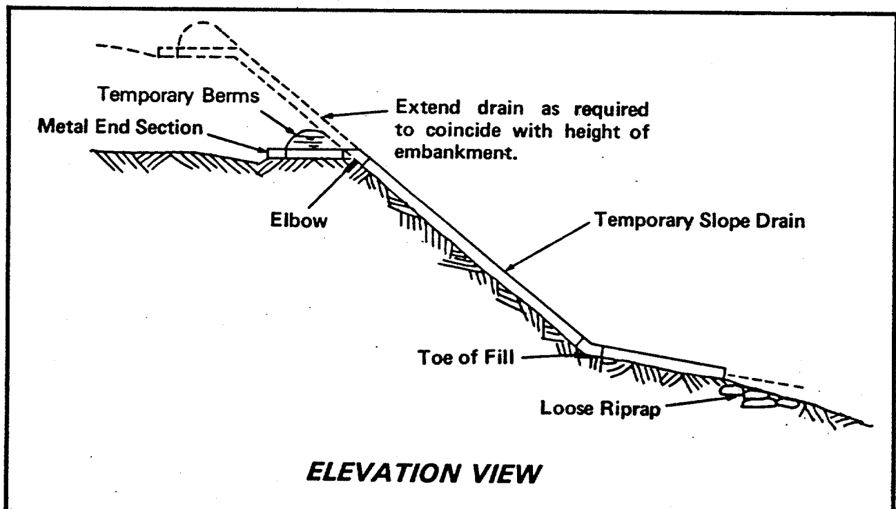
Figure 5.6 Temporary Slope Drain
