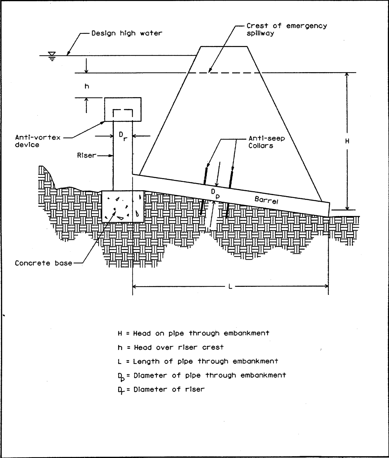
Figure 6.5 Principal Spillway Design
