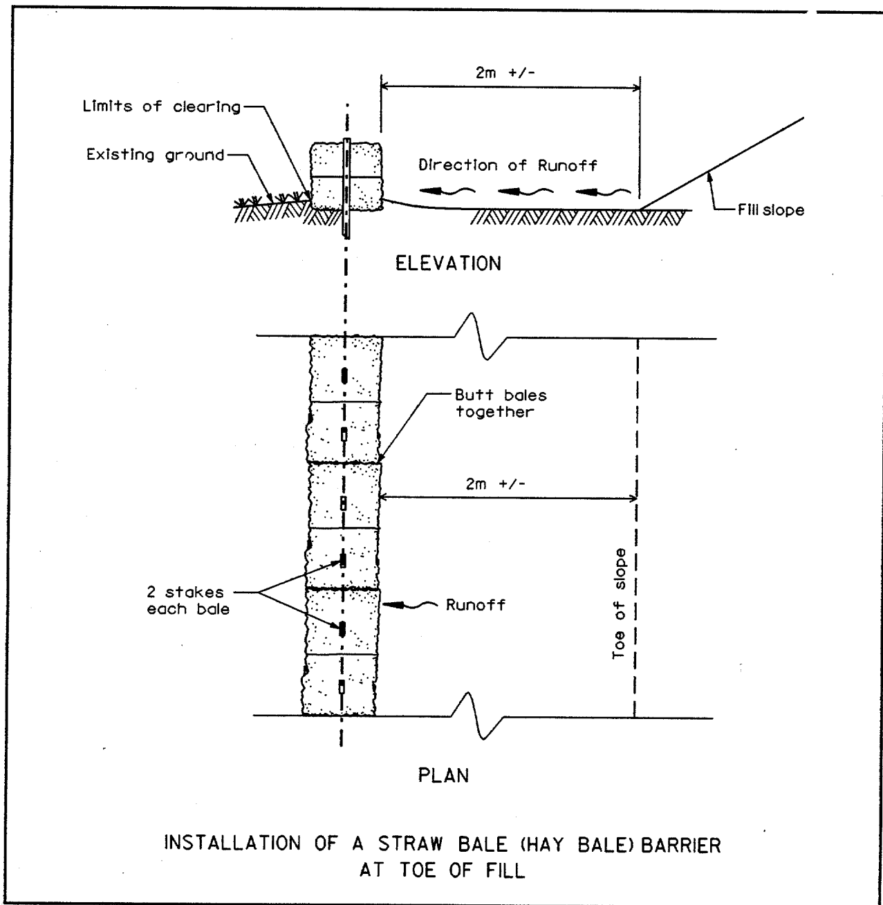
Figure 5.13 Straw Bale as a Perimeter Control
