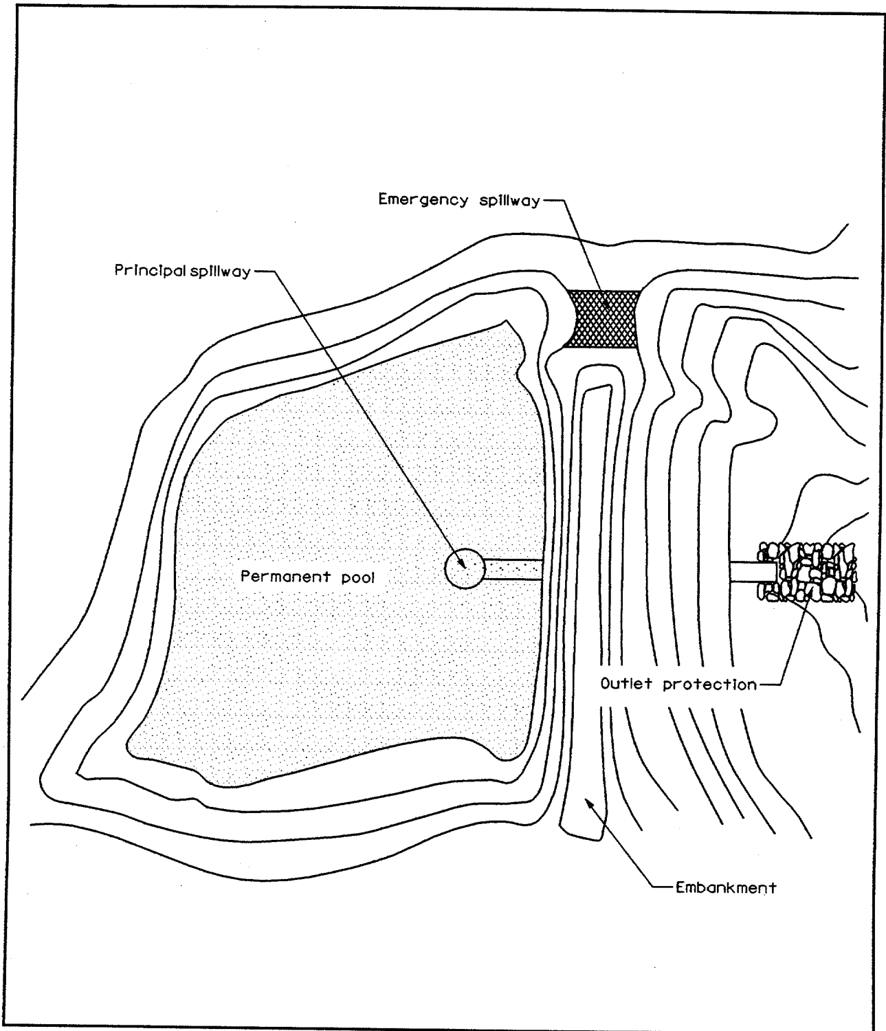
Figure 6.3 Sediment Basin
