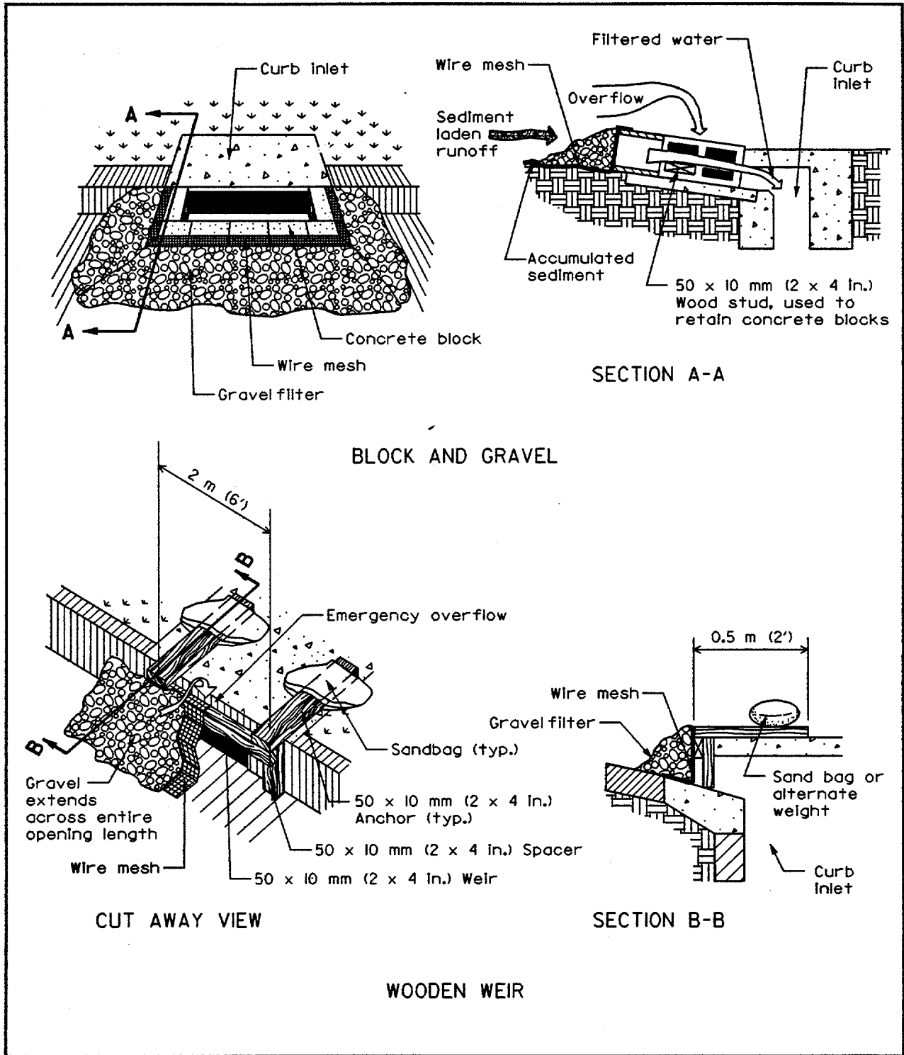
Figure 5.18 Curb Opening Drop Inlet Protection
