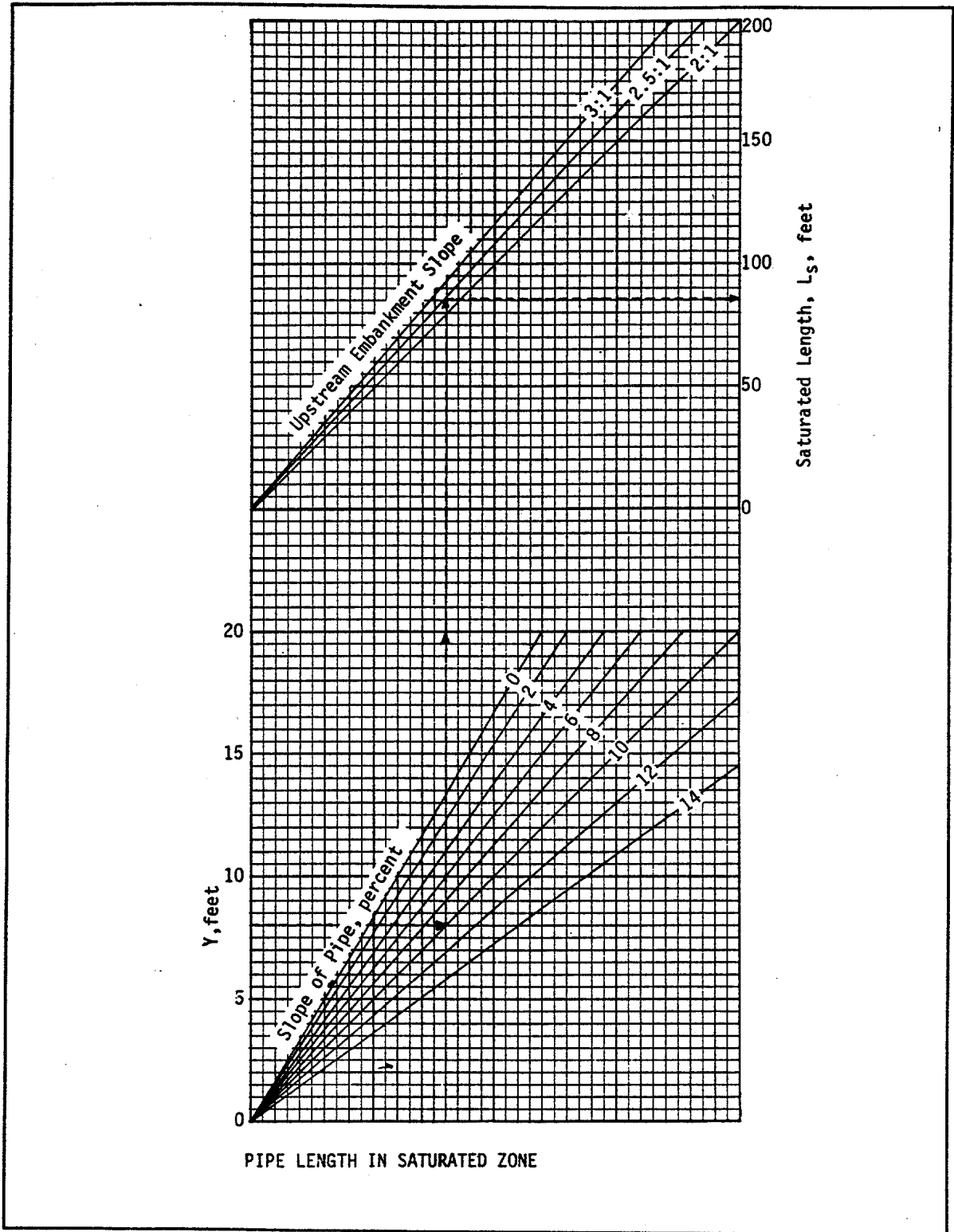
Figure 6.11 Pipe Length in Saturated Zone
