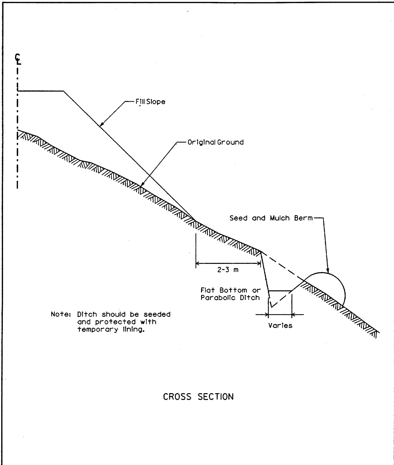
Figure 5.4 Diversion Channel and Berm
