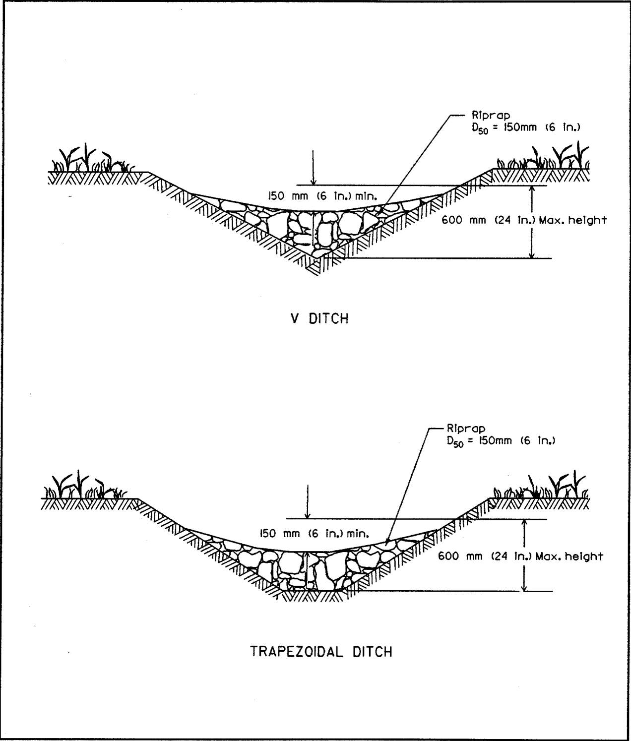
Figure 5.1 Check Dam Cross Section
