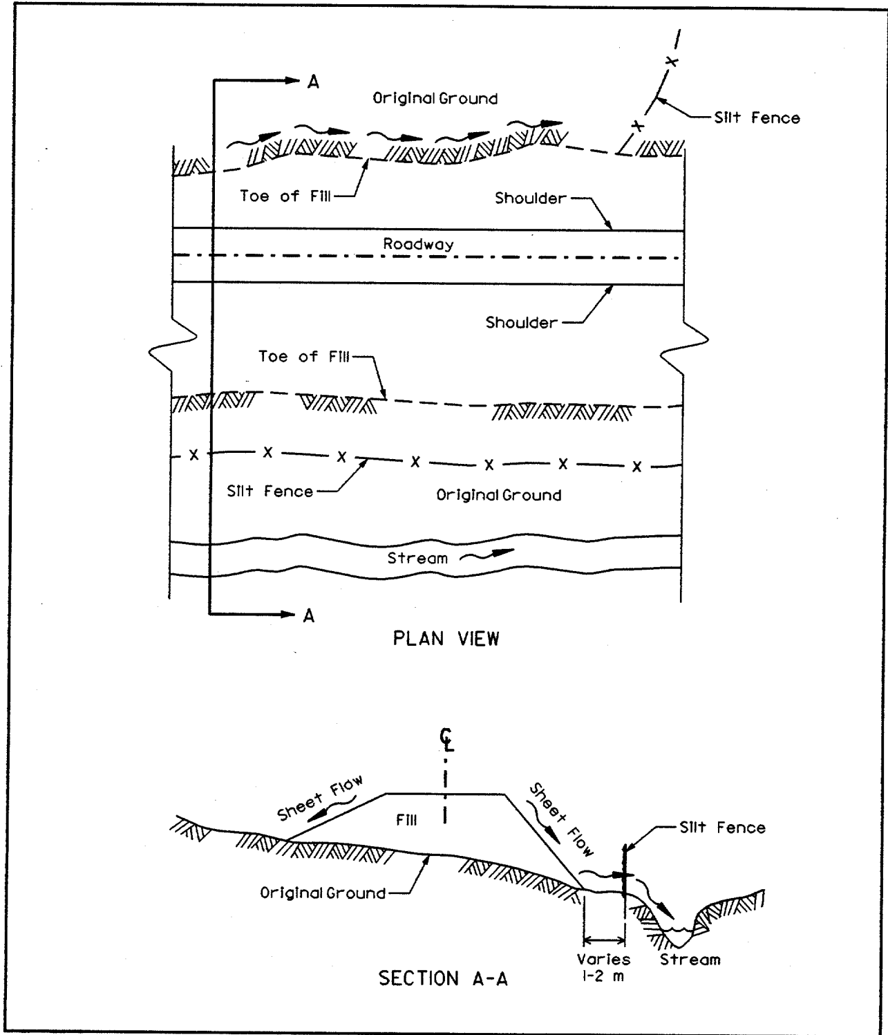
Figure 5.12 Silt Fence Protecting Waterway
