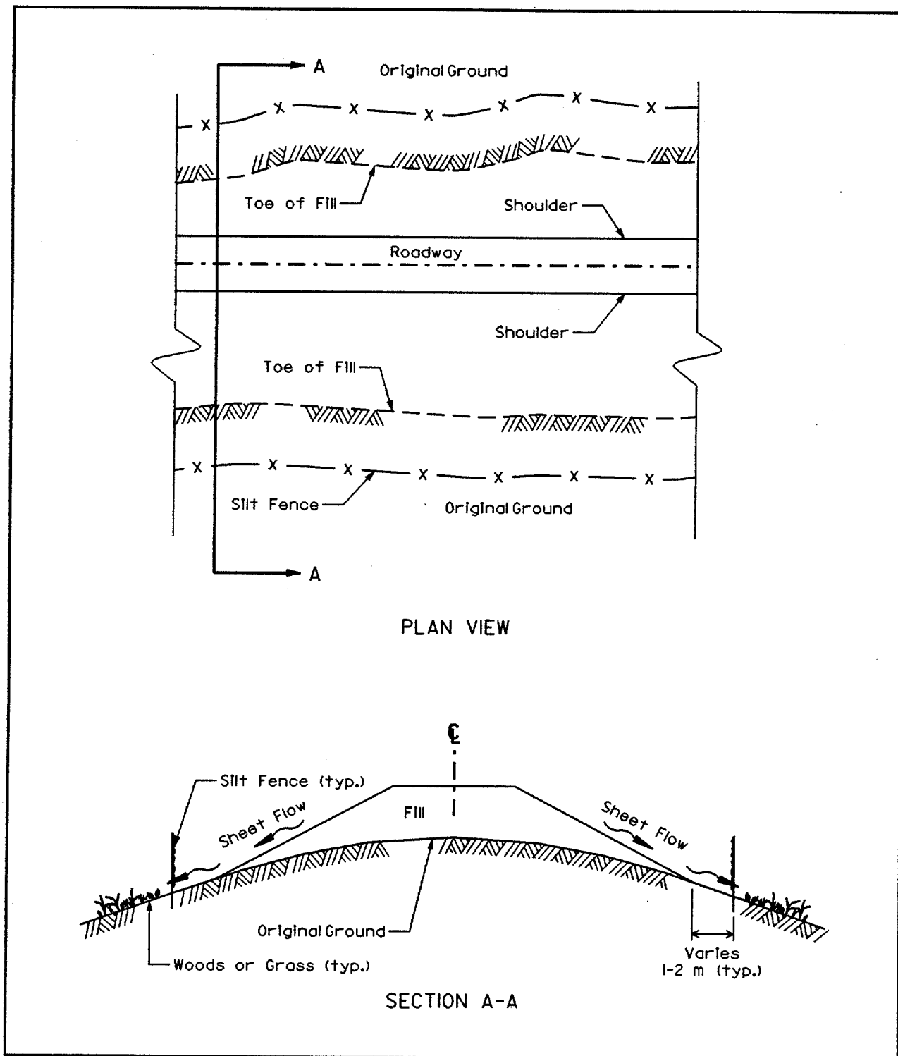
Figure 5.11 Silt Fence as a Perimeter Control
