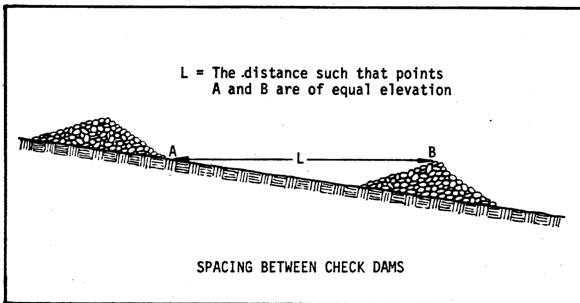
Figure 5.2 Spacing Between Check Dams
