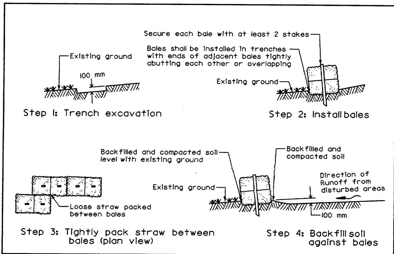
Figure 5.14 Straw Bale Installation
