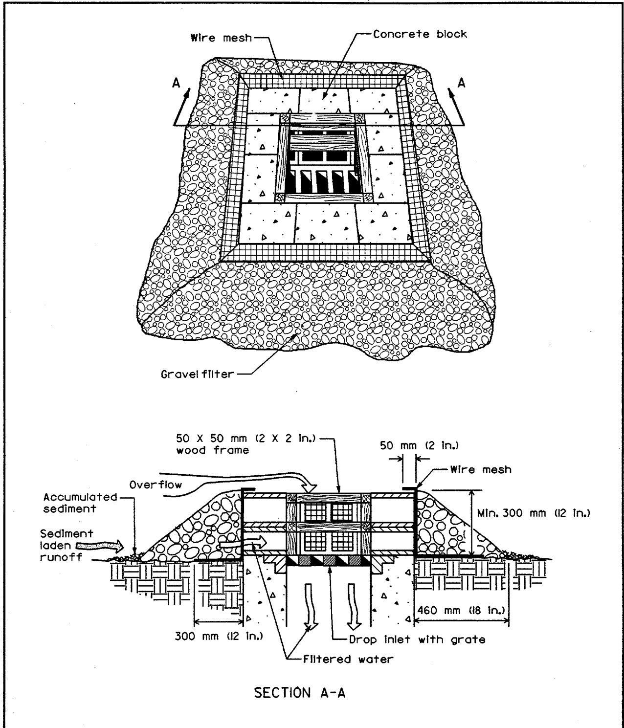
Figure 5.16 Block and Gravel Drop Inlet Protection
