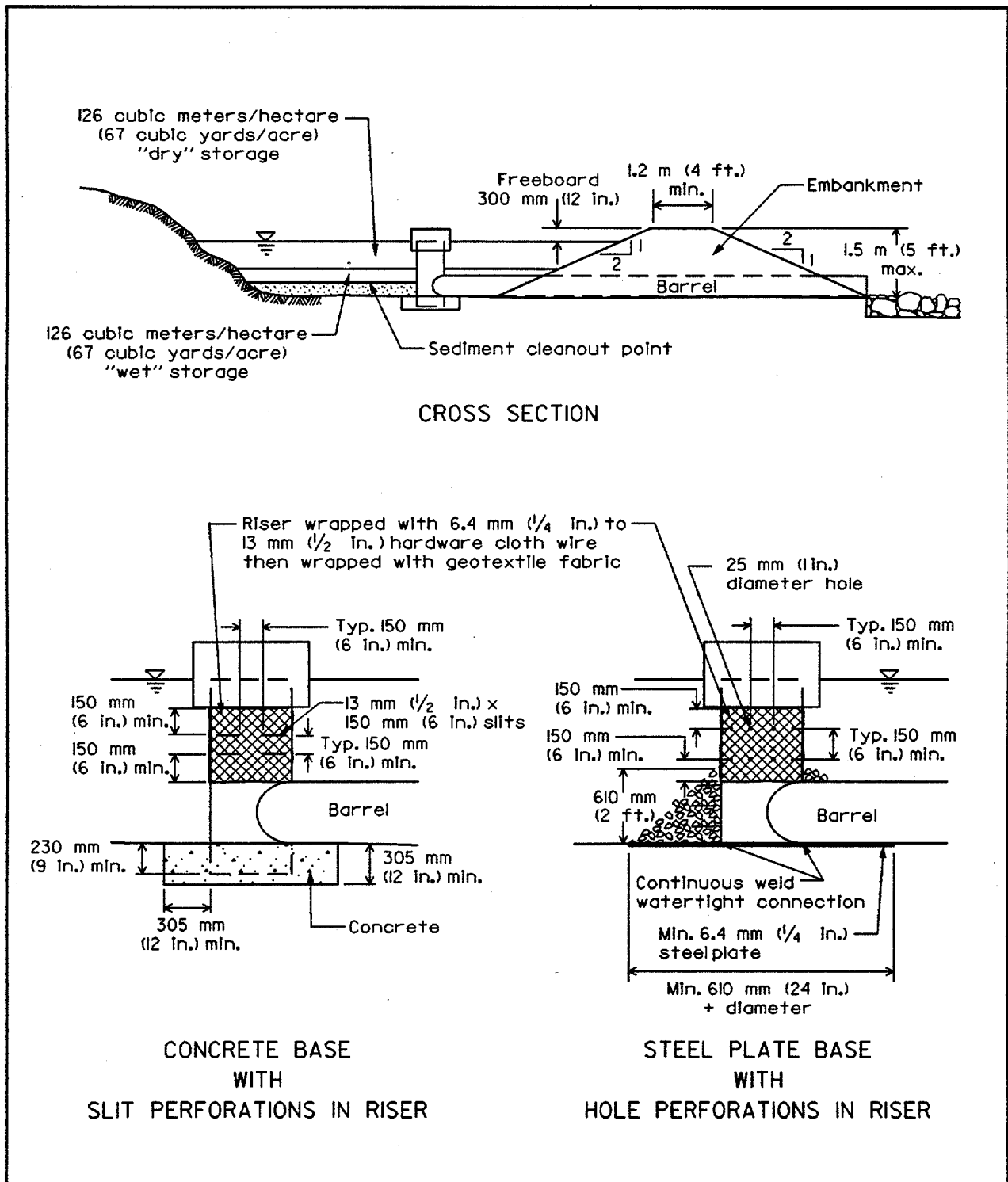
Figure 6.2 Pipe Outlet Sediment Trap
