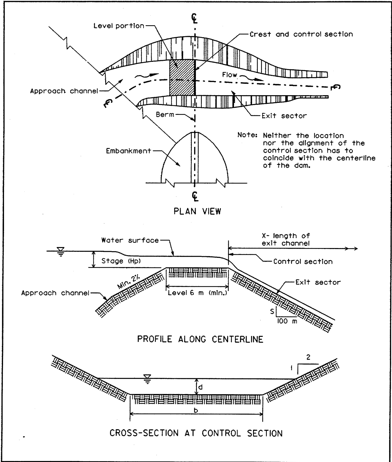
Figure 6.7 Emergency Spillway
