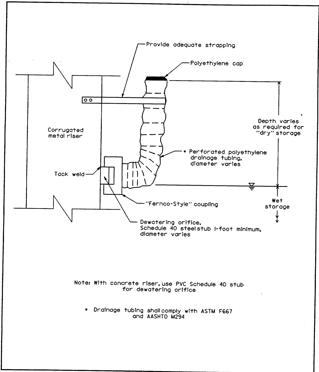
Figure 6.6 Dewatering Device
