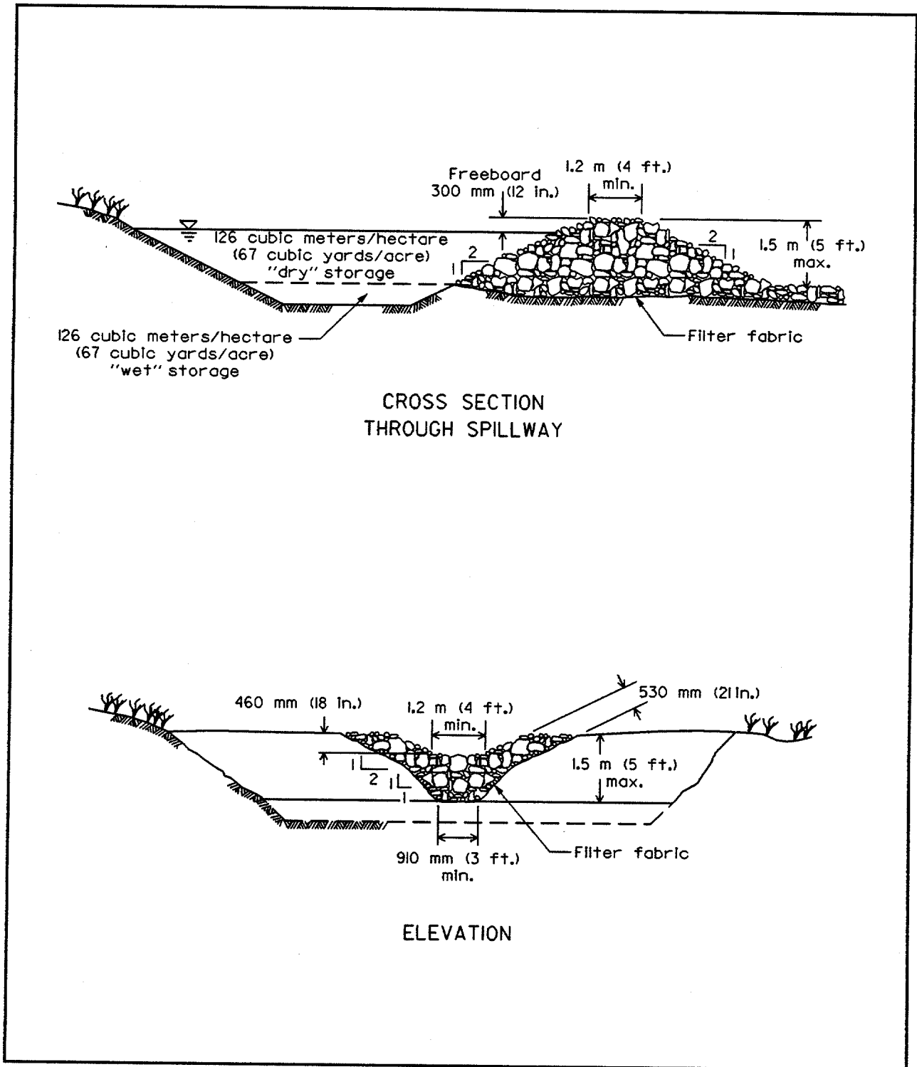
Figure 6.1 Stone Outlet Sediment Trap
