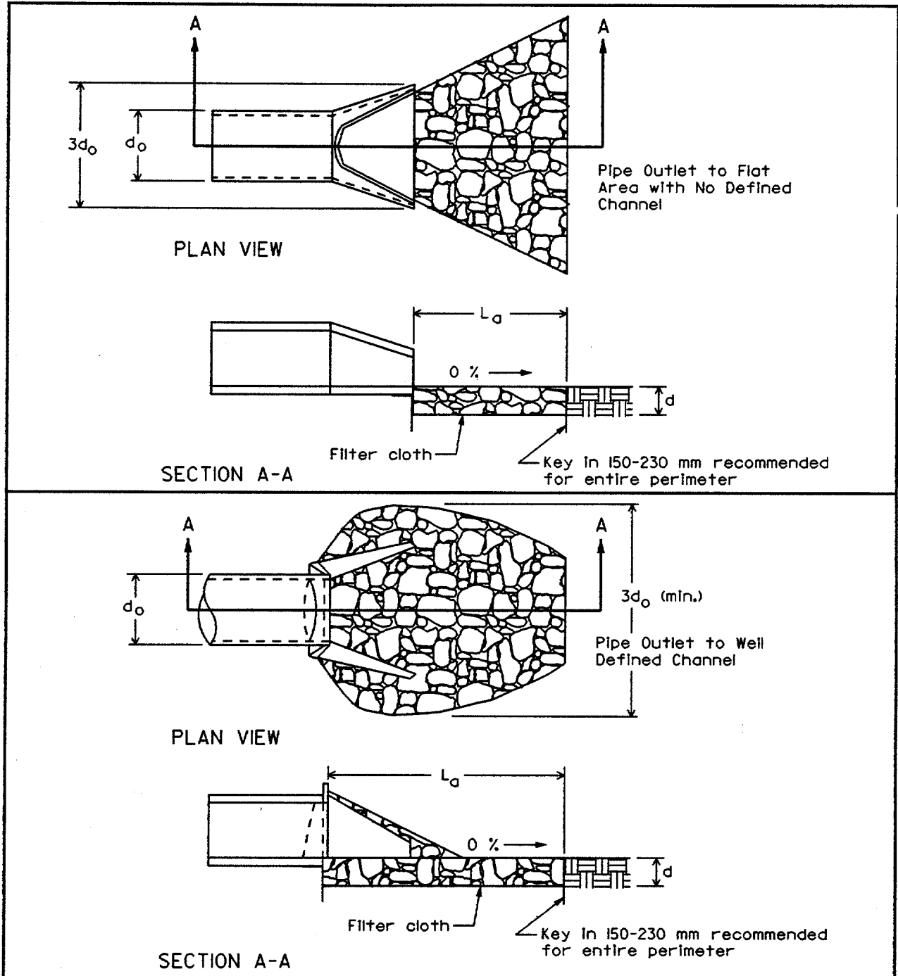
Figure 5.7 Outlet Protection
