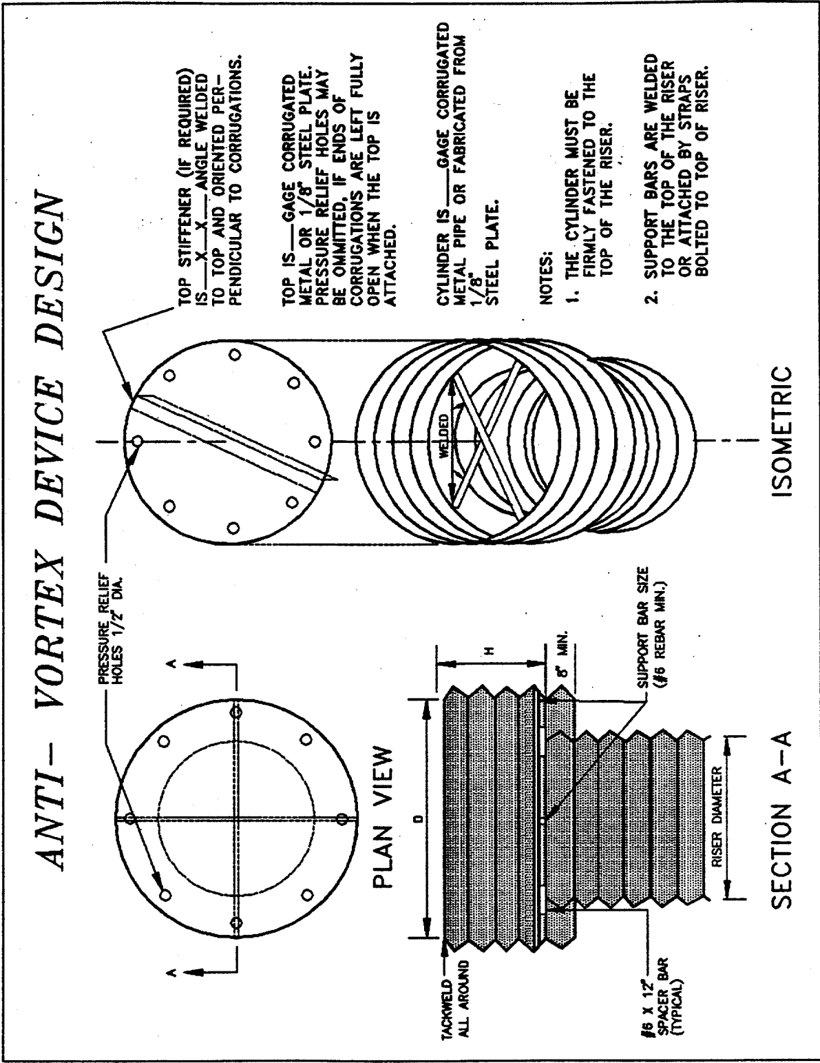
Figure 6.13 Anti-Vortex Device Details
