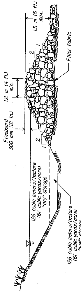
ELEVATION SEDIMENT TRAP (TYPE A) RIPRAP OUTLET
