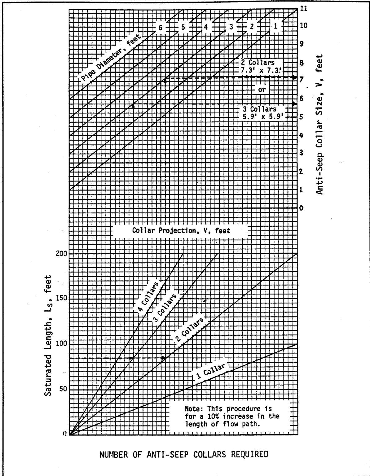
Figure 6.12 Anti-seep Collar Design
