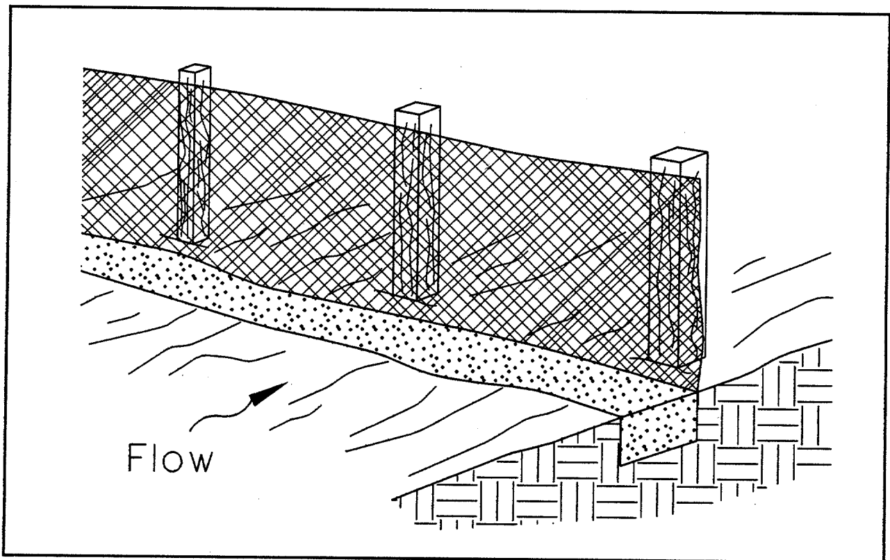
Figure 5.10 Silt Fence
