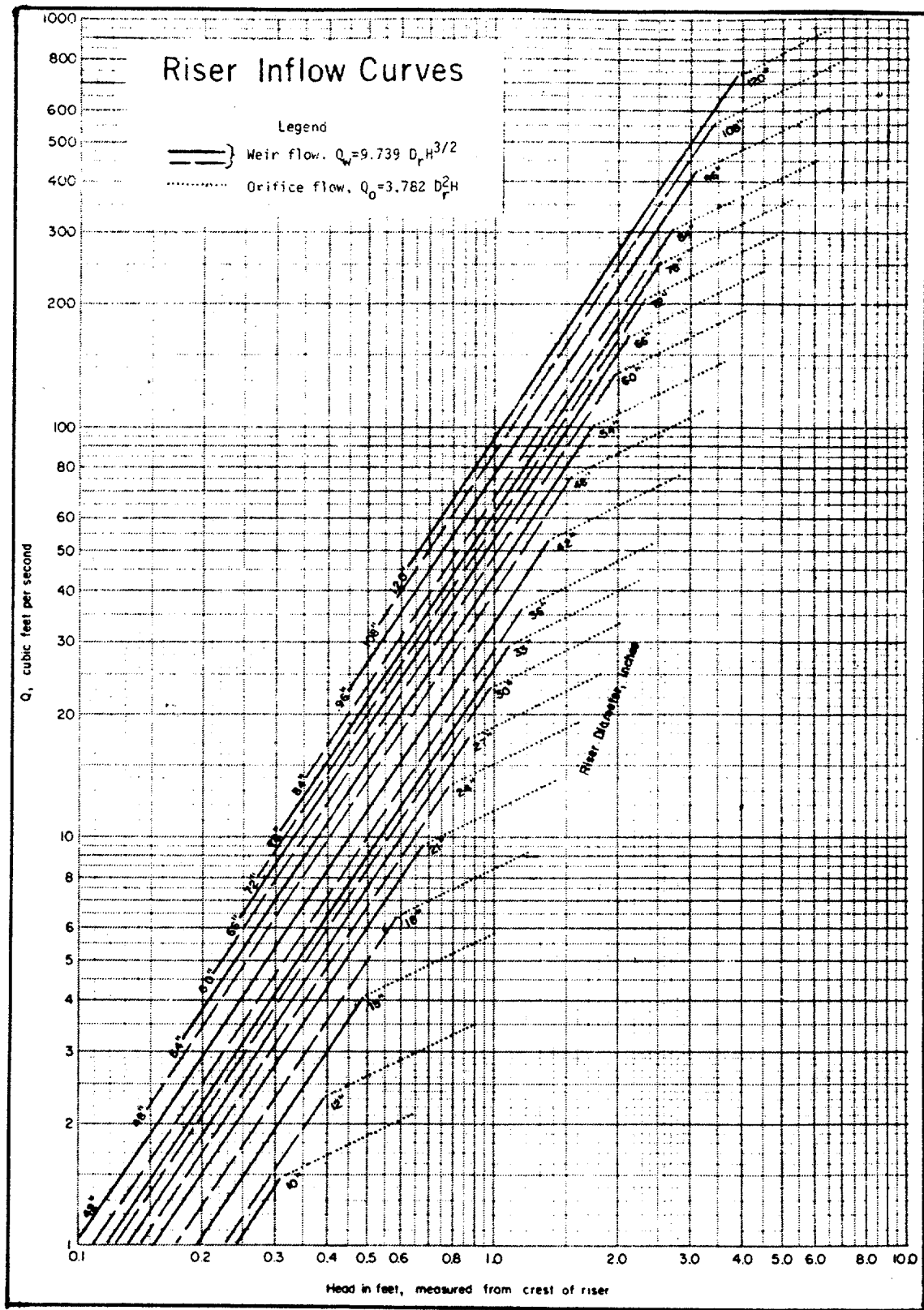
Figure 6.8 Riser Inflow Curves
