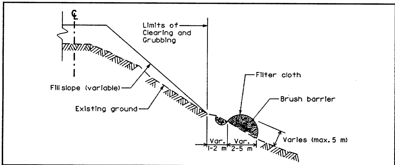
Figure 5.15 Brush Barrier Application
