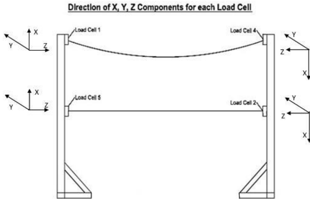
Figure 30: Direction of x , y , z components for each loadcell (direction of each axis shown)
