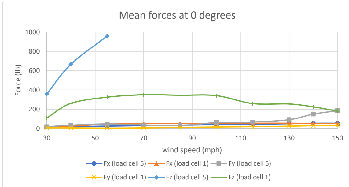
Figure 20: Mean forces on loadcells 1 (catenary wire) and 5 (messenger wire) at 0-degree wind direction
