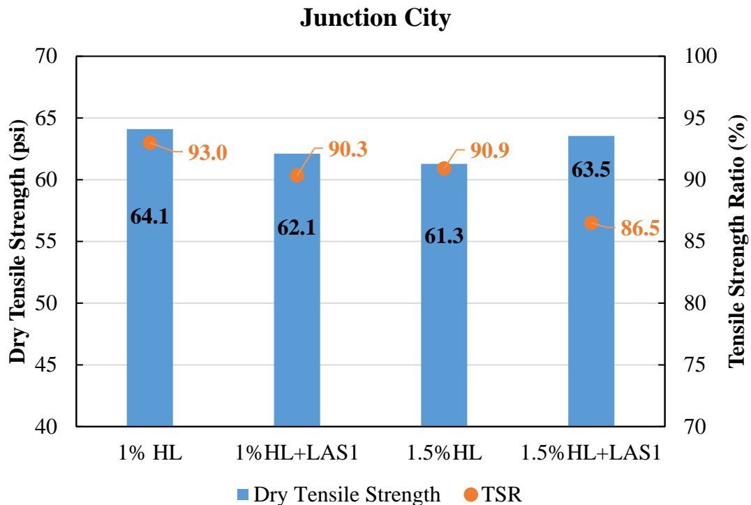
Figure 33. Tensile Strength Ratio Test Results for Junction City FC-5 Asphalt Mixtures
