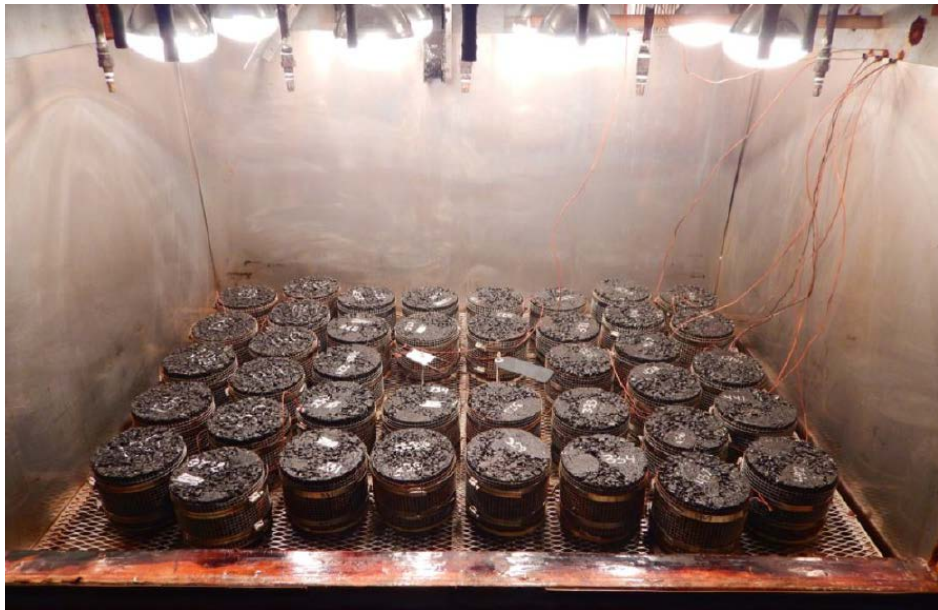
Figure 28. FC-5 Specimens in Asphalt Pavement Weathering System
