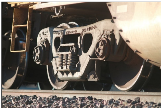
Figure 1. Freight car side frame and wheels
