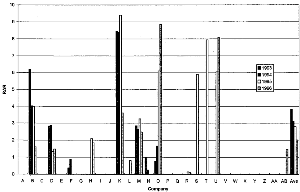
Figure 15 Road Accident Rate (Accidents per Million Kilometres)
