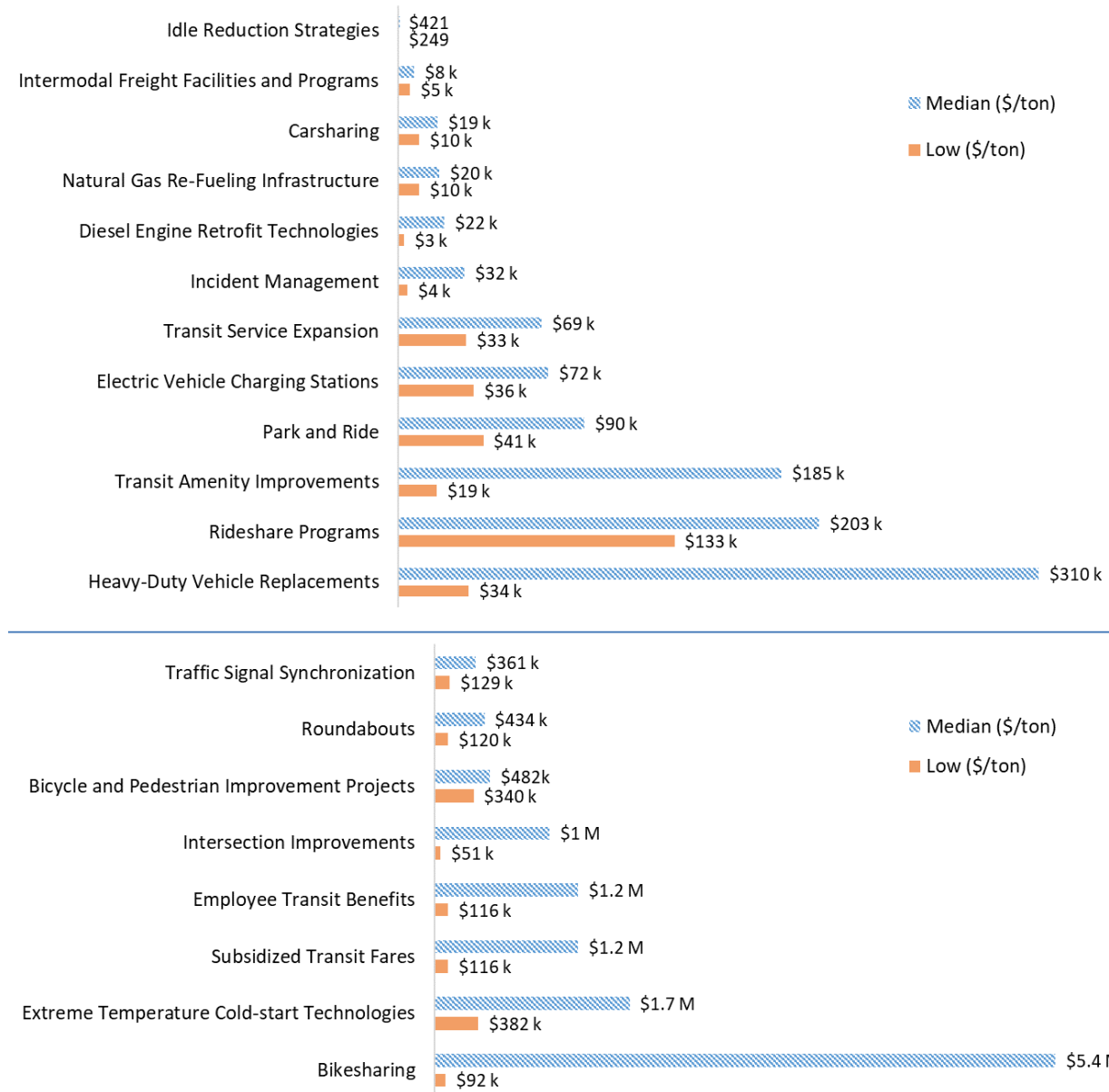
Figure 2. Median cost-effectiveness (dollars per ton reduced) for NOx
