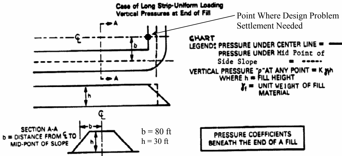
Figure A.6-4. Pressure distribution chart used to estimate the change in pressure at depths below the end of an embankment fill.
