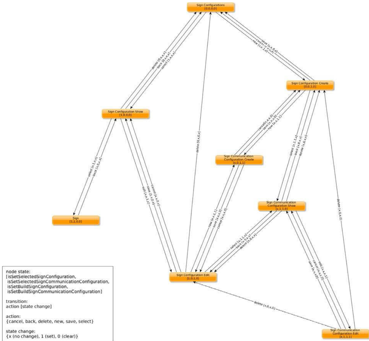
Figure 3.13 DMS configuration state architecture and transitions
