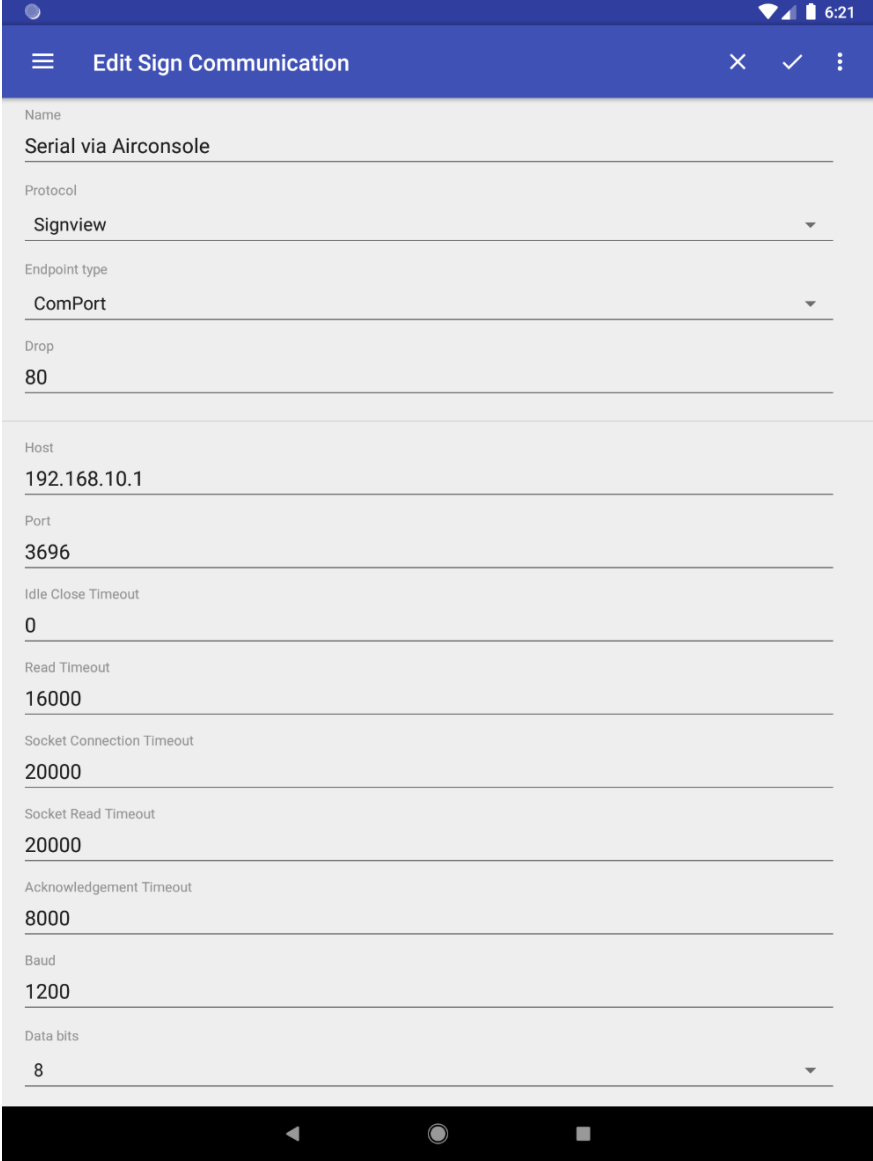
Figure 3.35: DMS edit sign communication
