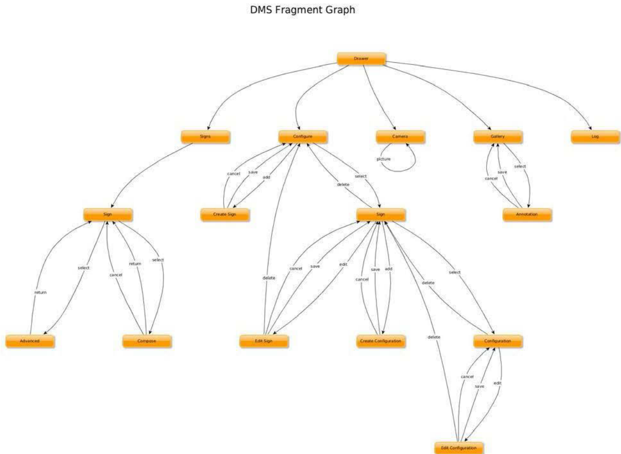
Figure 3.1: DMS fragment graph
