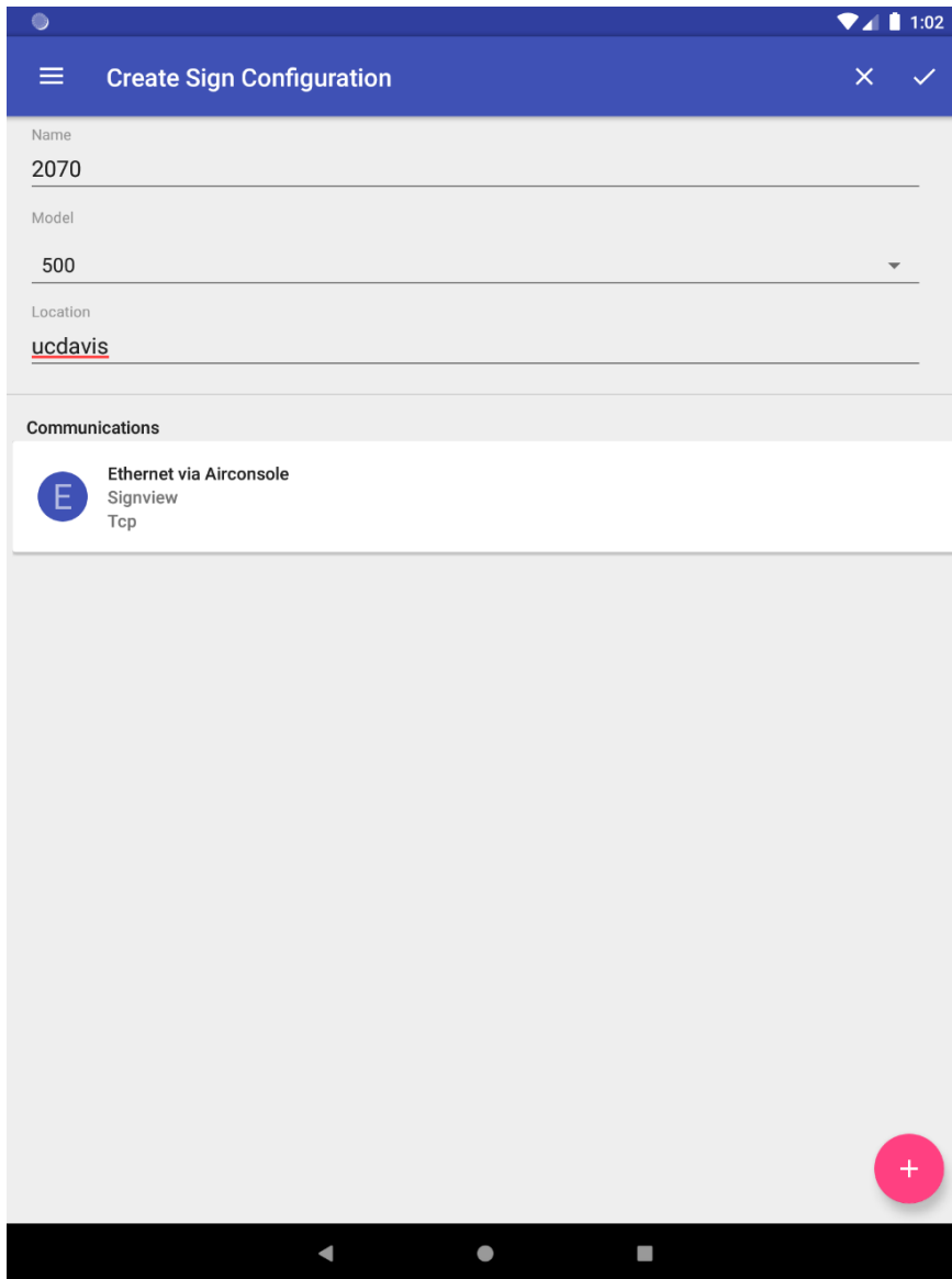
Figure 3.44: DMS 2070 sign configuration with a communications configuration
