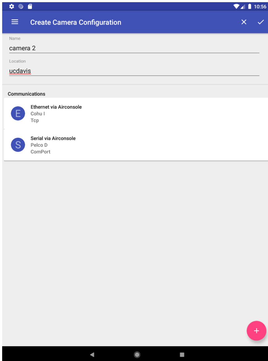
Figure 4.21: CCTV camera configuration with multiple communication configurations
