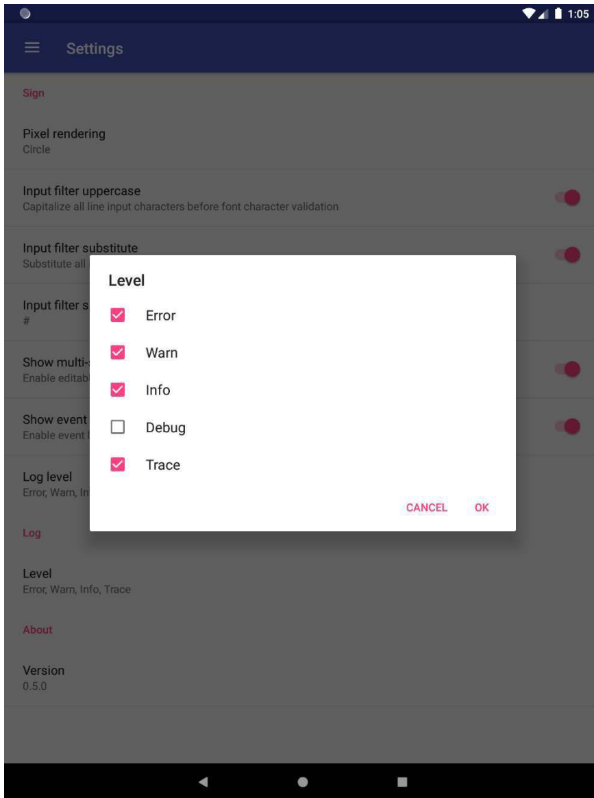
Figure 3.66: DMS settings event log level configuration
