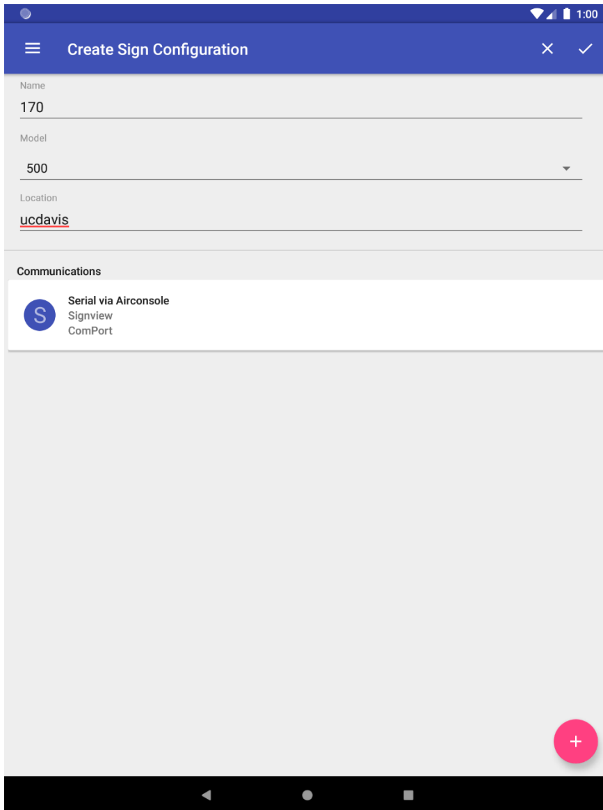
Figure 3.32: DMS sign configuration with a serial communication configuration
