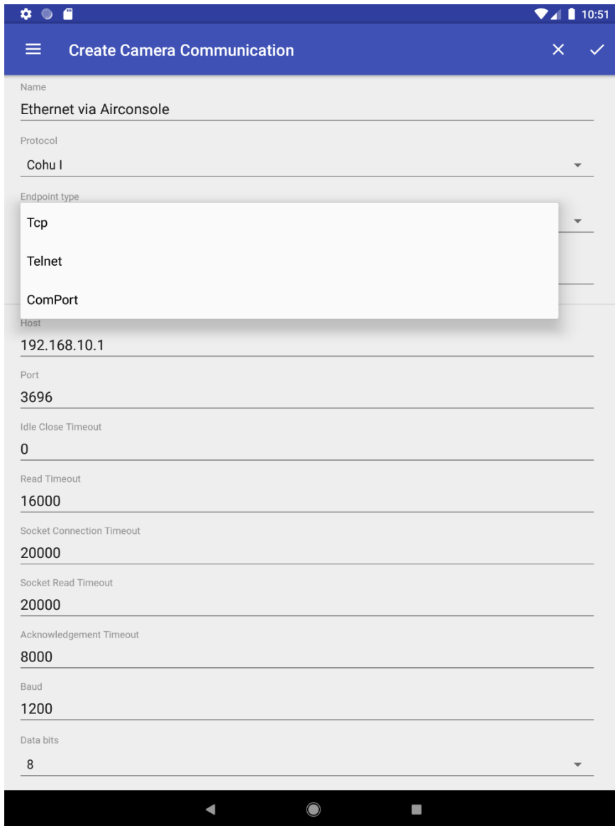
Figure 4.13: CCTV create camera communication endpoint type options
