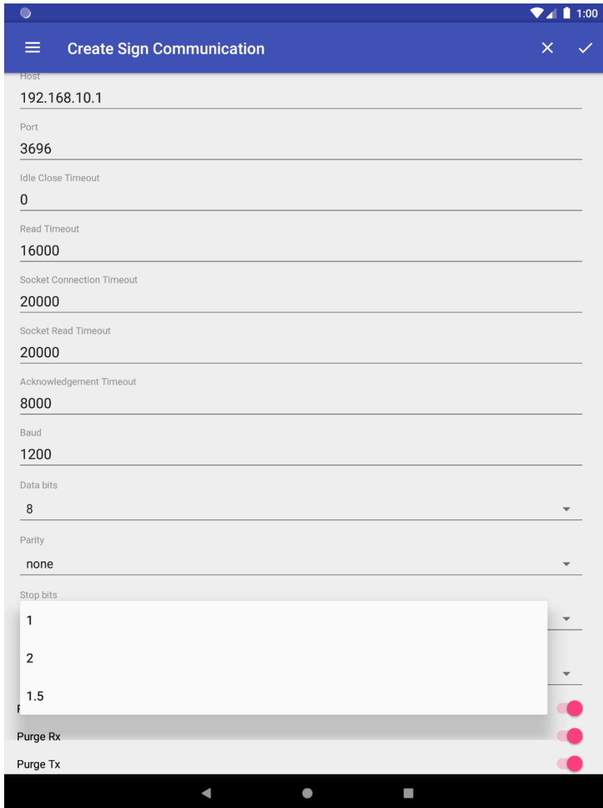
Figure 3.30: DMS create sign communication stop bits options
