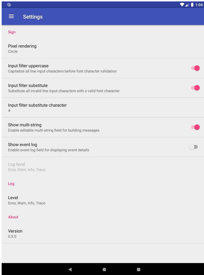
Figure 3.63: DMS settings with show multi-string enabled
