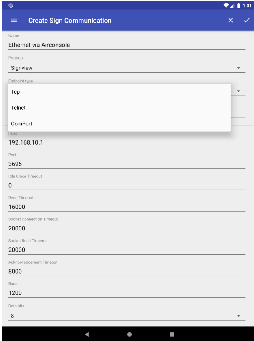
Figure 3.42: DMS create sign communication endpoint type options
