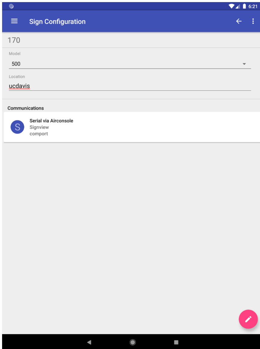
Figure 3.37: DMS sign configuration with option to edit
