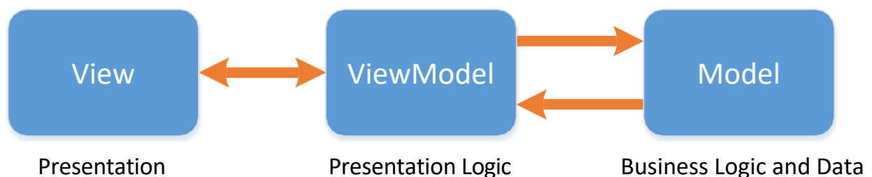
Figure 2.14: Model-View-ViewModel (MVVM) software pattern
