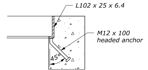
FRAME ANCHOR DETAIL
