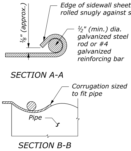
CONNECTOR DETAILS FOR METAL ROUND PIPES 15" THRU 24" TYPE #1 FOR METAL ROUND PIPES 30" AND LARGER. FOR PIPE ARCHES 21" X 15" AND LARGER TYPE #2 FOR ALL SIZES OF CONCRETE ROUND OR PIPE ARCHES TYPE #3
