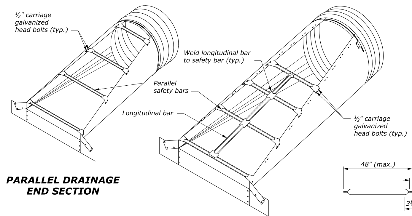
LONGITUDINAL DRAINAGE BAR PARALLEL BARS SAFETY BAR DETAILS
