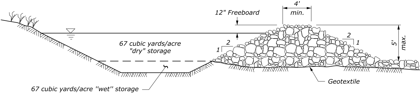
CROSS SECTION THROUGH SPILLWAY
