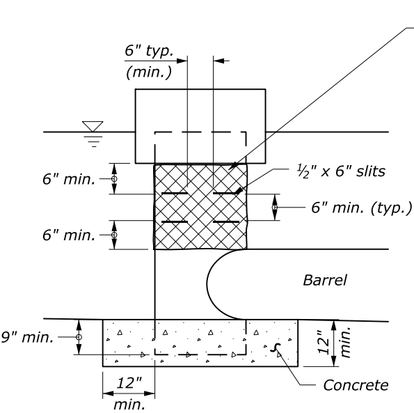
CONCRETE BASE WITH SLIT PERFORATIONS IN RISER
