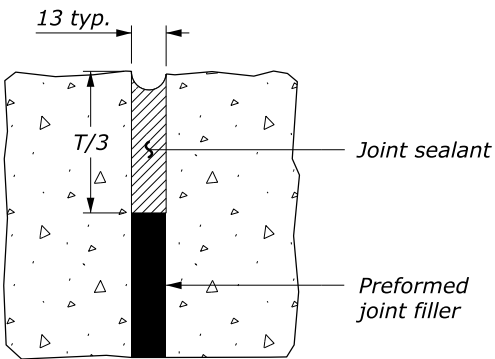
ISOLATION JOINT
