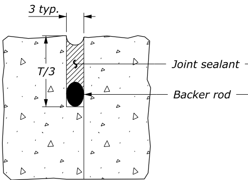
CONSTRUCTION JOINT
