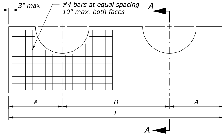
DOUBLE PIPE CULVERT HEADWALLS
