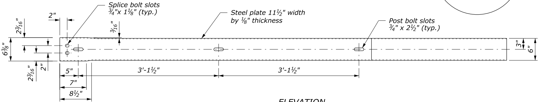
BENT PLATE RUBRAIL
