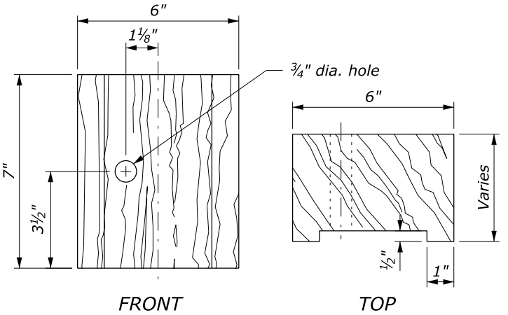
WOOD BLOCKOUT FOR RUBRAIL ON STEEL POSTS
