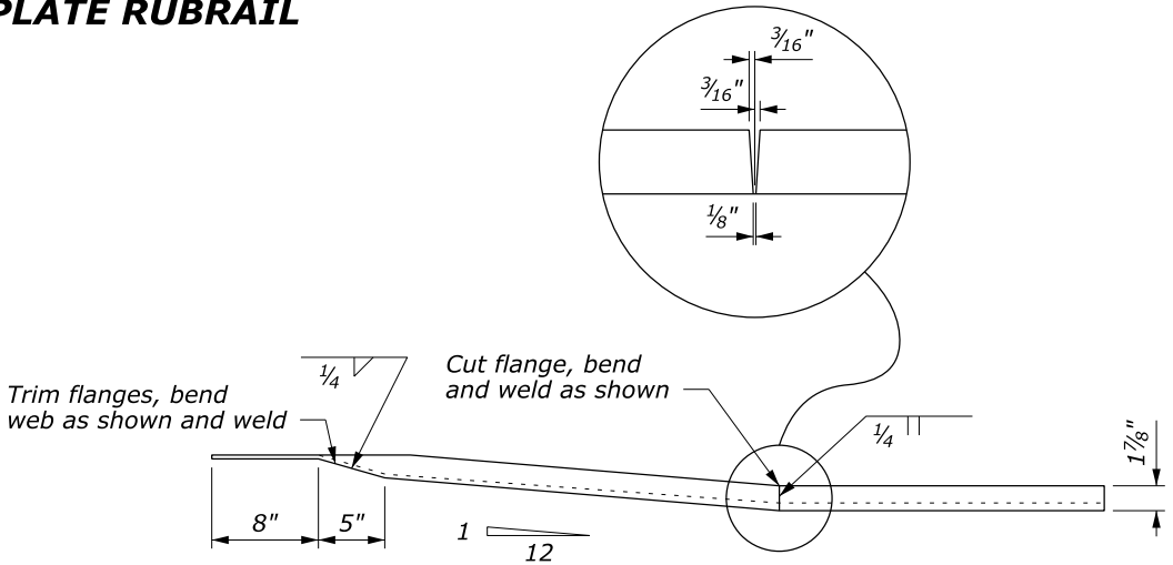
BENT PLATE RUBRAIL
