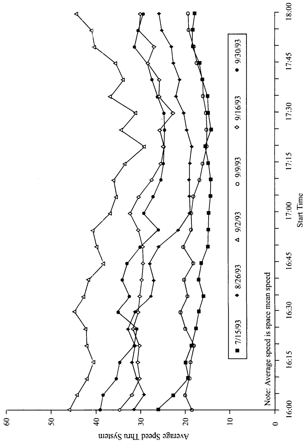
Figure 6. Example of Facility Speeds for Different Days and Departure Times for I-4 in Orlando, Florida.
