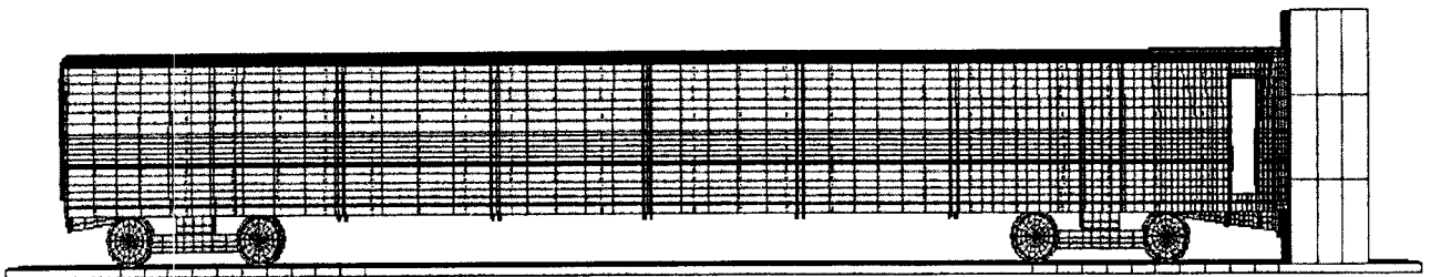
Figure 10. Finite-Element Model
