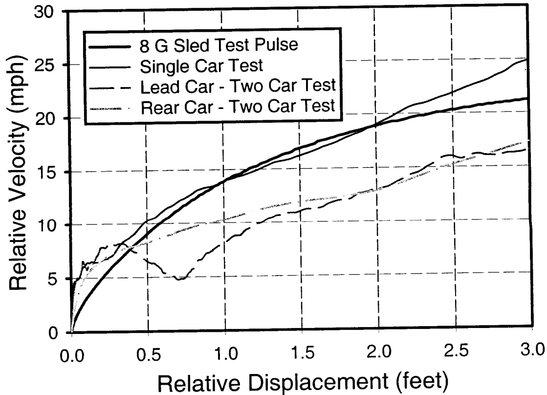
Figure 26. Relative Longitudinal Velocity of an Unrestrained Occupant as a Function of Relative Longitudinal Displacement
