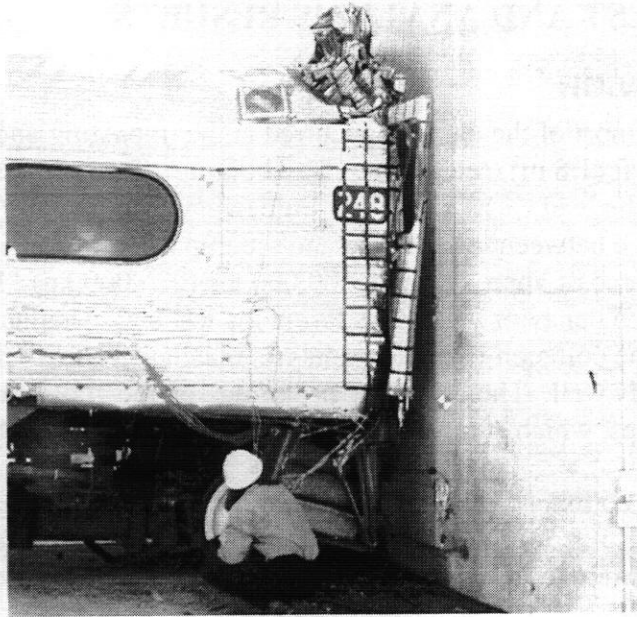
Figure 17. Photo of Impact End of Leading Car After Two-Car Impact Test
