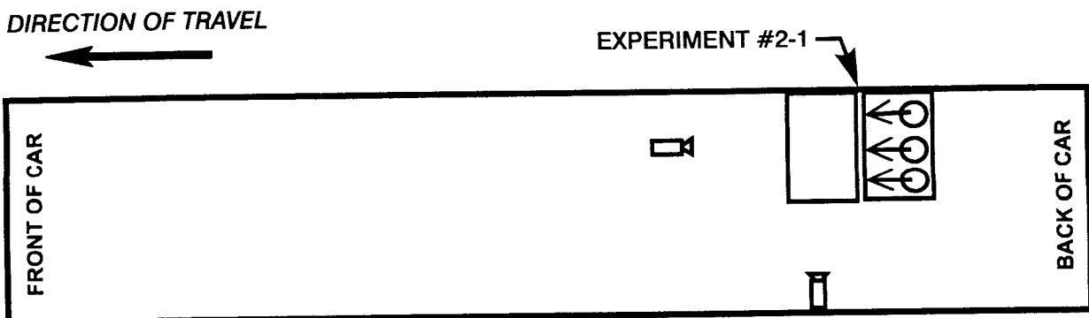
Figure 8b. Location of Interior Test Configurations in Trailing Car
