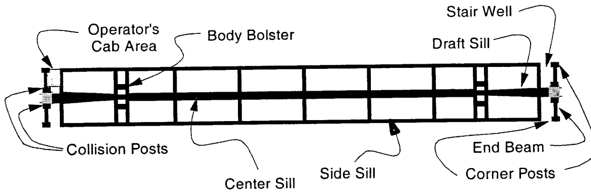
Figure A-1. Schematic of Typical Cab-car Structural Members, Top View
