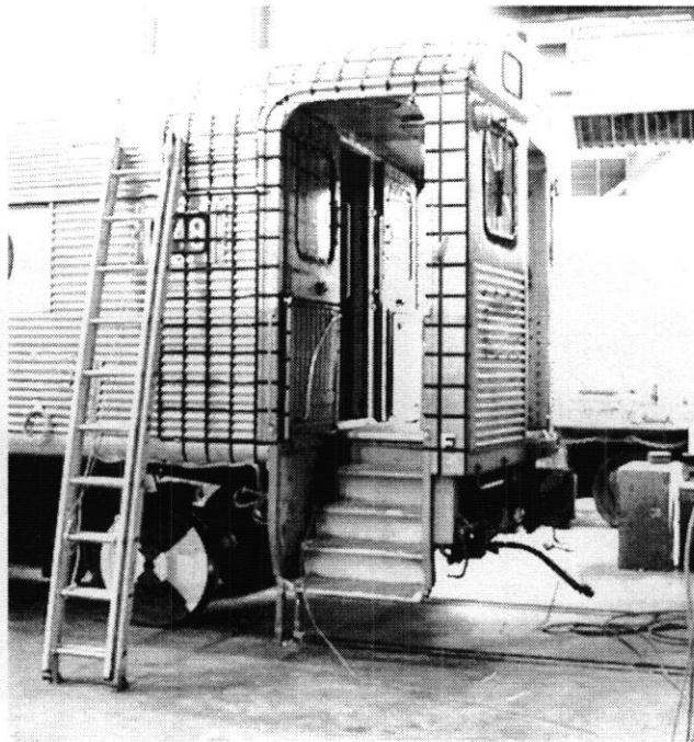
Figure 16. Photo of Impact End of Leading Car Prior to Two-Car Impact Test
