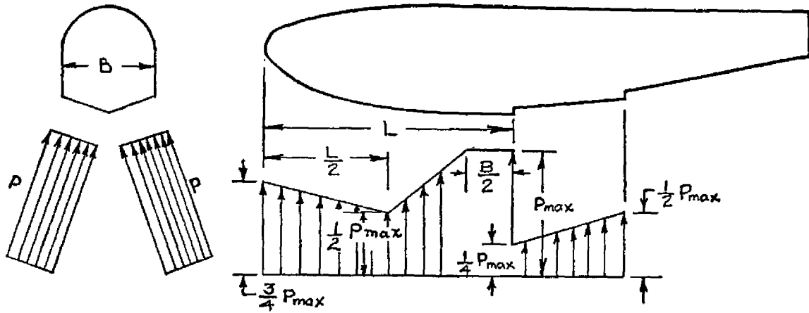
FIG. 04-11 DISTRIBUTION OF LOCAL PRESSURES - BOAT SEAPLANES
