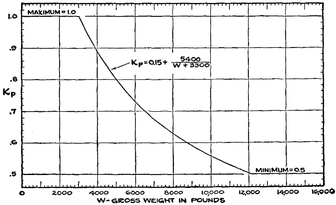
FIG. 04-2 PULL-UP SPEED FACTOR
