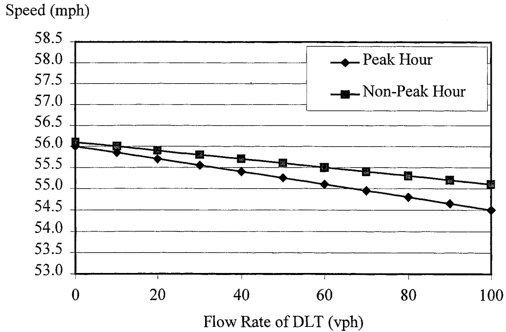
Figure 3.24 Speed Reduction of Through-Traffic Due to DLT at Site 7
