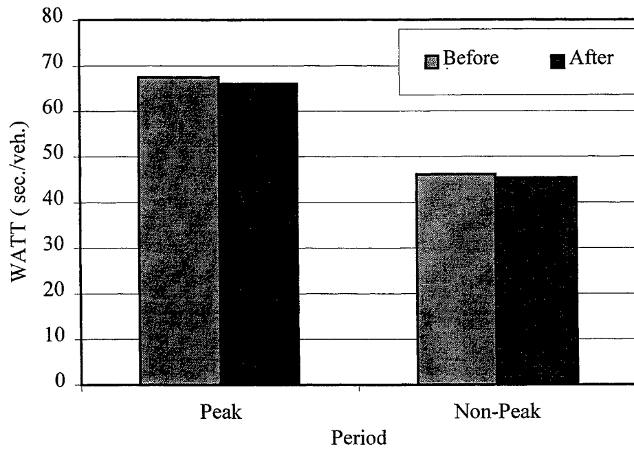
Figure 4.5 Before and After Comparison of WATT
