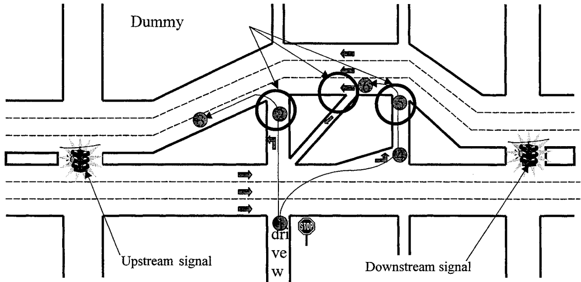
Figure 2.14 Graphic Description of Simulation Model for DLT & RTUT
