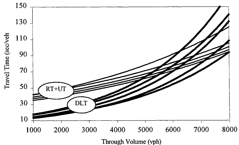
Figure 5.2 Comparison of Total Travels Time Between RTUT and DLT using GST
