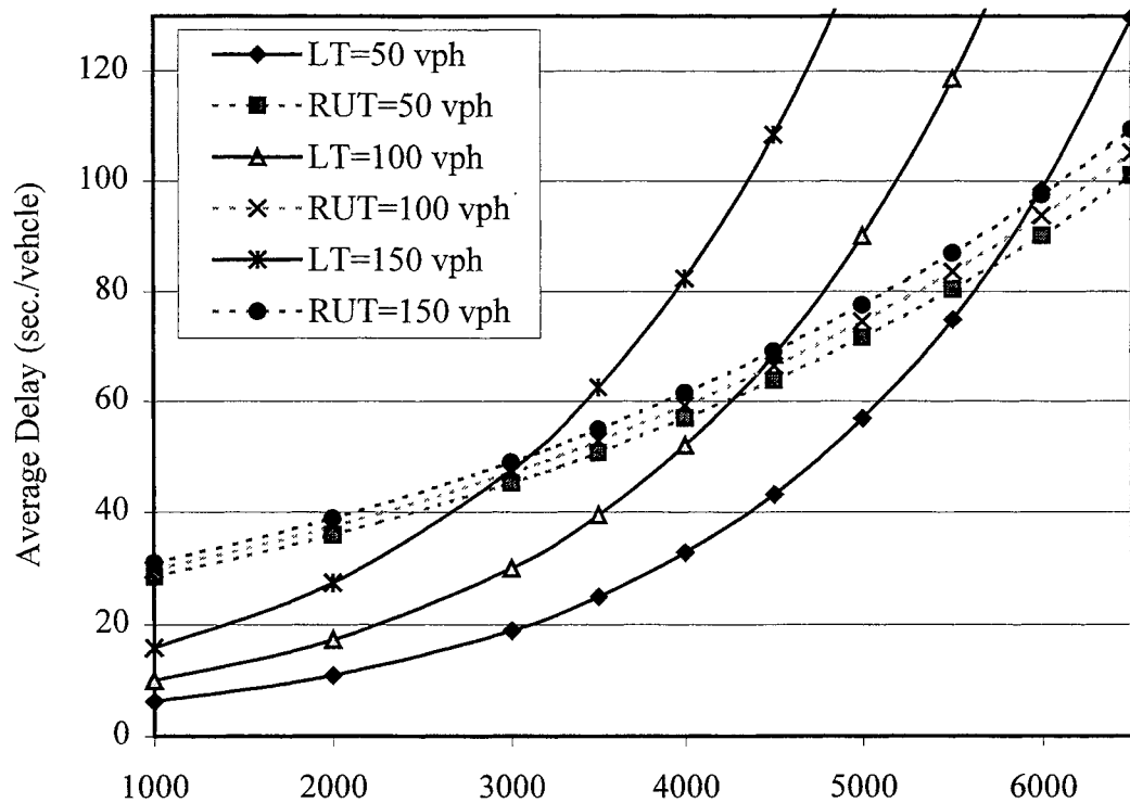
Flow Rate of Through-Traffic (vph) (LTIN=100 vph, Split=0.5, Weaving Distance=600 ft., Speed=50 mph)
