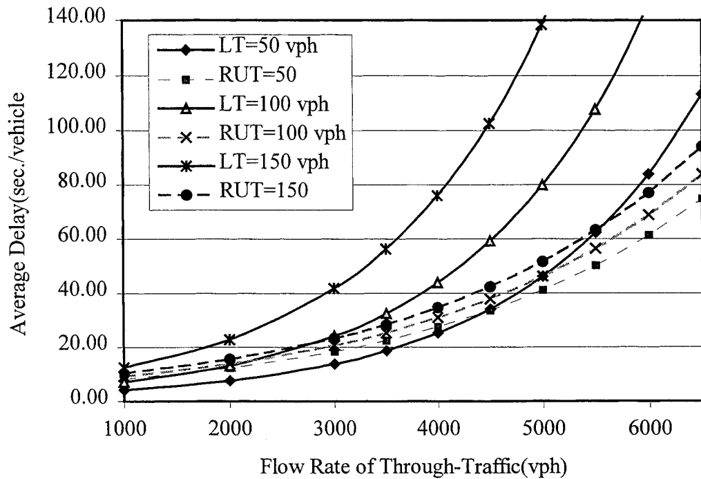
Figure 3.5 Comparison of Average Delay of Two Movements
