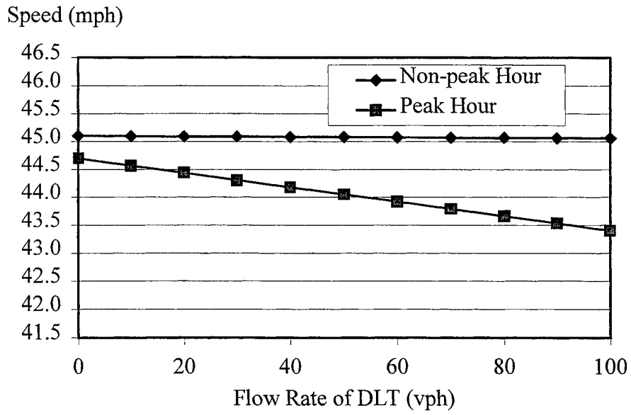
Figure 3.20 Speed Reduction of Through-Traffic Due to DLT at Site 2
