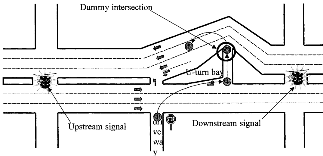
Figure 2.11 Graphic Description of U-Turn Model
