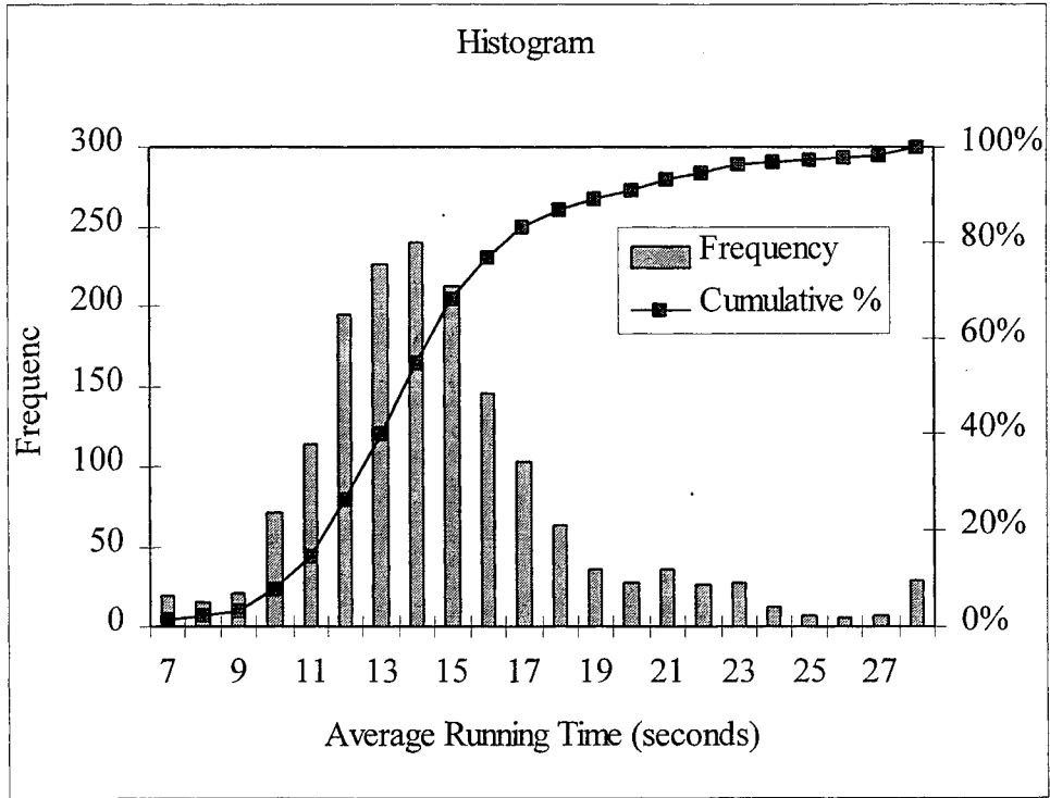
Figure 3.8 Average Running Time in the Weaving Section (420 ft.) of Site 3
