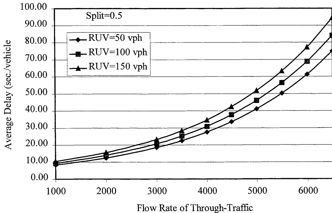
Figure 3.4 Curves for Average Total Delay of RTUT (Split=0.5)
