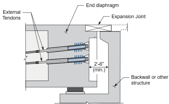
a) Tendons installed
