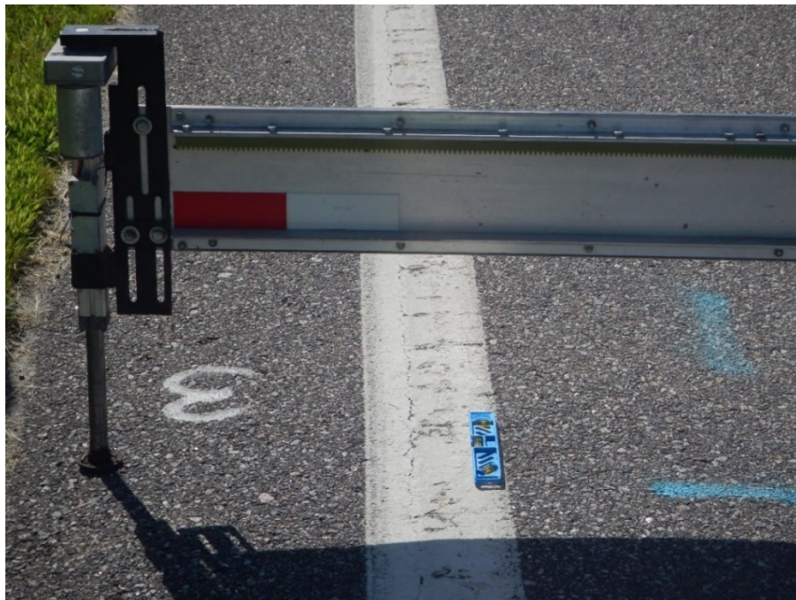
Figure 3. Picture. Example transverse profile used in rut depth validation.
