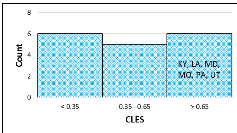
Figure 64. Chart. CLES results for IS2 and HPMS cracking condition metric.
