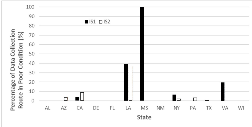
Figure 51. Chart. Comparison of IS1 and IS2 Poor faulting condition ratings at route level.
