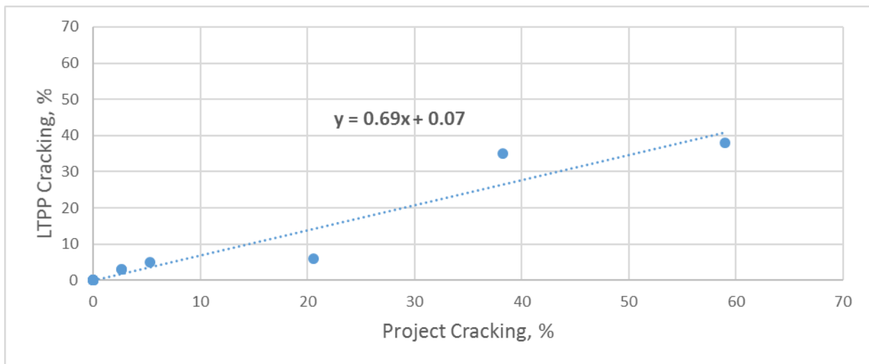
Figure 74. Plot. Project versus LTPP IRI measurements on asphalt pavement test sections.
