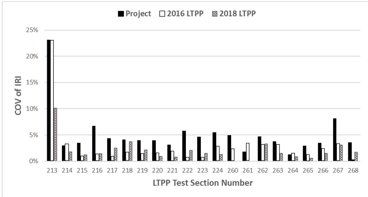
Figure 67. Plot. IRI COV for LTPP test sections.
