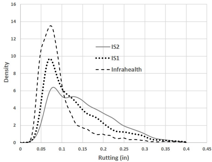
Figure 79. Plot. Density plots of IRI condition metric for IS1, IS2, and InfraHealth datasets.
