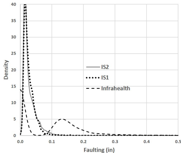
Figure 81. Plot. Density plots of cracking condition metric for IS1, IS2, and InfraHealth datasets.
