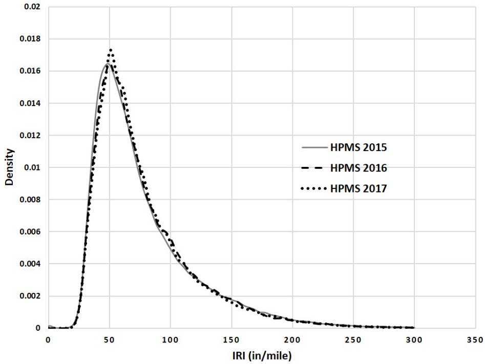
Figure 52. Plot. Density plots of IRI condition metric for 2015, 2016, and 2017 HPMS datasets.
