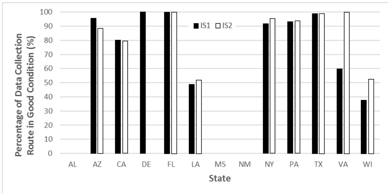
Figure 49. Chart. Comparison of IS1 and IS2 Poor cracking condition ratings at route level.
