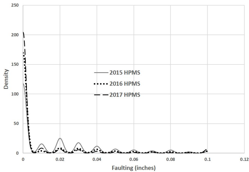
Figure 54. Plot. Density plots of cracking condition metric for 2015, 2016, and 2017 HPMS datasets.
