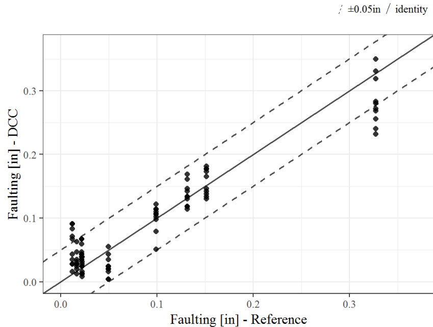
Figure 11. Plot. Faulting validation data.
