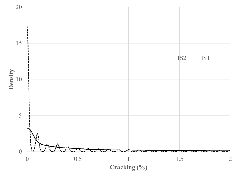
Figure 33. Plot. Density plots of rutting condition metric for IS1 and IS2 datasets.
