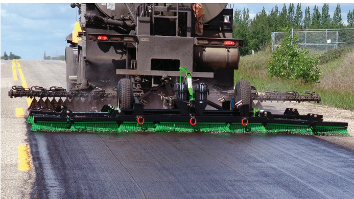
Saskatchewan Ministry of Highways and Infrastructure Figure 7. Scrub sealing
