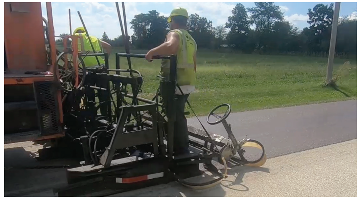
Strawser Construction Inc. Figure 8. Cape sealing
